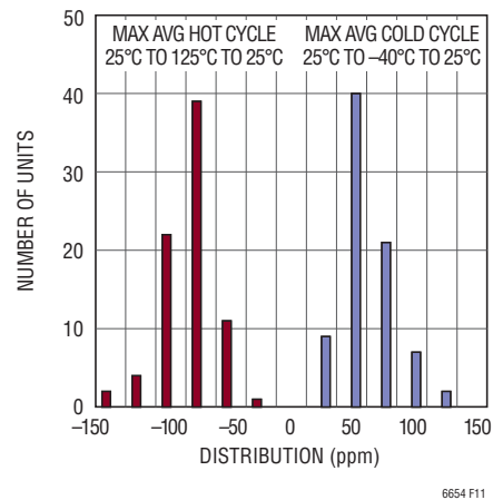
Figure 11. Thermal Hysteresis -40^{\circ}\text{C} to 125^{\circ}\text{C}
