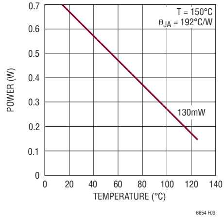
Figure 9. Maximum Allowed Power Dissipation of the LT6654
