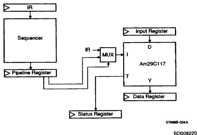
Figure 13. System Block Diagram
