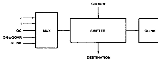
Figure 3. Shift-Down Function
