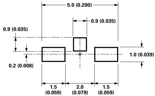
Figure 10. Recommended Soldering Pattern for HSMB-C110.
