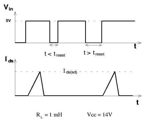
Figure 17 Definition of t_{reset}
