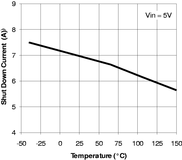
Figure 6 Over-Current Shutdown Threshold vs. Temperature
