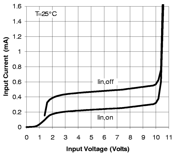
Figure 7 Input Current vs. Input Voltage
