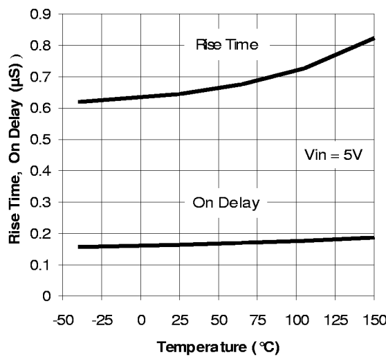
Figure 10 Turn-On Characteristics vs. Temperature
