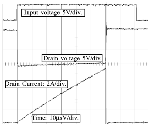
Figure A4. Waveforms at over-current shut-down
