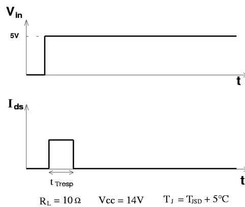
Figure 18 Definition of t_{Tresp}
