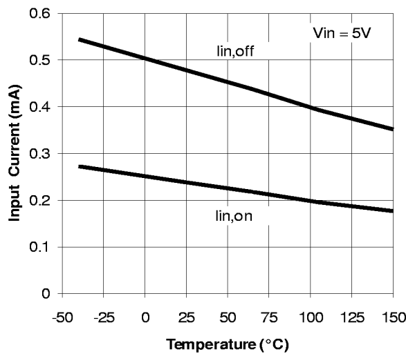
Figure 8 Input Current vs. Temperature
