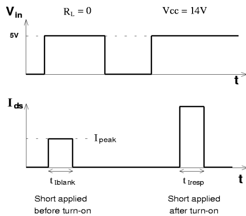
Figure 16 Definition of I_{peak} , t_{blank} , t_{iresp}
