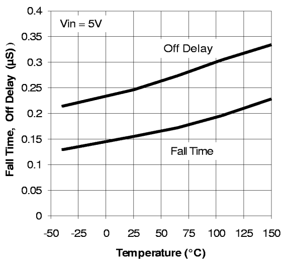
Figure 12 Turn-Off Characteristics vs. Temperature
