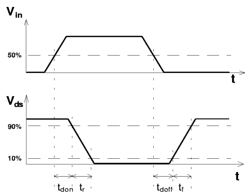
Figure 15 Definition of Switching Times
