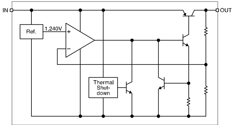
MIC37139 Fixed Regulator Block Diagram
