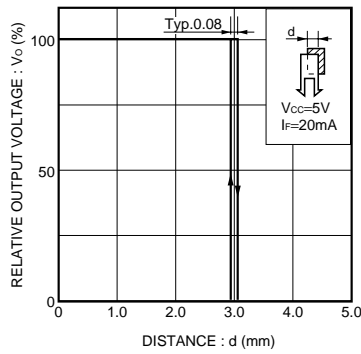
Fig.8 Relative output voltage vs. distance
