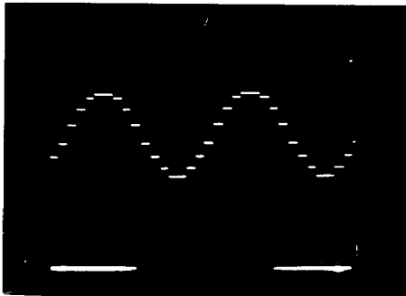
Figure 2. Transmit Carrier Sine Wave
