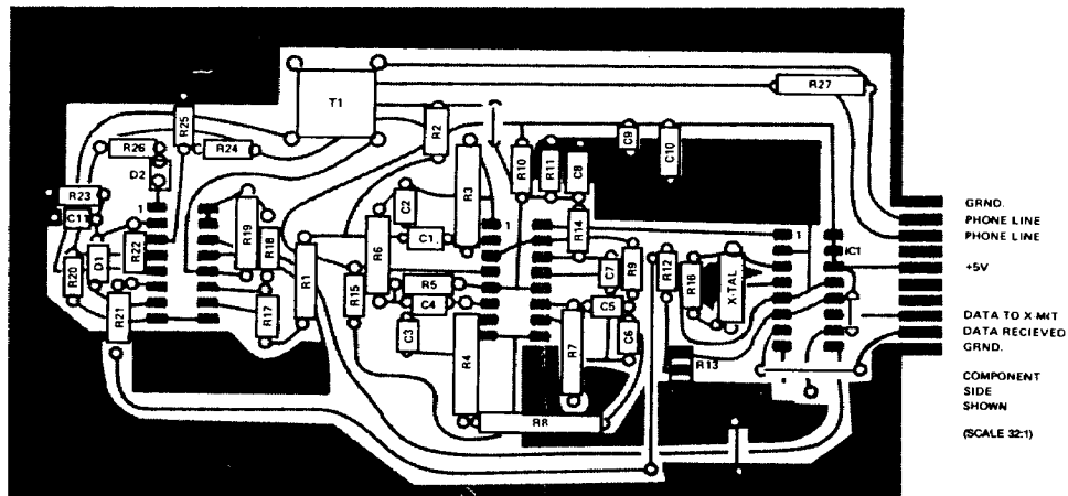
Figure 6. Complete FSK Modem Printed Circuit Board Layout (Circuit Shown in Figure 4)
