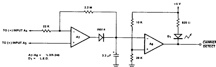
Figure 5. Carrier Detect Circuit
