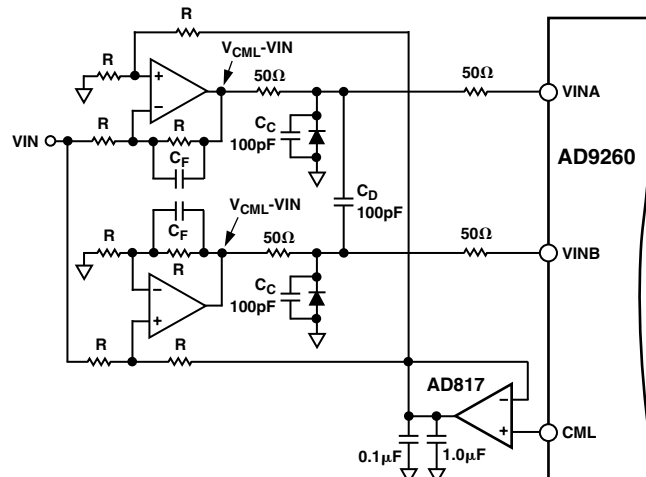
Figure 58. DC-Coupled Differential Driver with Level-Shifting
