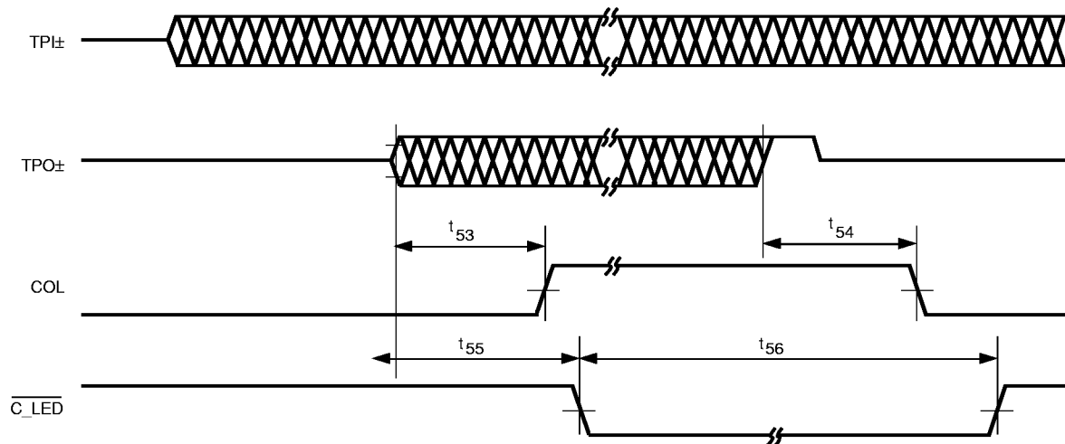
Figure 25. Collision Timing, Transmit
