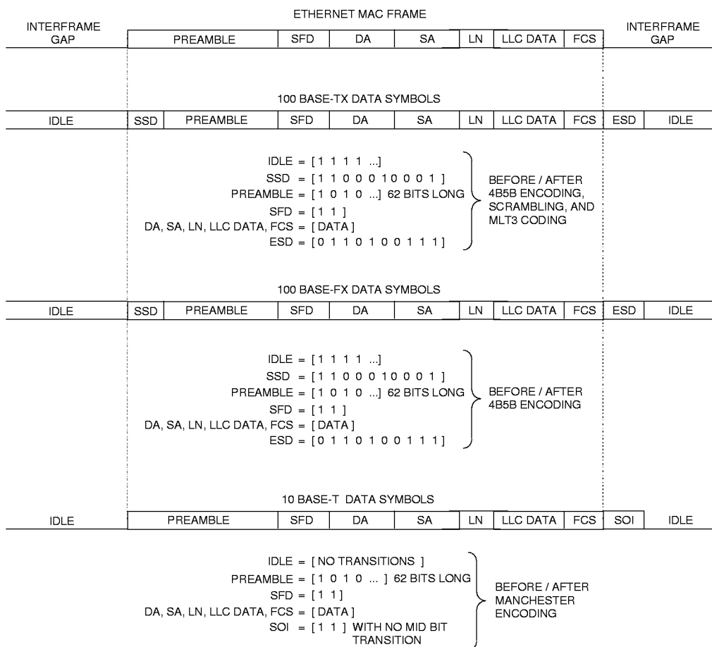
Figure 2. TX/10BT Frame Format
