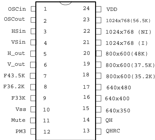
WT8045N24P6
