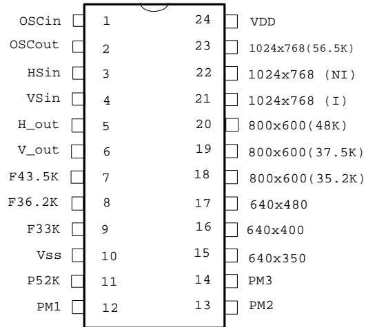
WT8045N24P7
