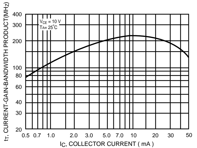
Figure 6. Current-Gain-Bandwidth Product
