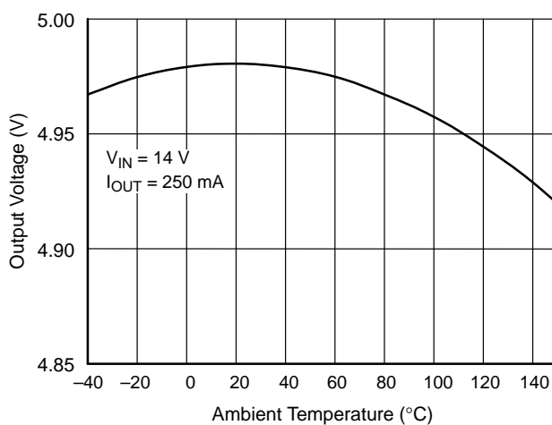
Figure 3. Regulator 2 Output Voltage
