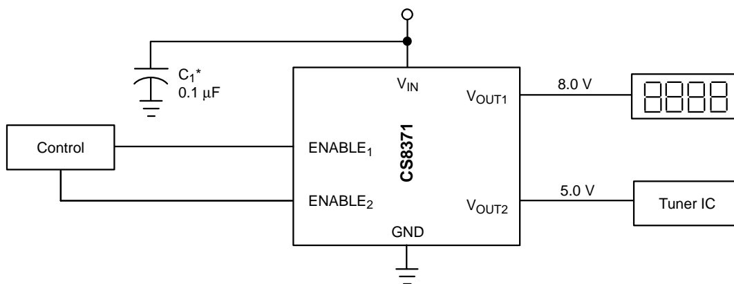
Figure 23. Applications Circuit
