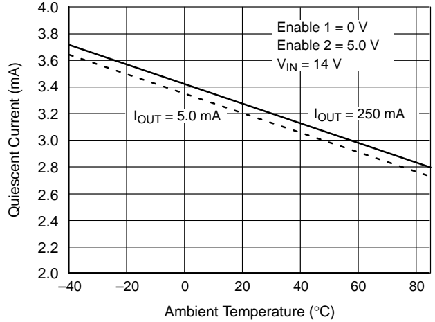
Figure 11. Regulator 2 Quiescent Current
