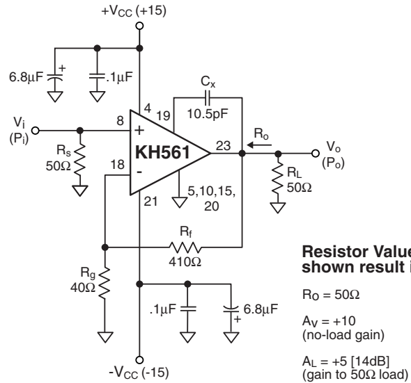
Figure 1: Test Circuit
