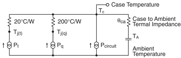
www.datasheet4u.com Figure 10: Thermal Model
