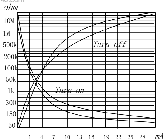
Input mA/ohm curve
