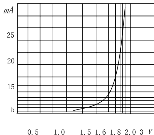
Input v/mA curve
