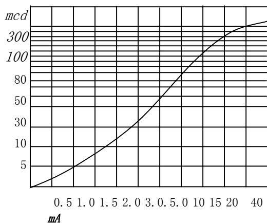
Input mA / mcd curve
