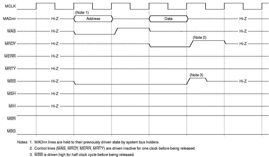
Figure 3. MBus Single Read
