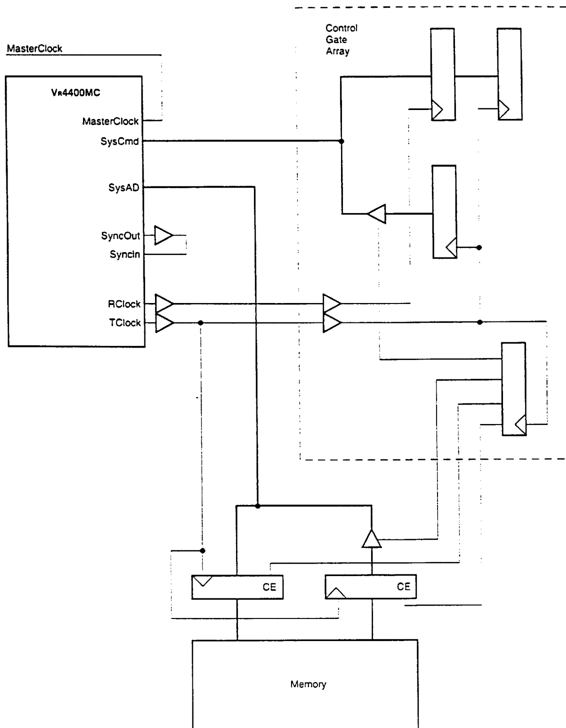
Fig. 11-6 System Without Phase Lock Employing the Vn4400MC Processor (b)
