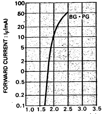
FORWARD VOLTAGE : V_F (V) FORWARD CURRENT vs. FORWARD VOLTAGE
