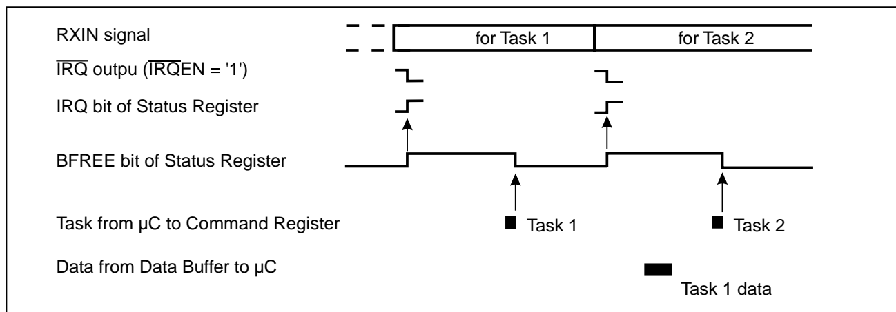
Figure 8: The Receive Process
