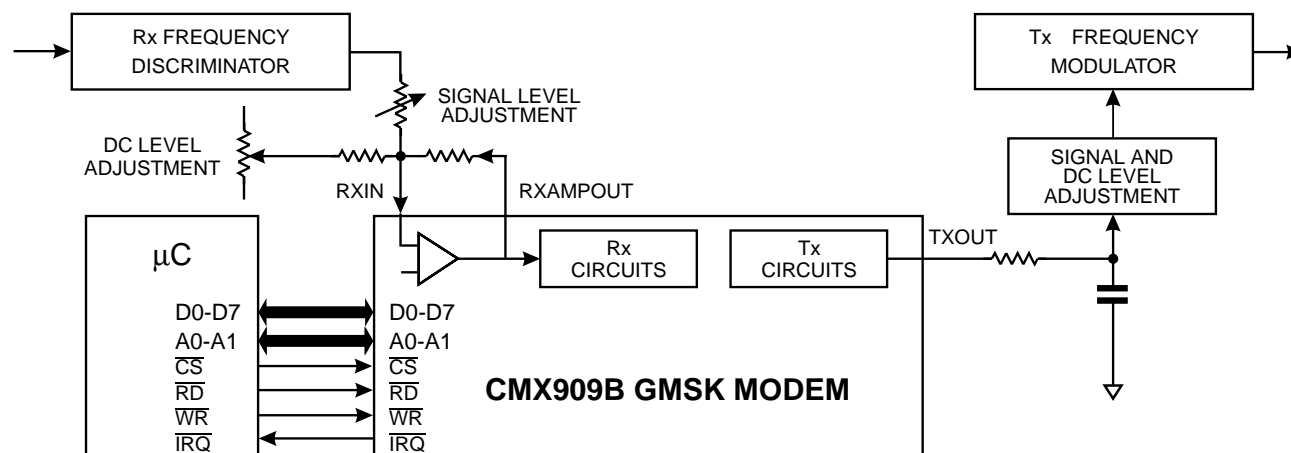
Figure 19: Typical System Installation
