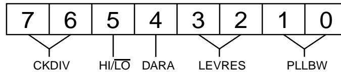
Control Register
