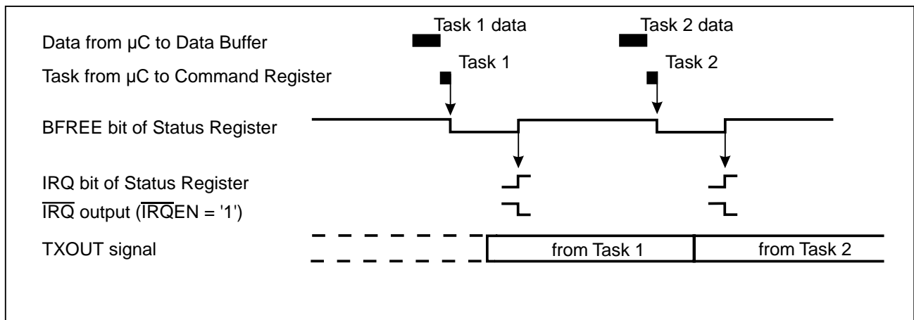
Figure 7: The Transmit Process
