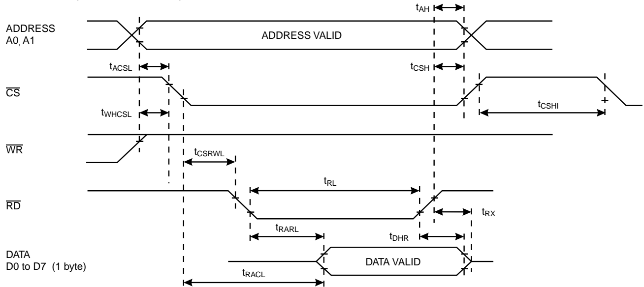
Figure 20: \mu C Parallel Interface Timings
