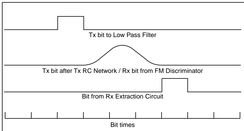
Figure 11: Low Pass Filter Delay
