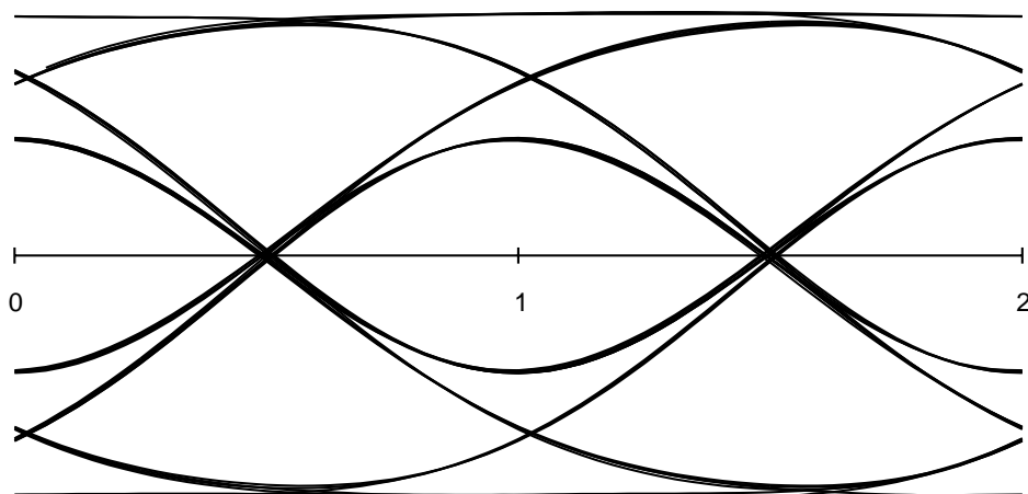
Figure 5: Transmitted Signal Eye Diagram (after the external RC Filter)
