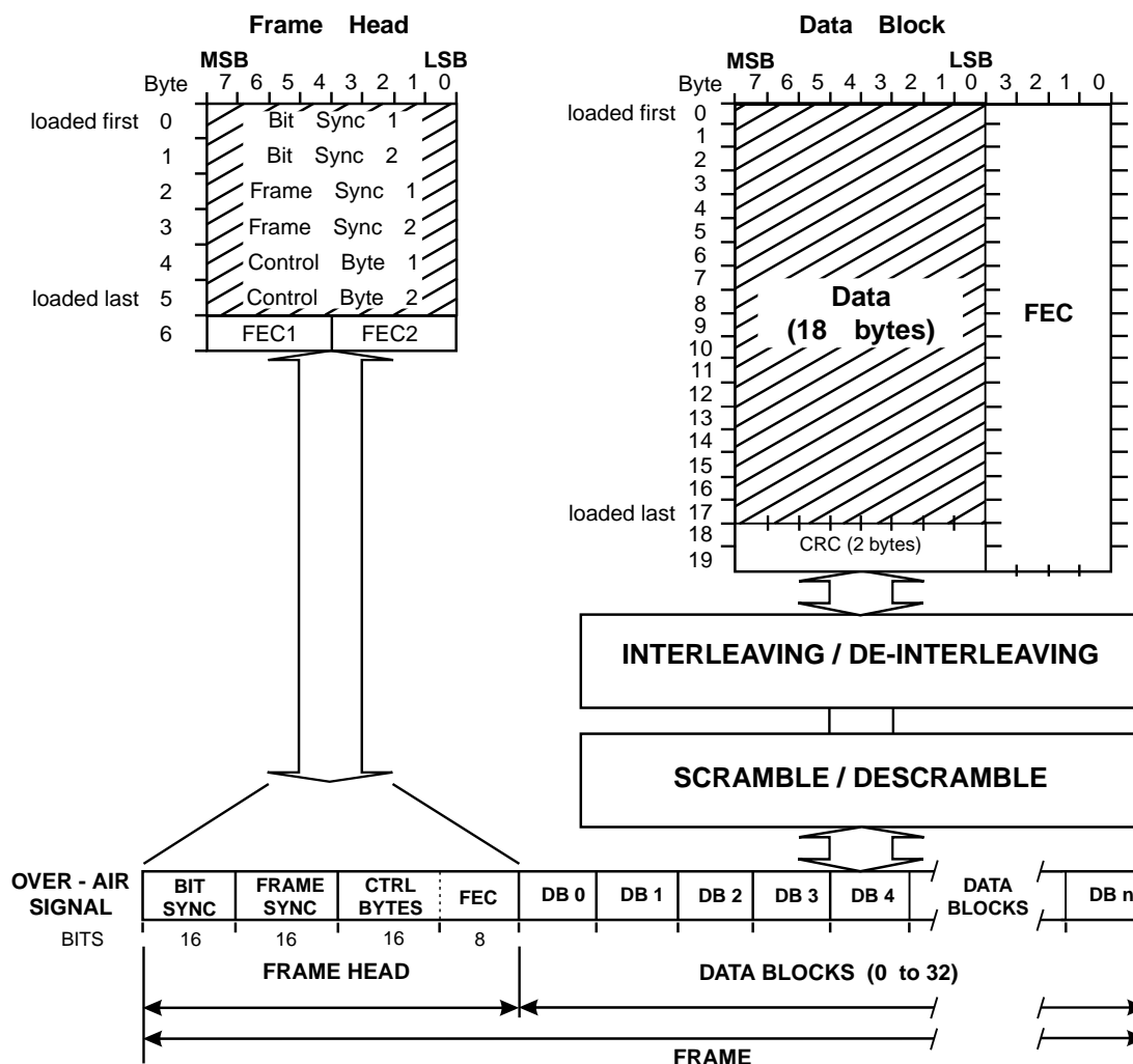
Figure 6: Mobitex Over Air Signal Format
