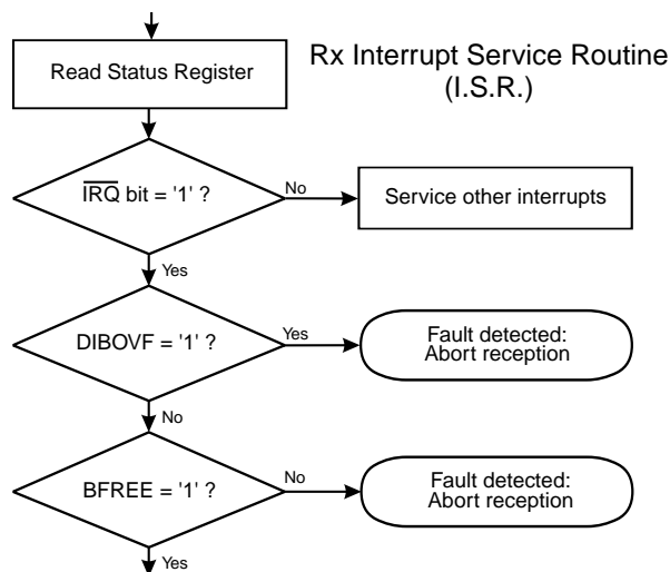
Figure 15: Receive Process
