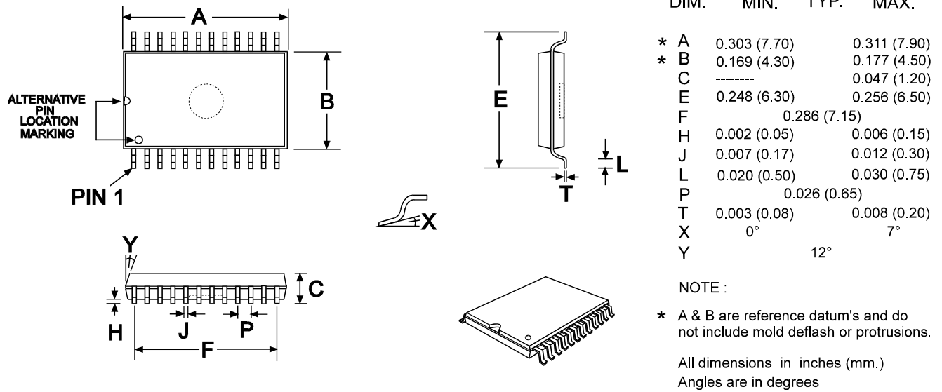
Figure 22: 24-pin TSSOP (E2) Mechanical Outline: Order as part no. CMX909BE2
