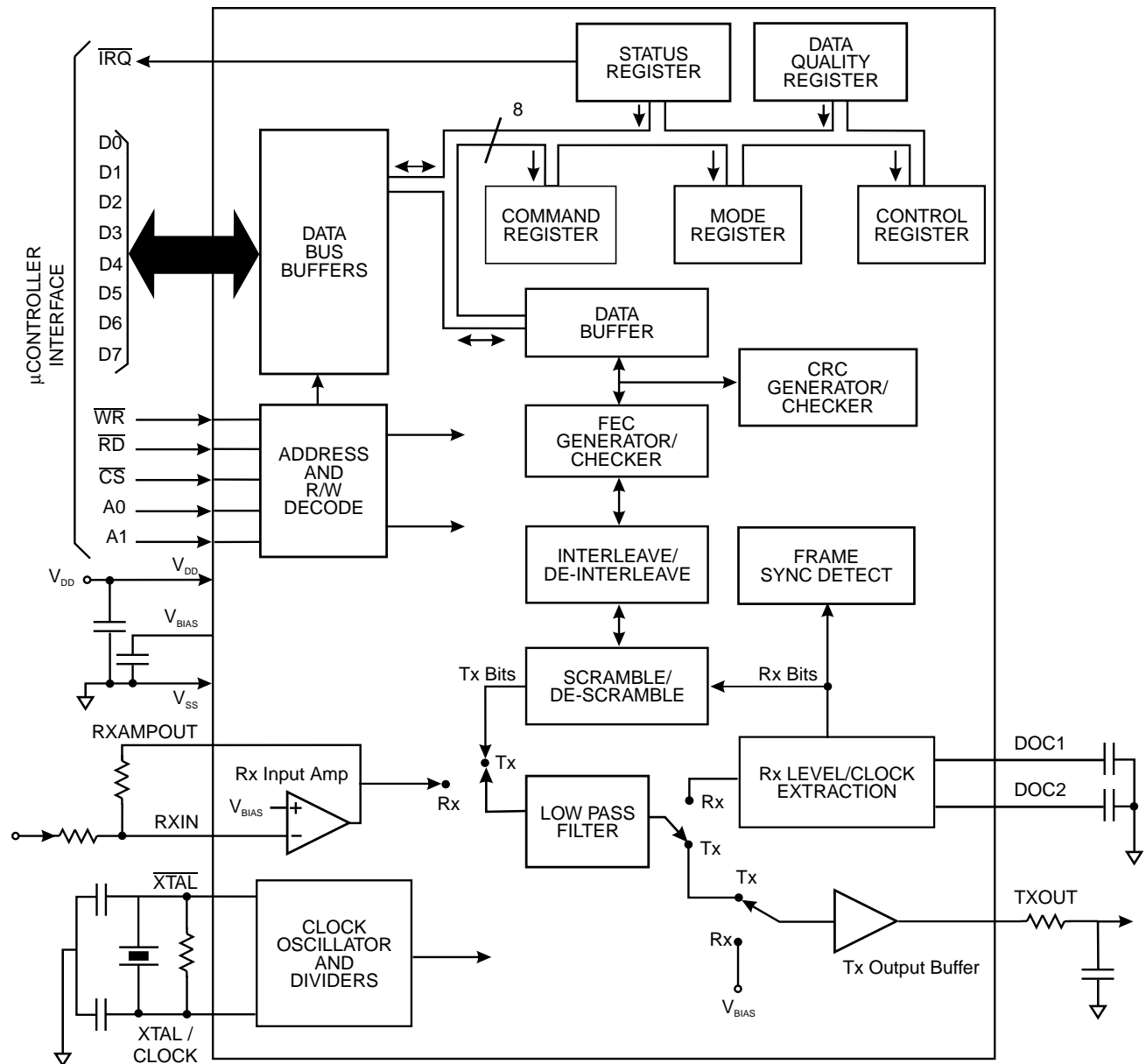
Figure 1: Block Diagram
