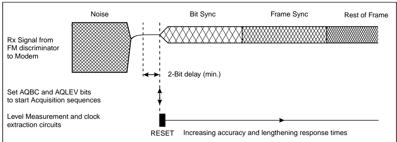
Figure 16: Bit Clock and Level Acquisition Example
