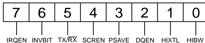
Mode Register
