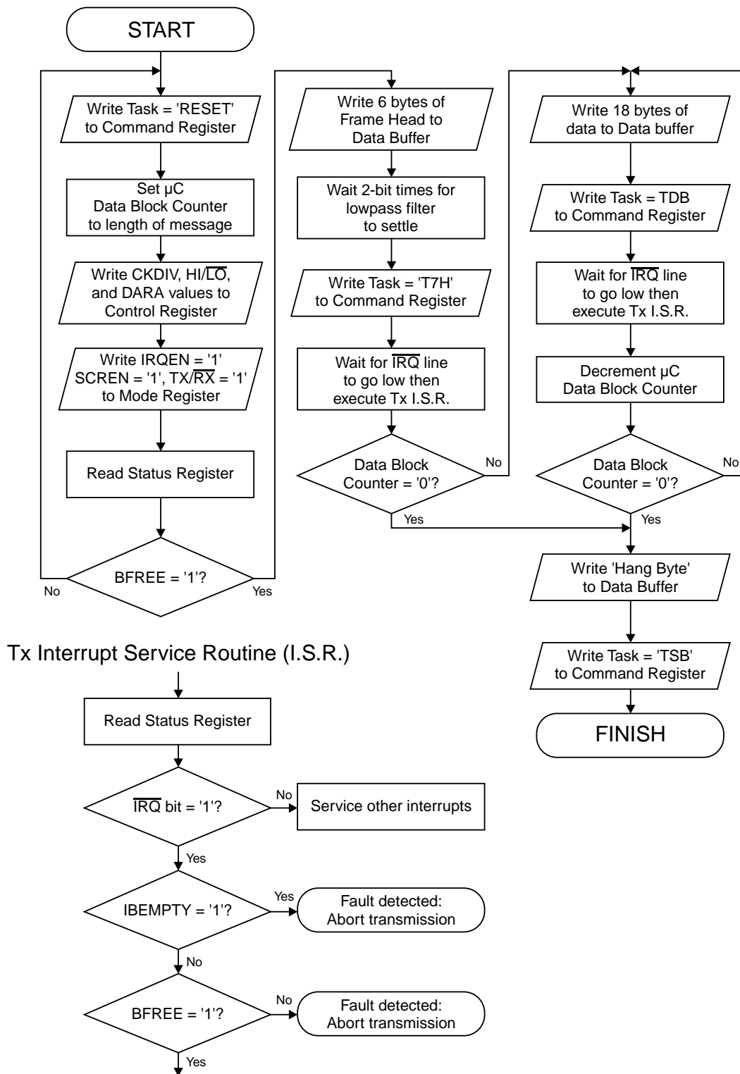
Figure 14: Transmit Process
