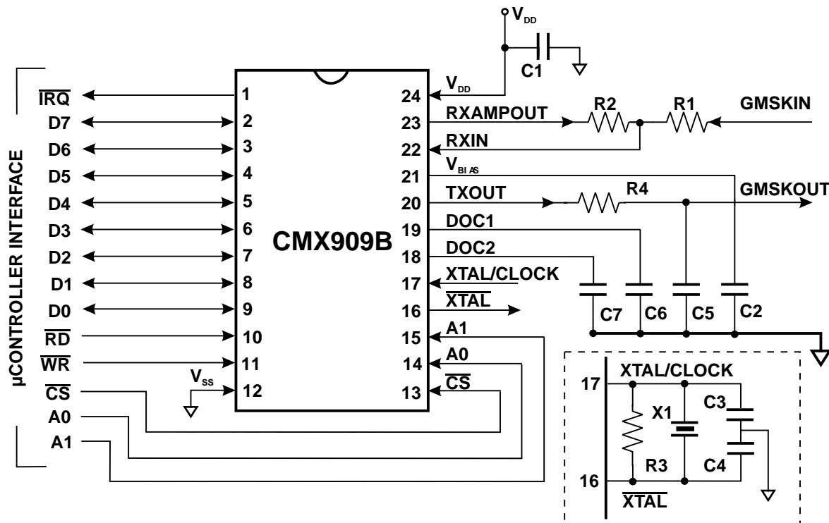
Figure 2: Recommended External Components
