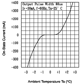
Fig.7 On-State Characteristics
