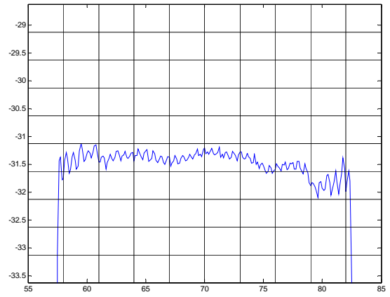
Phase Linearity(f0±12MHz)
