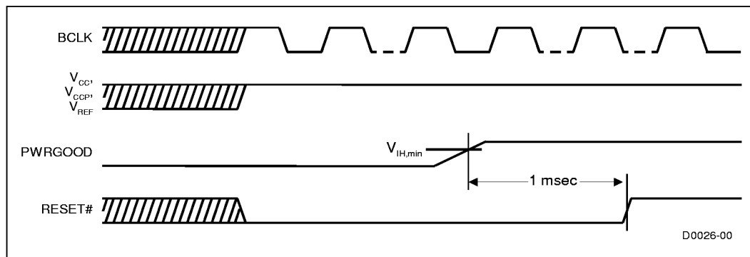
Figure 21. PWRGOOD Relationship at Power-On
