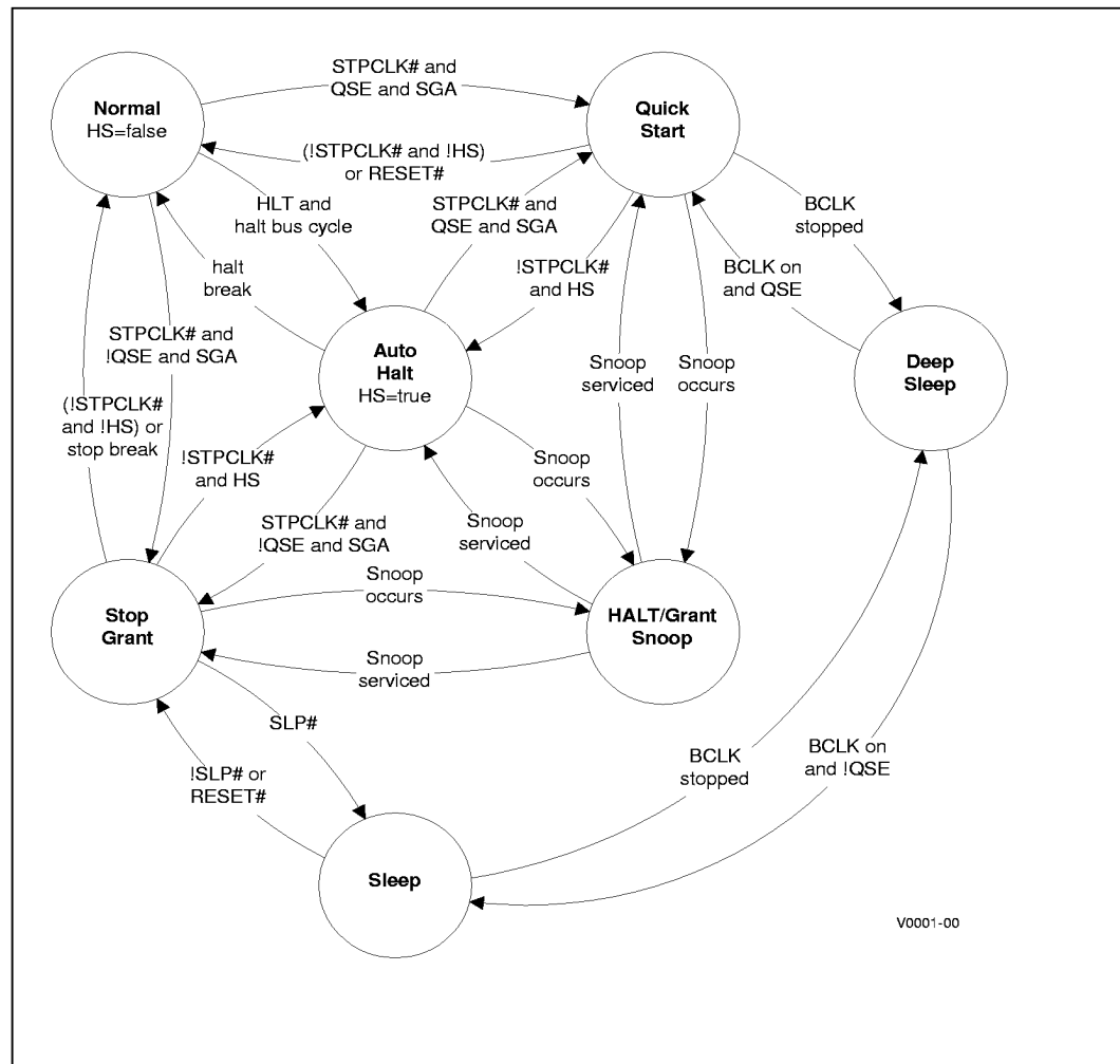
Figure 2. Clock Control States
