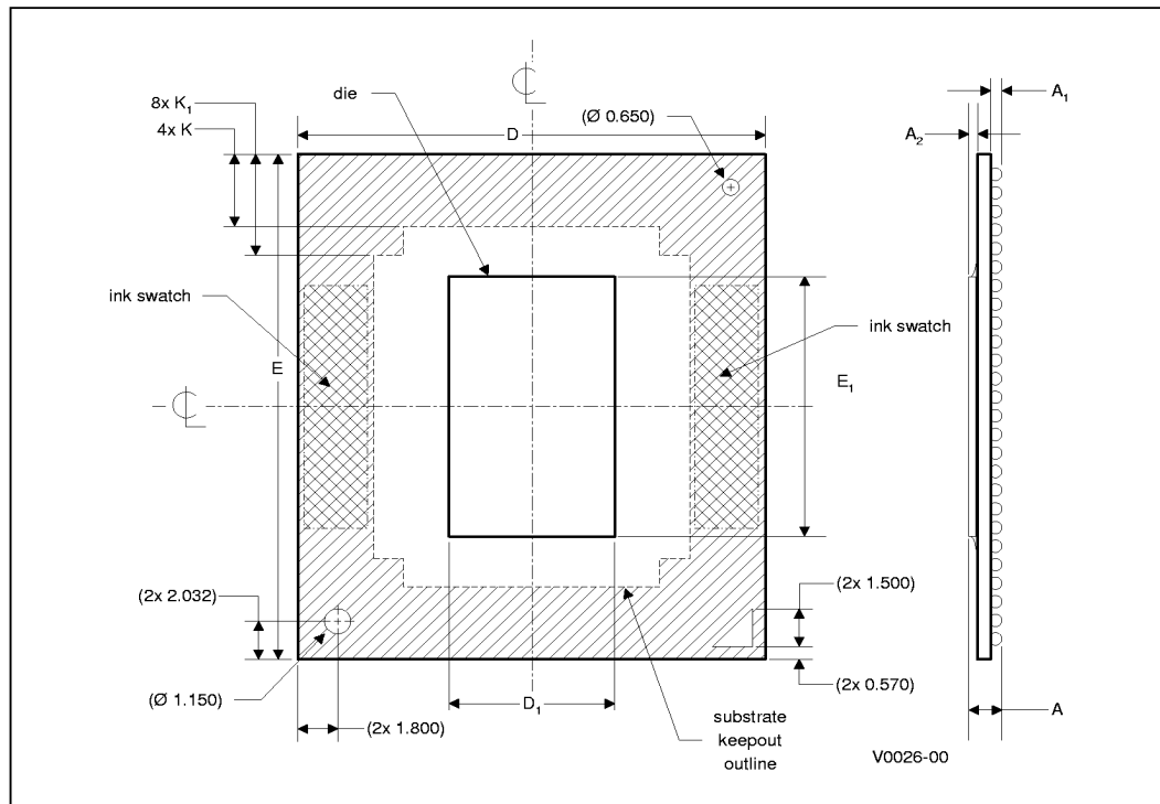
Figure 17. Surface-Mount BGA1 Package-Top and Side View
