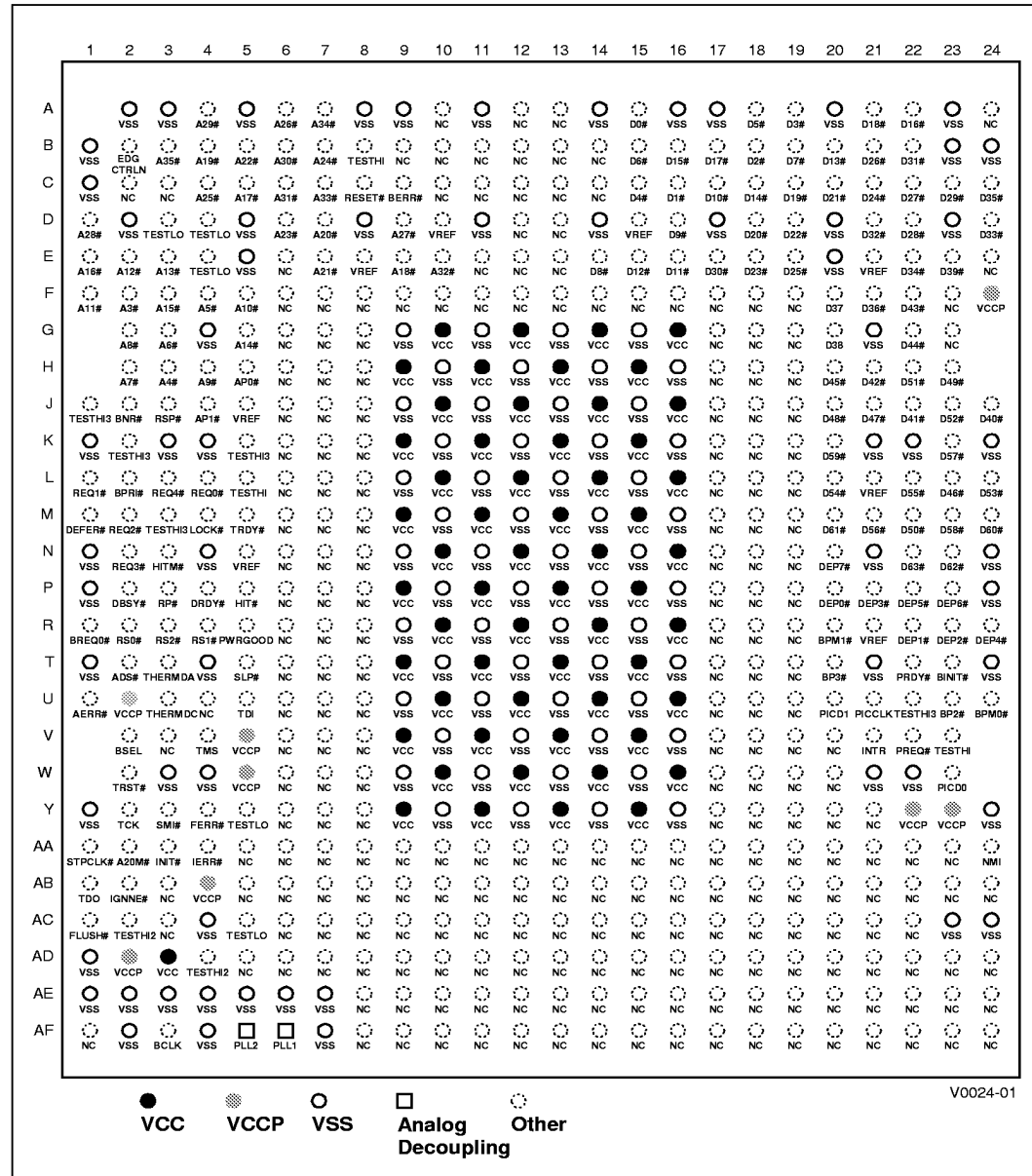
Figure 19. Ball Map - Top View
