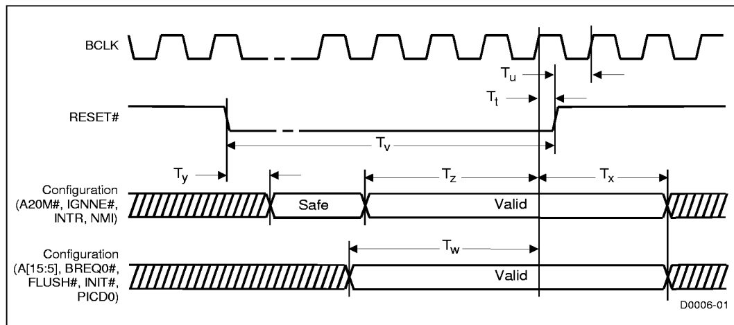
Figure 8. Cold/Warm Reset and Configuration Timings
