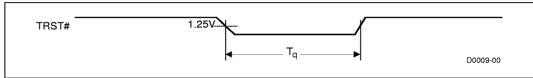
Figure 11. Test Reset Timings
