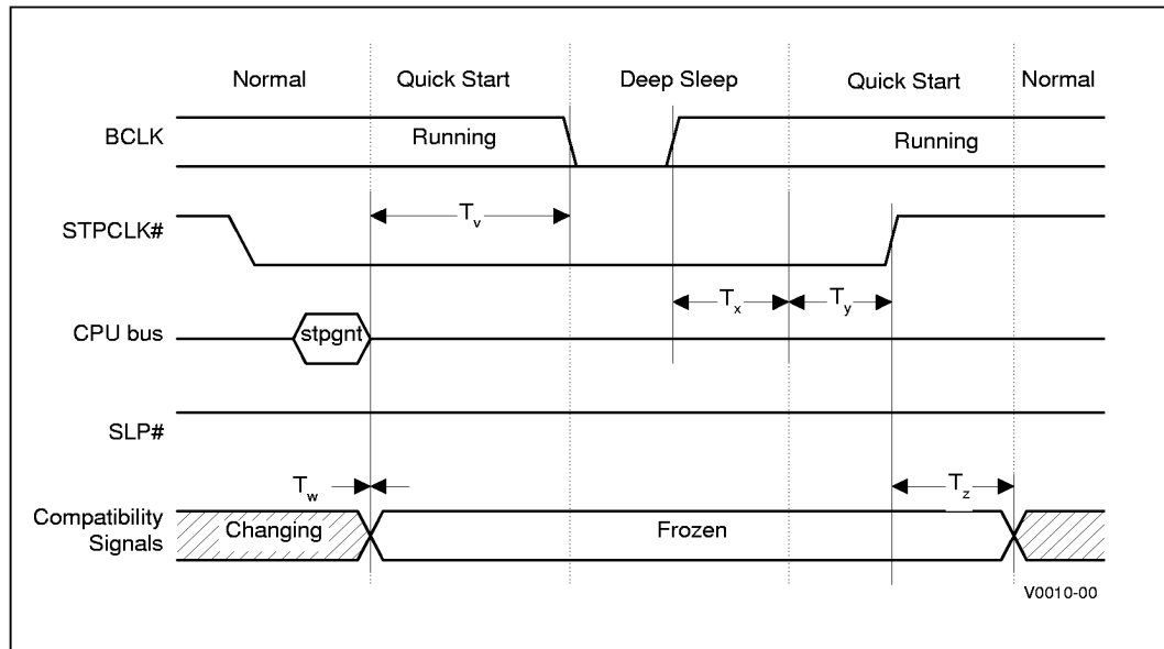
Figure 12. Quick Start/Deep Sleep Timing
