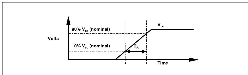
Figure 3. Ramp Rate Requirement
