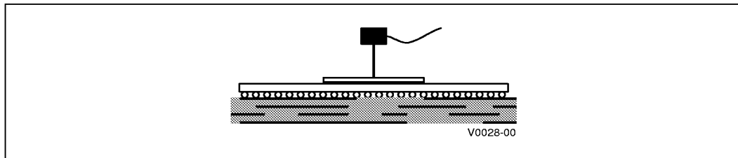
Figure 20. Technique for Measuring Case Temperature
