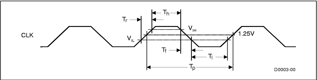
Figure 5. Generic Clock Waveform
