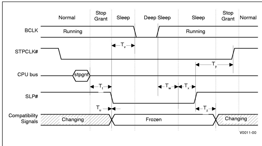
Figure 13. Stop Grant/Sleep/Deep Sleep Timing
