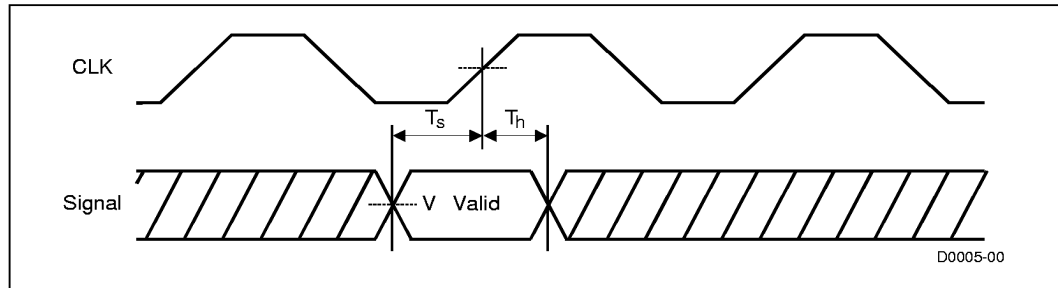
Figure 7. Setup and Hold Timings
