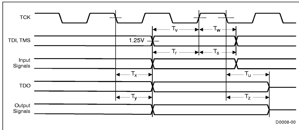
Figure 10. Test Timings (Boundary Scan)
