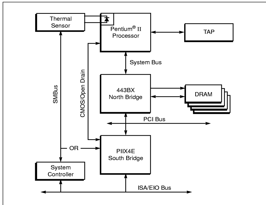
Figure 1. Components of a Pentium® II Processor - Low Power-based System
