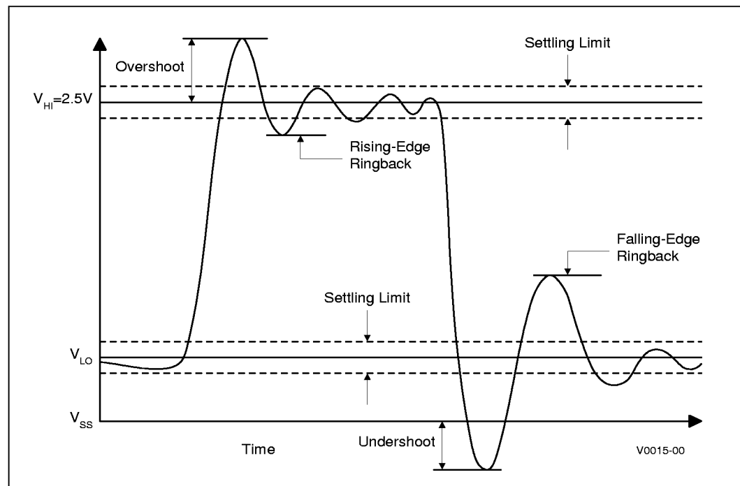
Figure 16. Non-GTL+ Overshoot/Undershoot and Ringback
