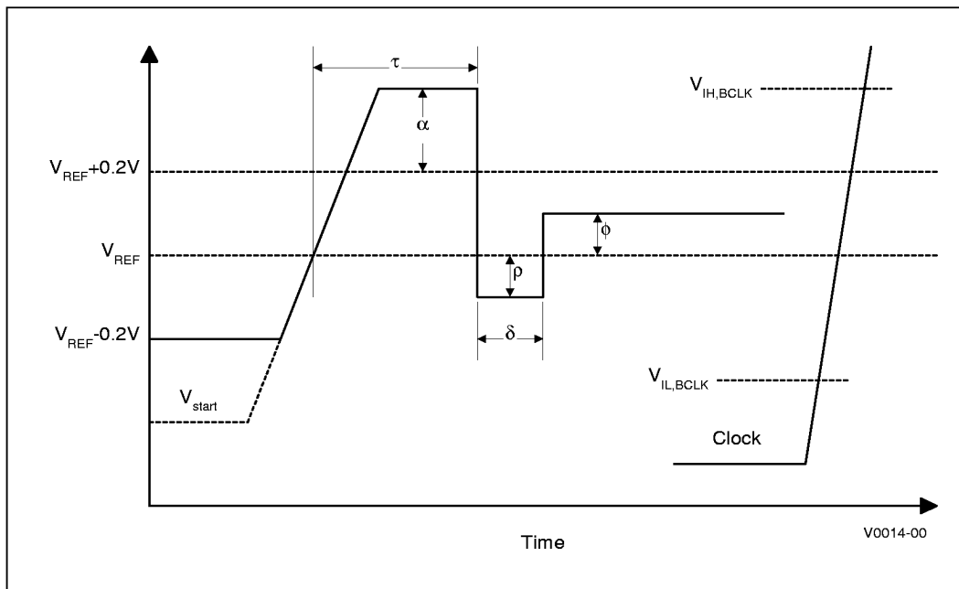
Figure 15. Low to High, Low Power GTL+ Receiver Ringback Tolerance
