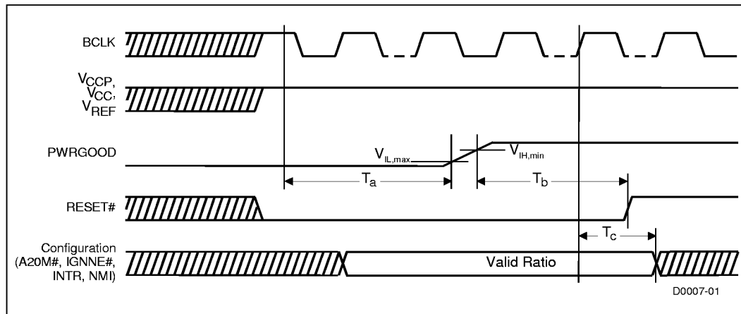
Figure 9. Power-On Reset Timings
