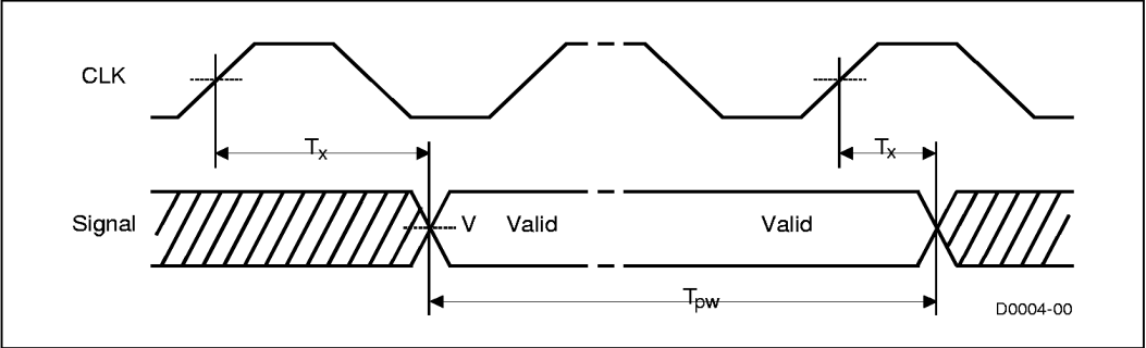
Figure 6. Valid Delay Timings
