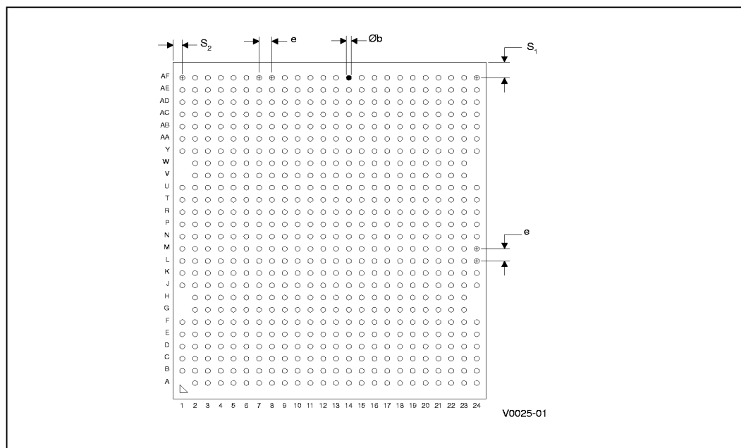
Figure 18. Surface-Mount BGA1 Package-Bottom View
