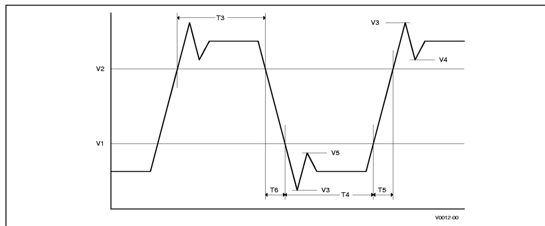
Figure 14. BCLK Generic Clock Waveform
