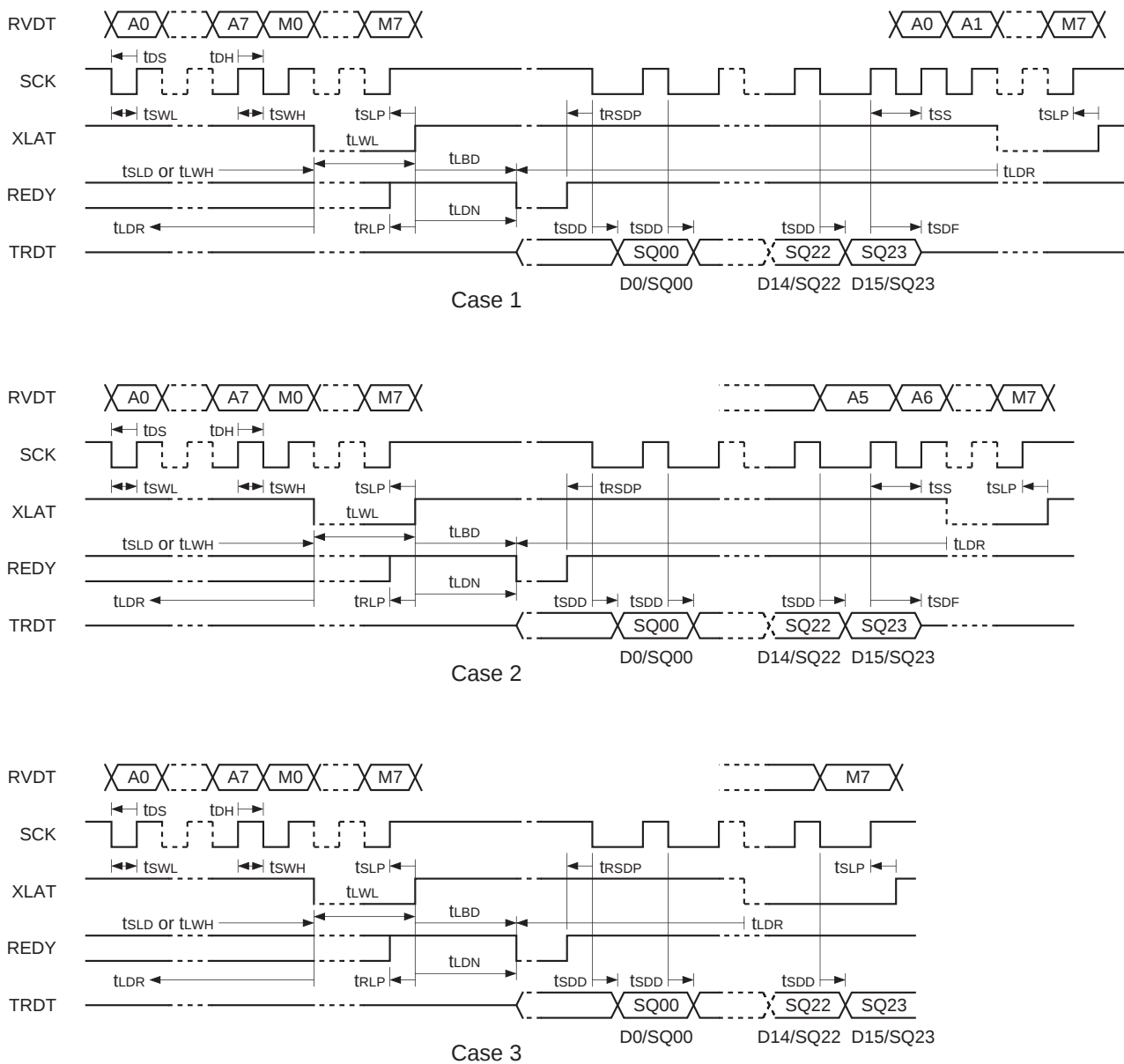
Figure 6-3. Read Timing
