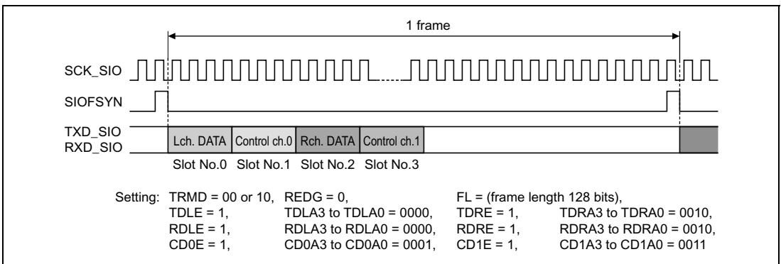
Figure 20.7 Control Data Interface (Slot Position)
