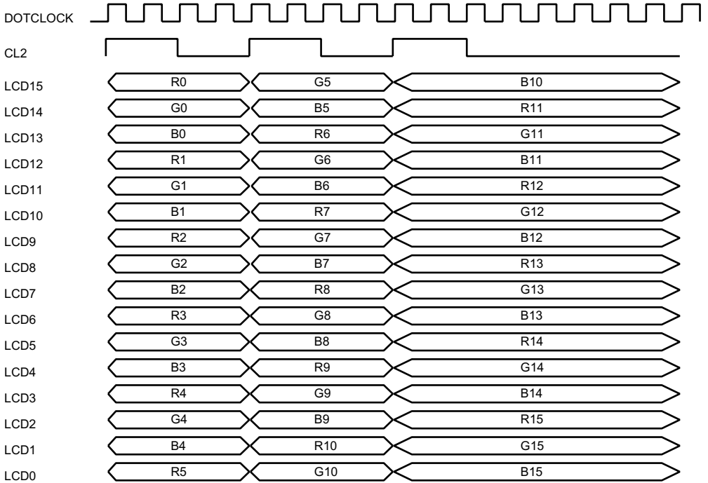
Figure 25.13 Clock and LCD Data Signal Example
