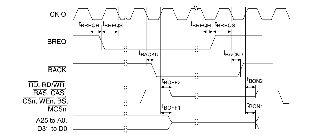
Figure 32.13 Bus Release Timing
