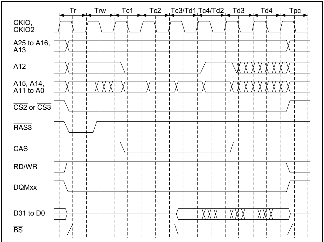
Figure 12.14 Synchronous DRAM Burst Read Wait Specification Timing
