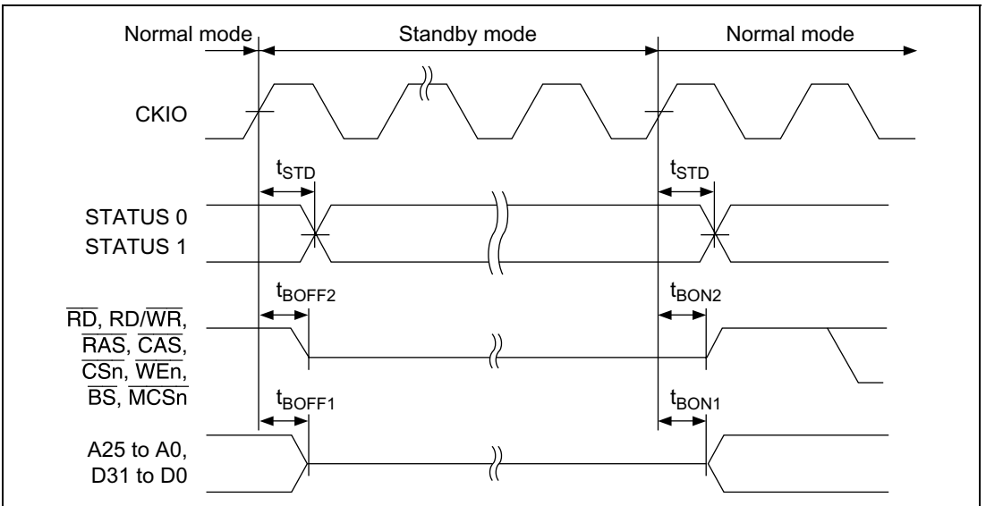
Figure 32.14 Pin Drive Timing at Standby
