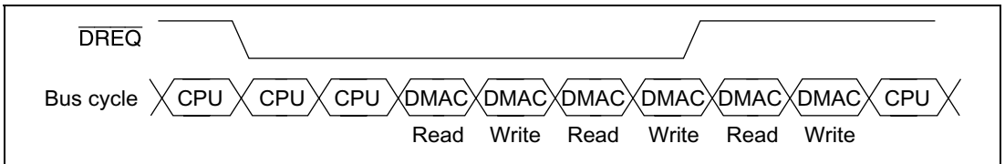
Figure 14.15 Example of Transfer in Burst Mode
