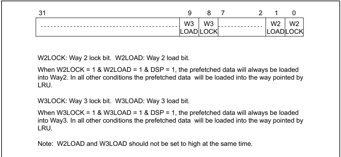
Figure 5.3 CCR2 Register Configuration
