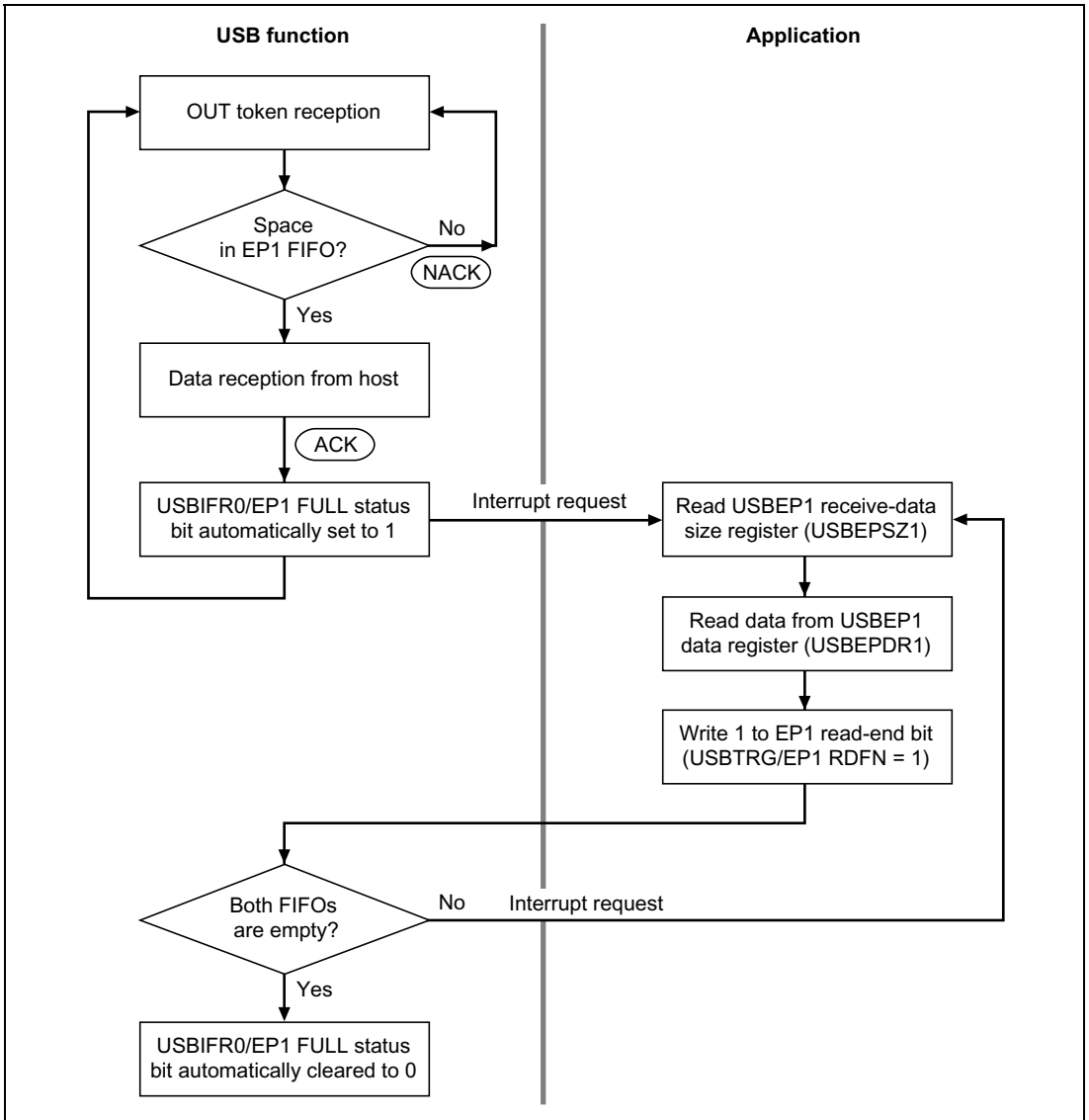
Figure 23.10 EP1 Bulk-Out Transfer Operation
