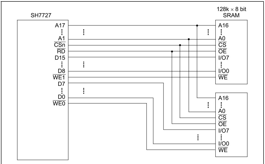
Figure 12.7 Example of 16-Bit Data-Width Static RAM Connection
