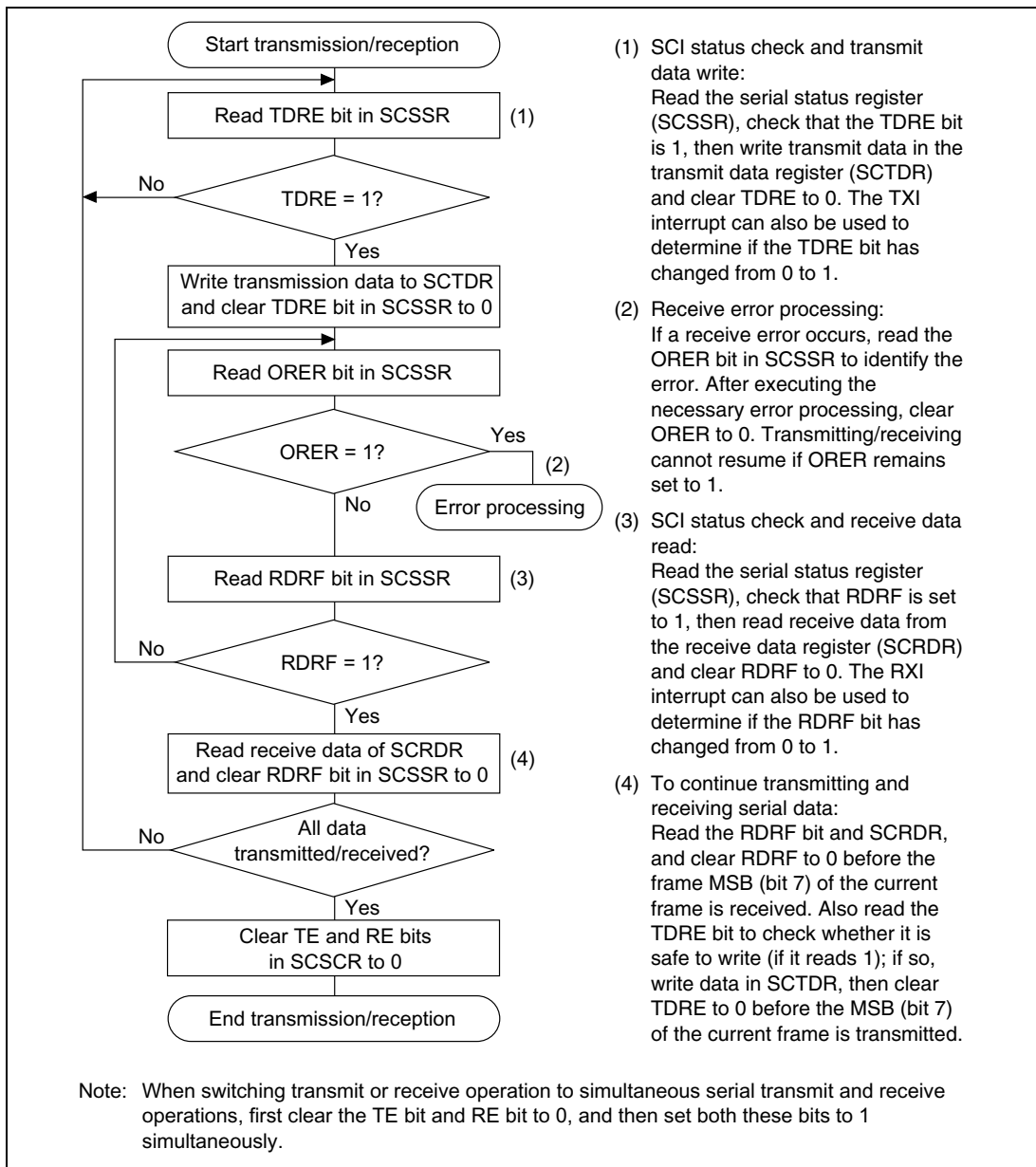
Figure 17.23 Sample Flowchart of Simultaneous Serial Transmit and Receive Operations
