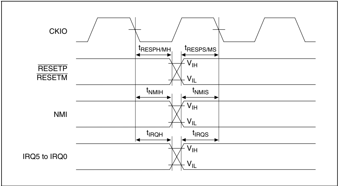
Figure 32.12 Interrupt signal Input Timing
