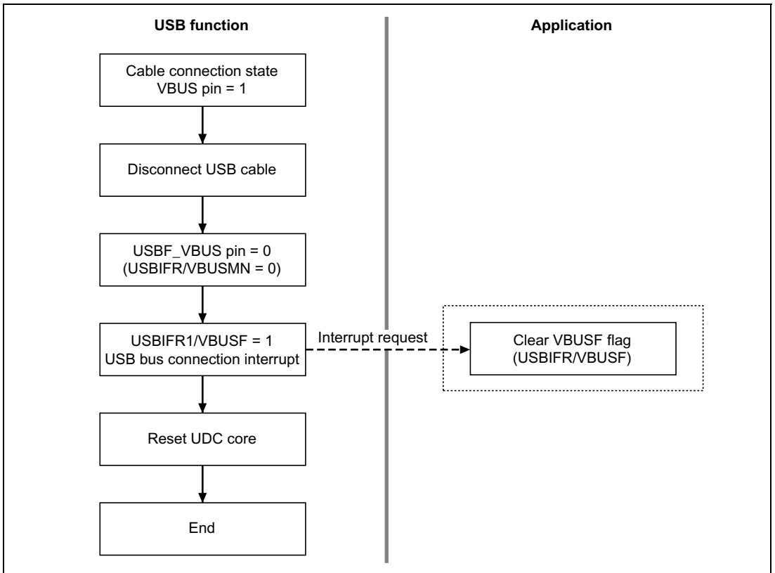
Figure 23.3 Cable Disconnection Operation
