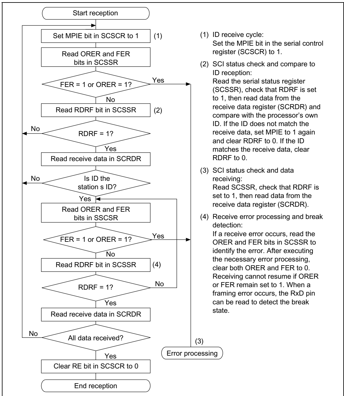
Figure 17.15 Sample Multiprocessor Serial Reception Flowchart (1)
