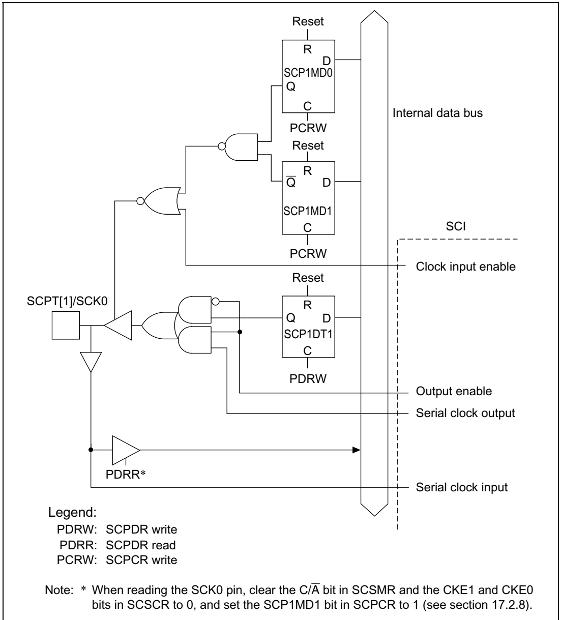
Figure 17.2 SCPT[1]/SCK0 Pin
