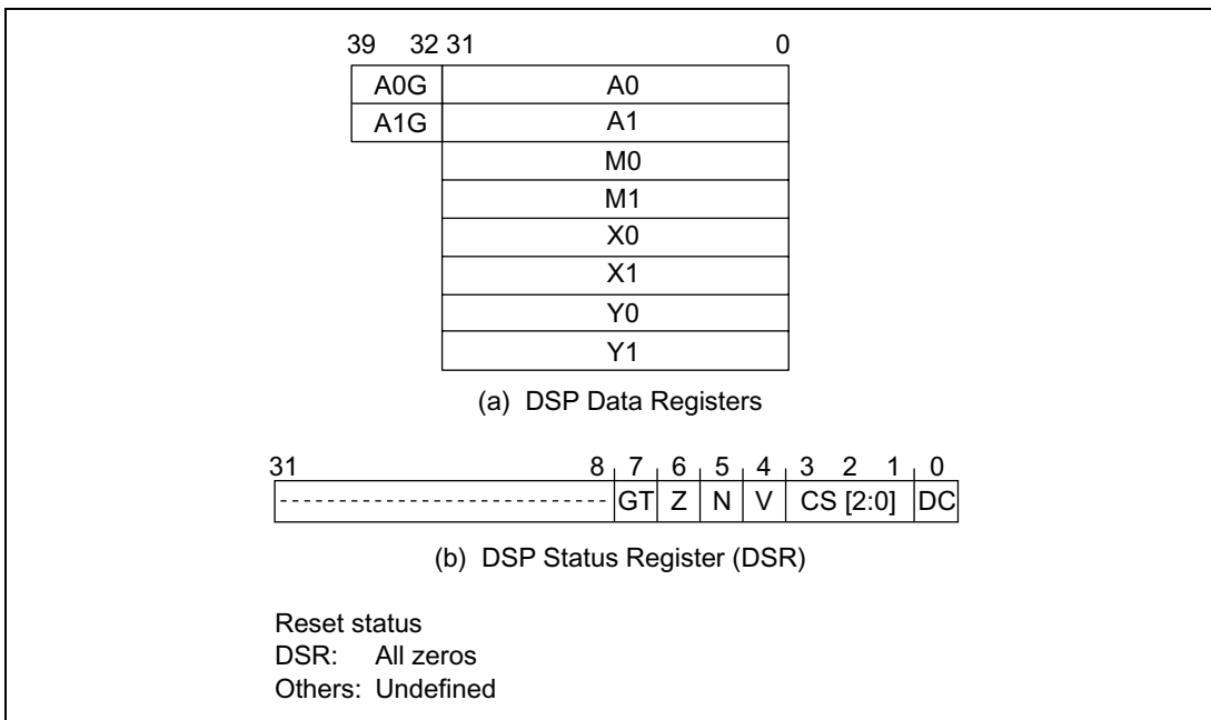
Figure 2.7 DSP Registers
