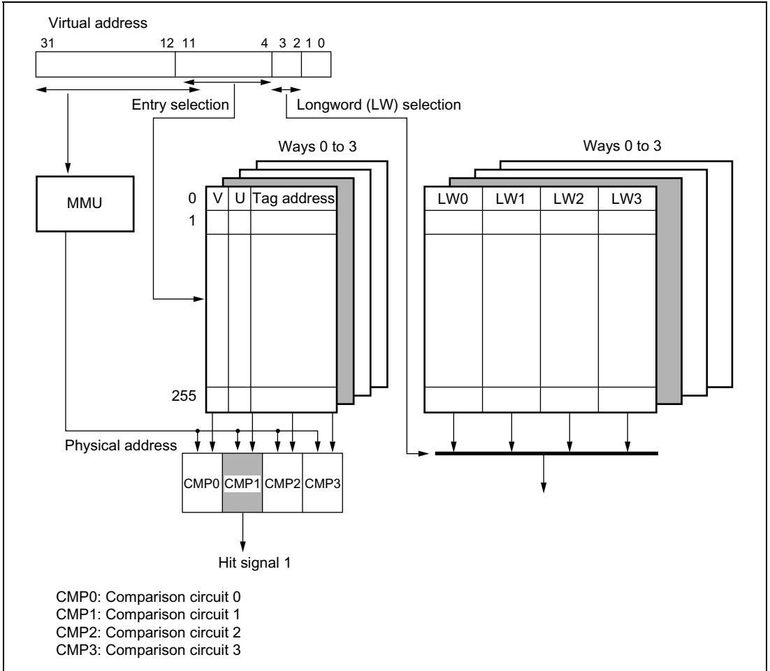
Figure 5.4 Cache Search Scheme
