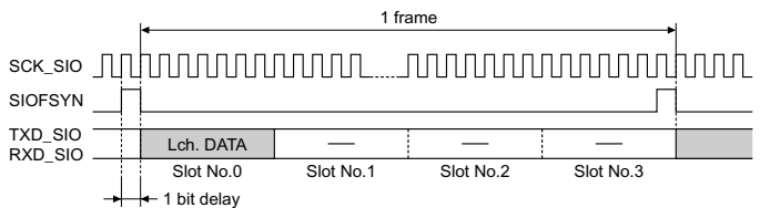
Figure 20.15 Transmit or Receive Timing (16 bits monaural—1)
