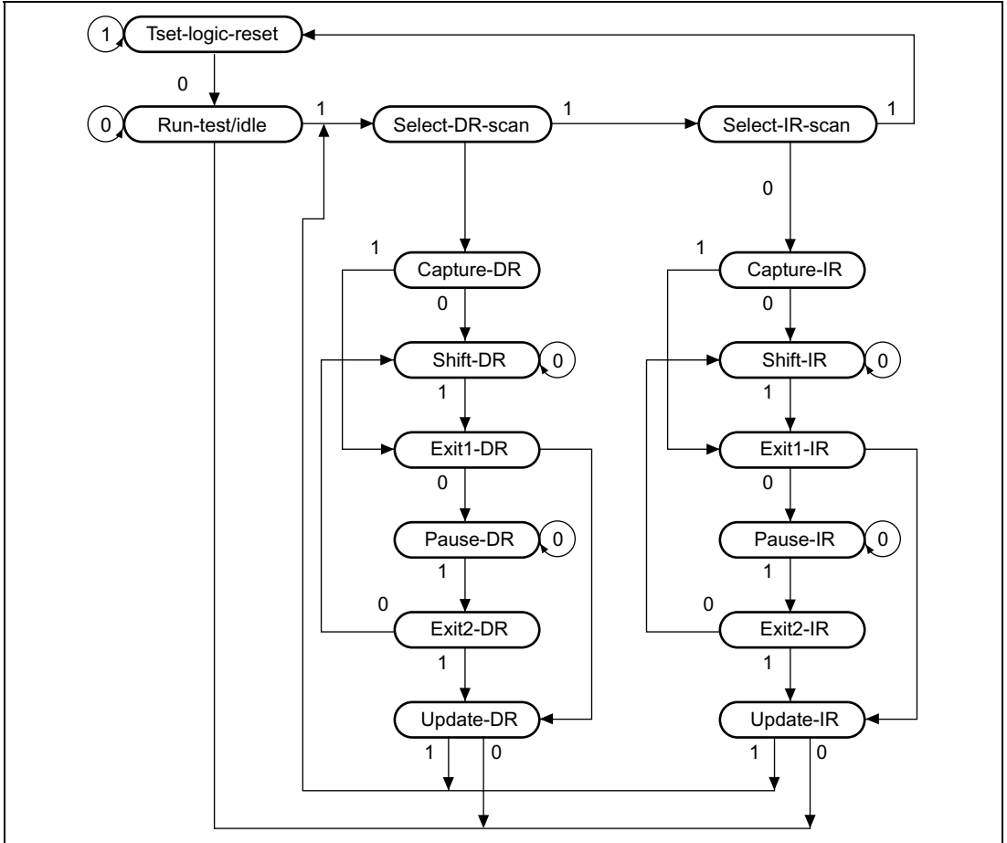
Figure 31.2 TAP Controller State Transitions
