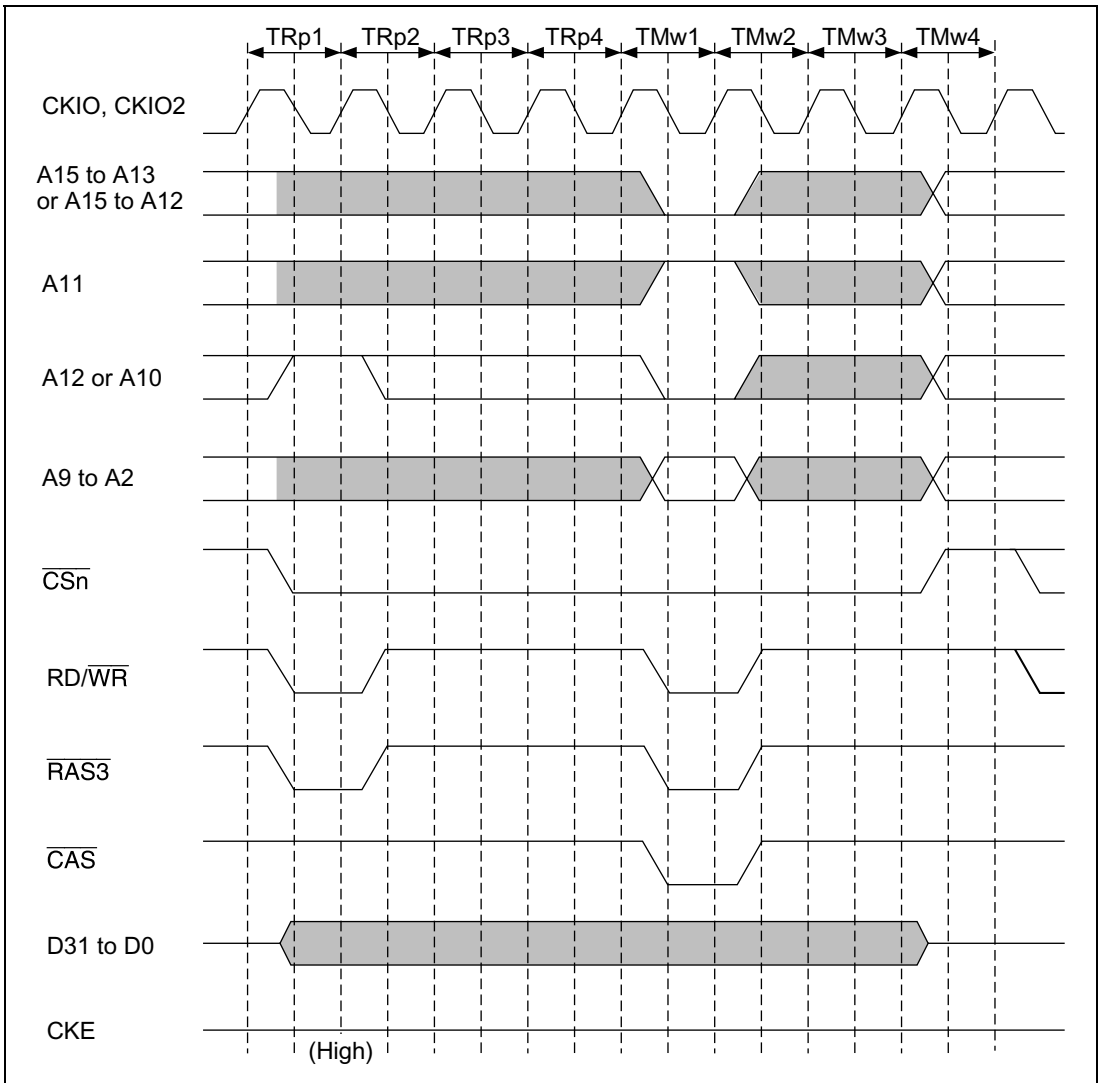
Figure 12.21 Synchronous DRAM Mode Write Timing
