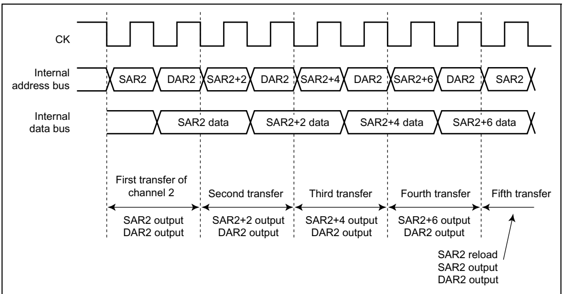
Figure 14.25 Timing Chart of Source Address Reload Function
