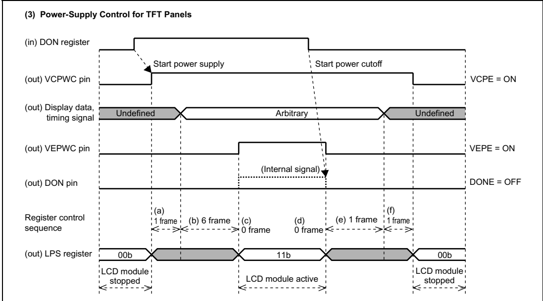
Figure 25.6 Power-Supply Control Sequence and States of the LCD Module
