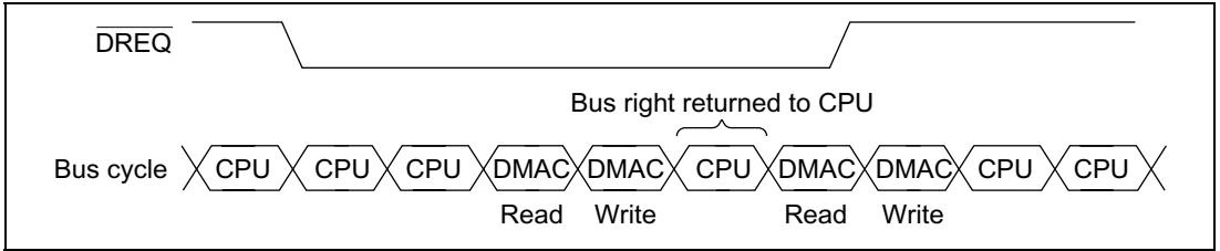
Figure 14.14 Transfer Example in Cycle-Steal Mode
