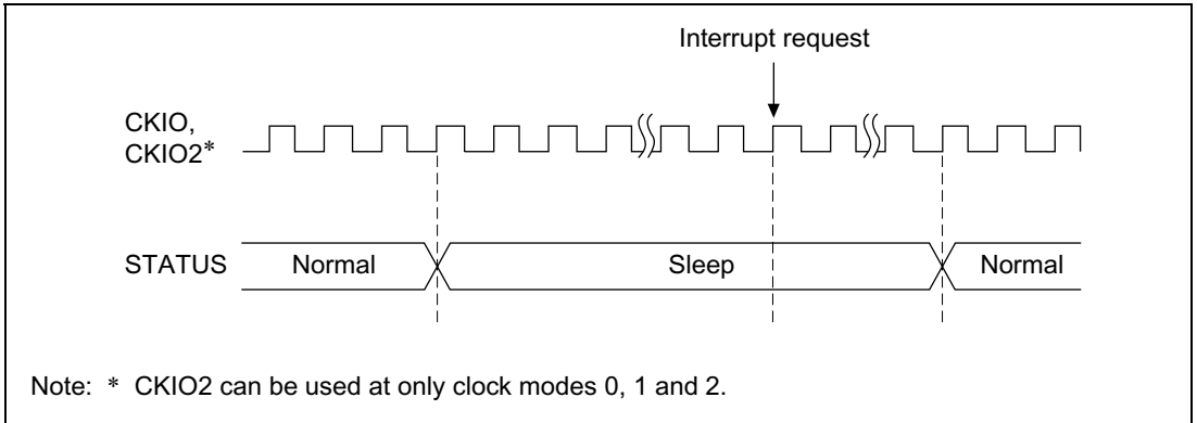
Figure 9.7 Sleep to Interrupt STATUS Output
