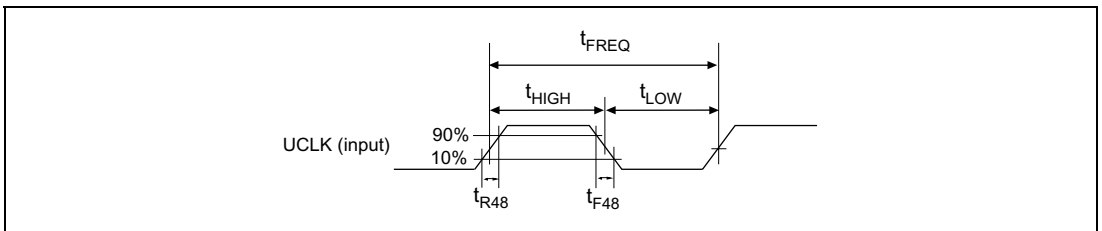
Figure 32.56 USB Clock Timing
