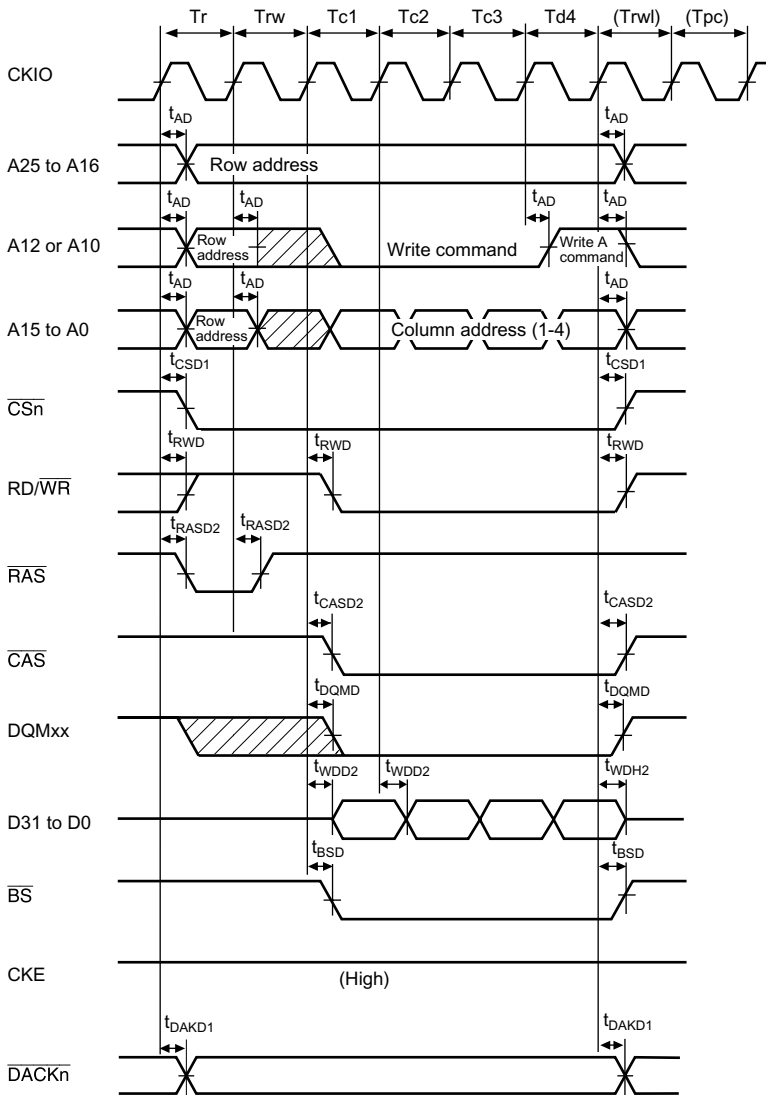
Figure 32.28 Synchronous DRAM Write Bus Cycle (Burst Mode (Single Write \times 4), RCD = 1, TPC = 0, TRWL = 0)
