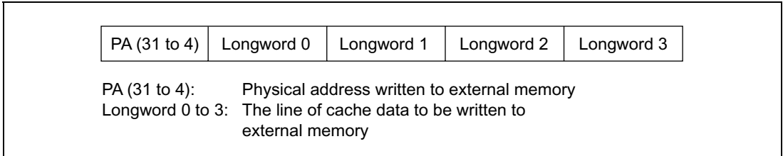
Figure 5.5 Write-Back Buffer Configuration
