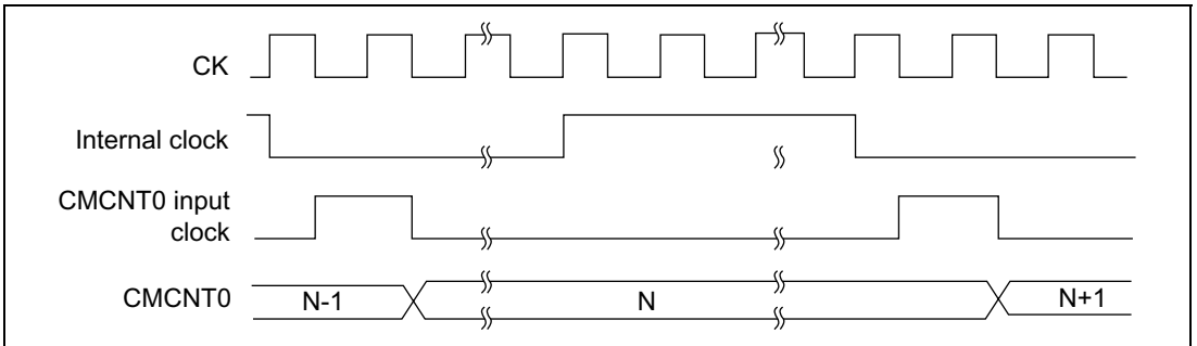
Figure 14.28 Count Timing
