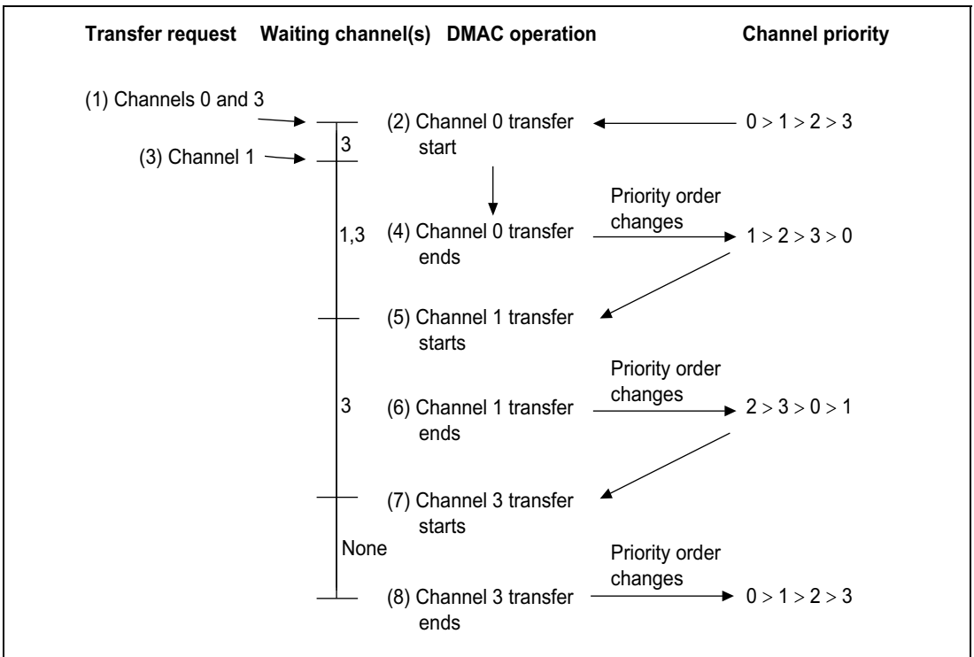
Figure 14.4 Channel Priority Order in Round-Robin Mode
