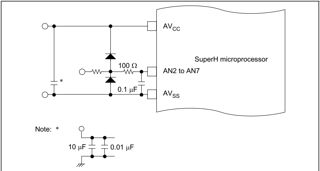
Figure 28.9 Example of Analog Input Protection Circuit
