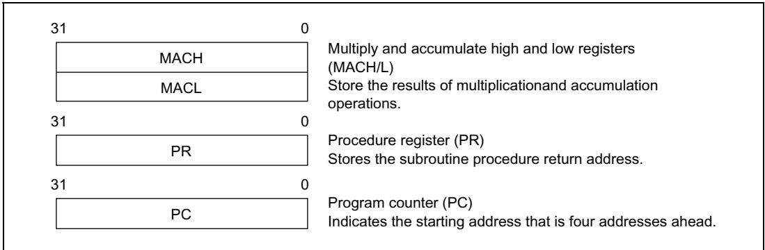
Figure 2.6 System Registers
