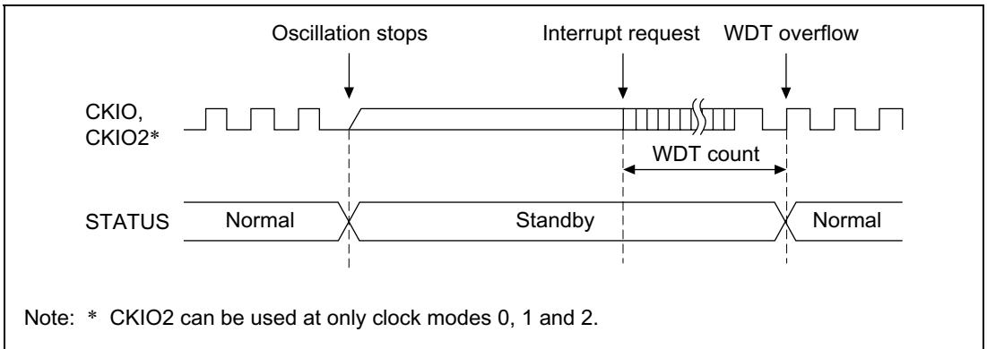
Figure 9.4 Standby to Interrupt STATUS Output
