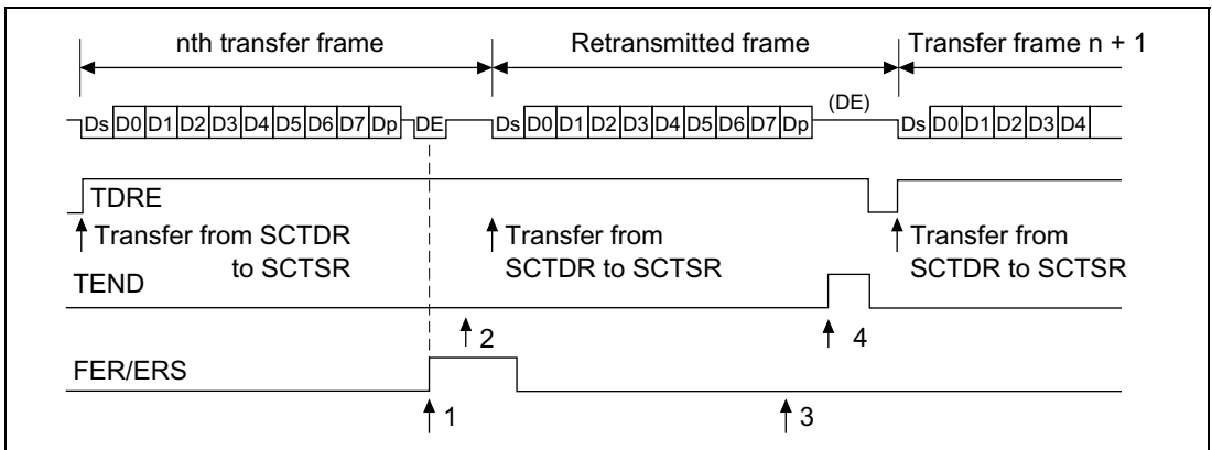
Figure 18.10 Retransmission in SCI Transmit Mode
