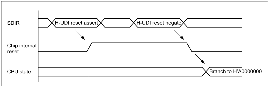
Figure 31.3 H-UDI Reset
