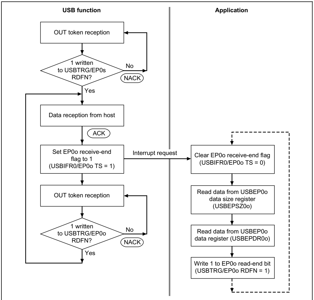
Figure 23.7 Data Stage Operation (Control-Out)
