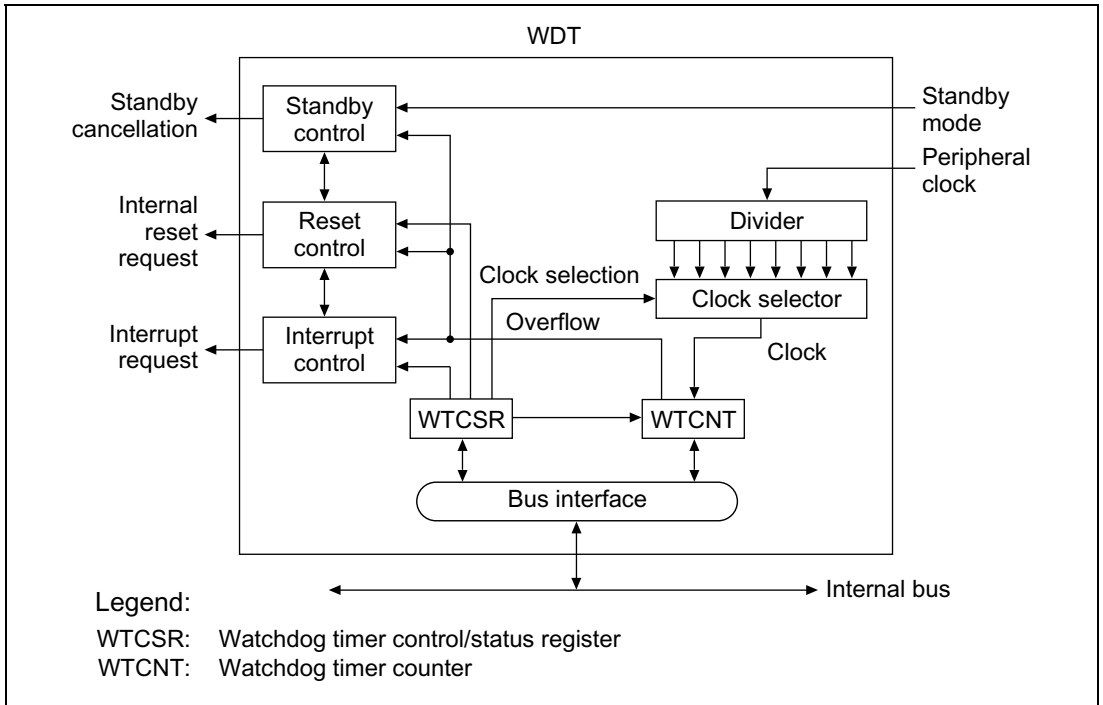
Figure 10.2 Block Diagram of the WDT
