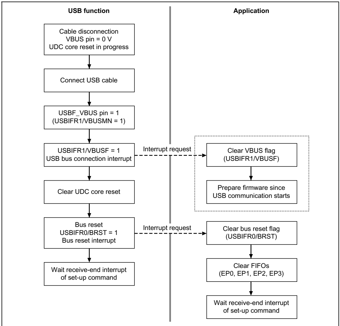
Figure 23.2 Cable Connection Operation
