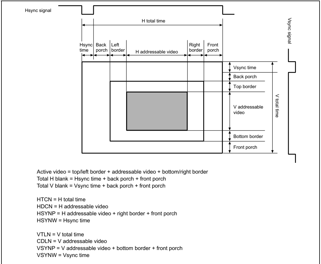
Figure 25.2 Valid Display and Retrace Period
