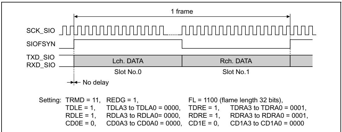
Figure 20.16 Transmit or Receive Timing (16 bits stereo—1)
