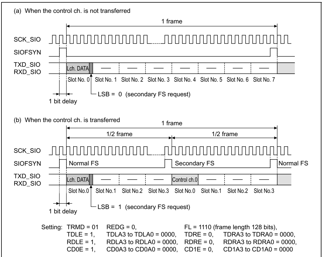
Figure 20.19 Transmit or Receive Timing (16 bits monaural—2)
