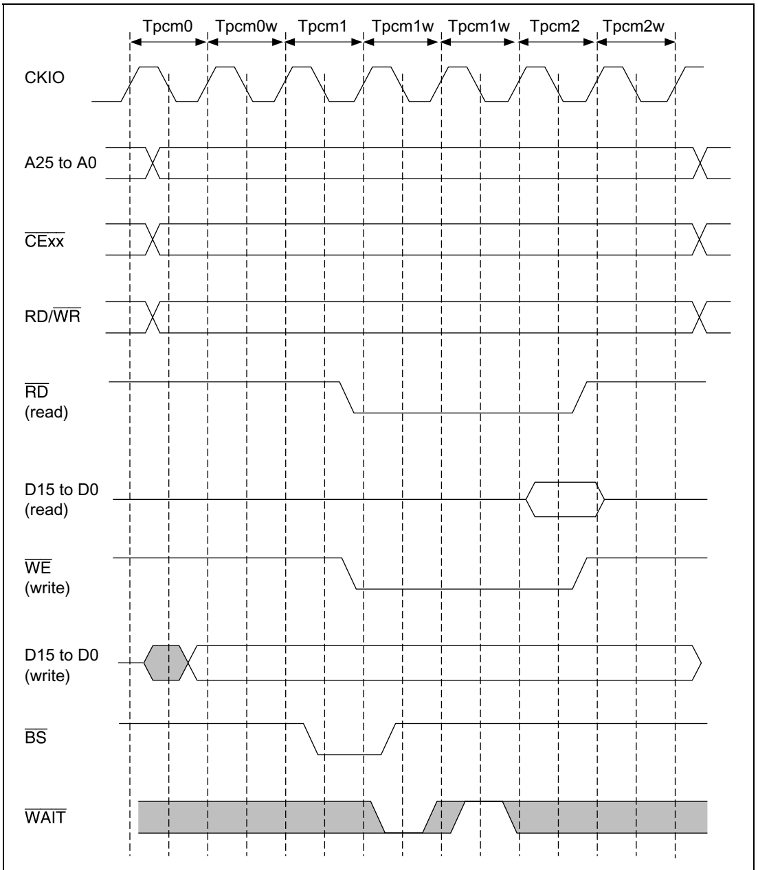
Figure 12.26 Wait Timing for PCMCIA Memory Card Interface
