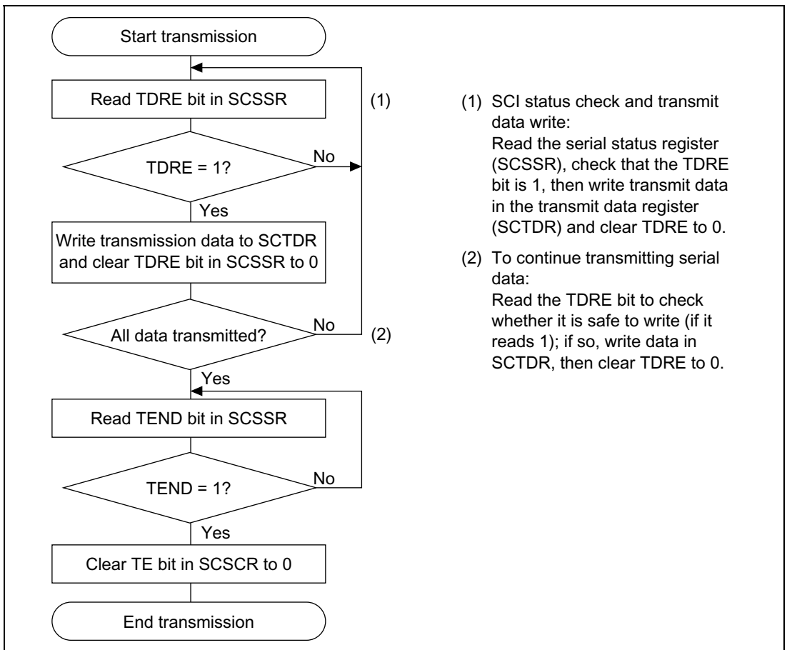
Figure 17.19 Sample Serial Transmission Flowchart
