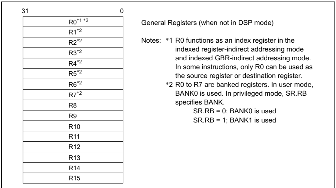
Figure 2.3 General Purpose Register (Not in DSP Mode)
