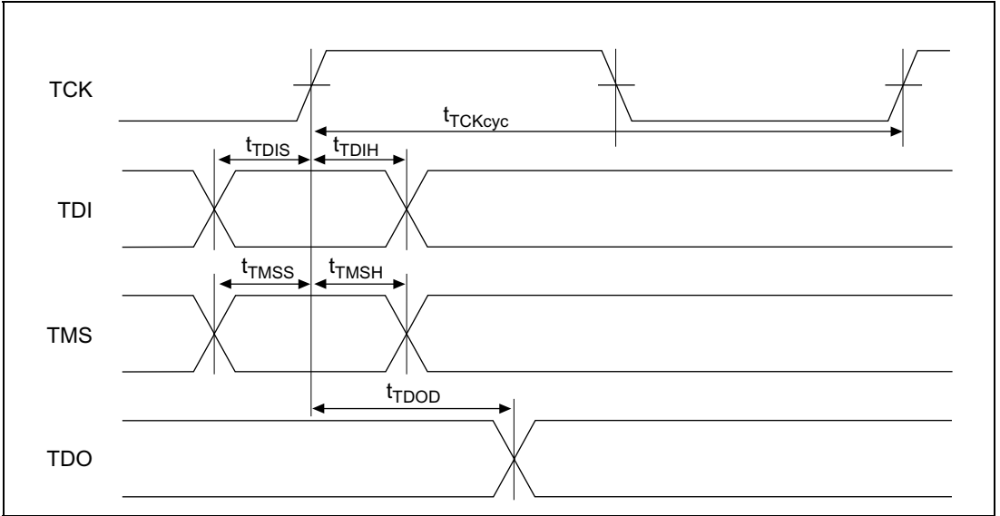
Figure 32.47 H-UDI Data Transfer Timing
