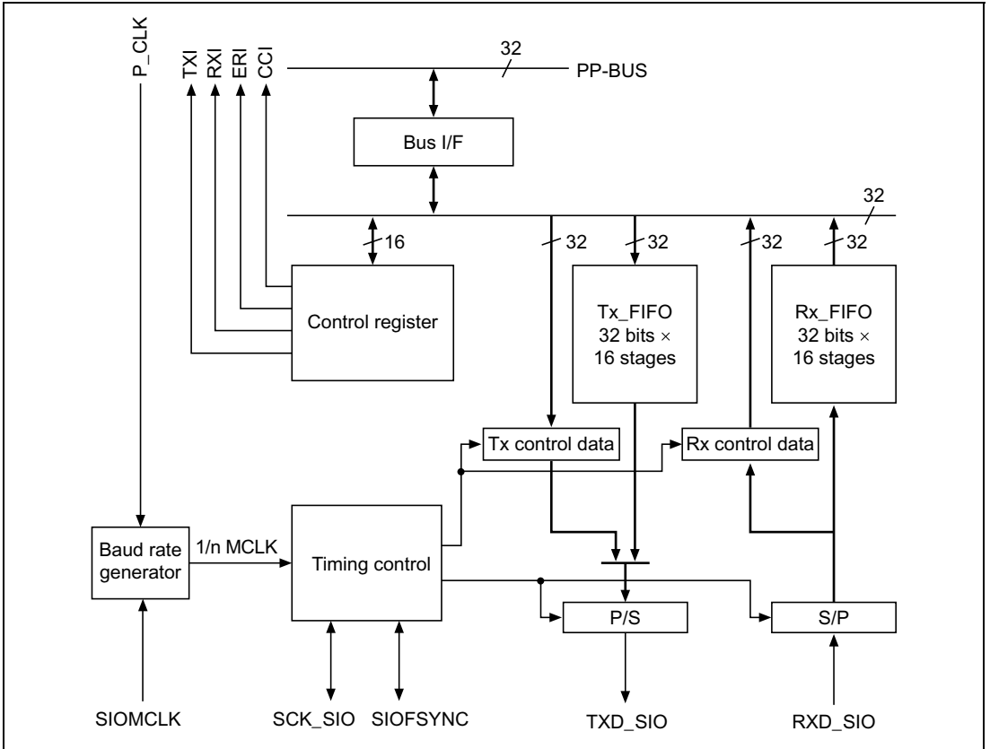
Figure 20.1 SIOF Block Diagram
