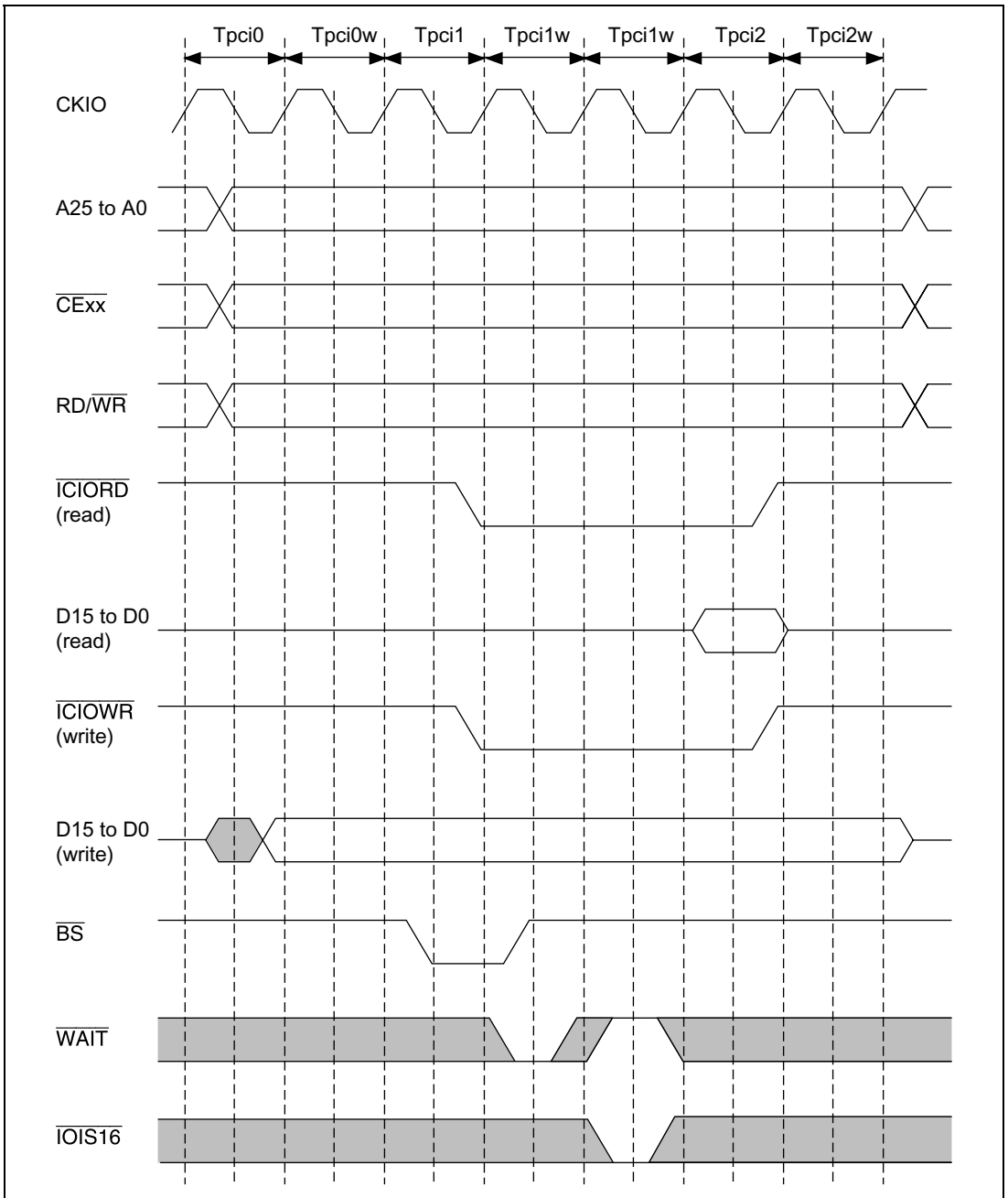
Figure 12.31 Wait Timing for PCMCIA I/O Card Interface
