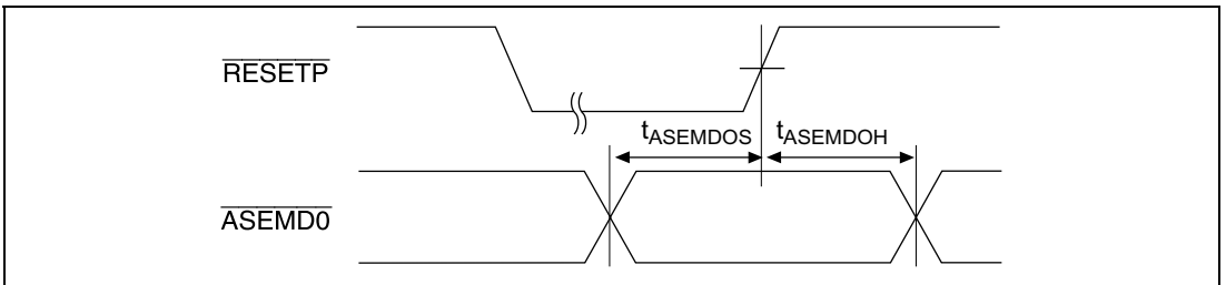
Figure 32.48 ASEMD0 Input Timing
