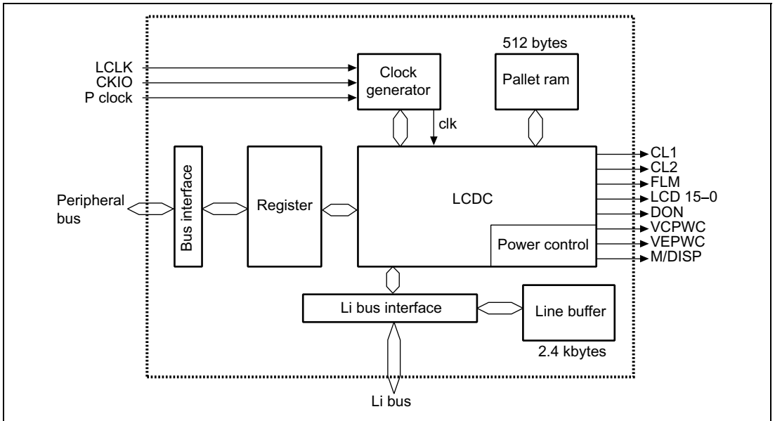
Figure 25.1 Block Diagram
