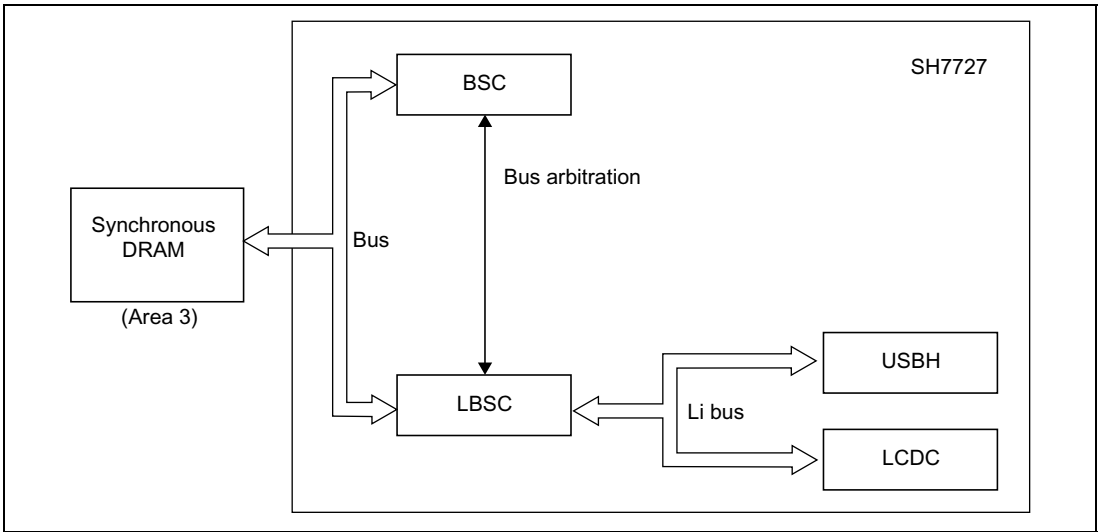
Figure 13.1 Block Diagram of Li Bus Architecture
