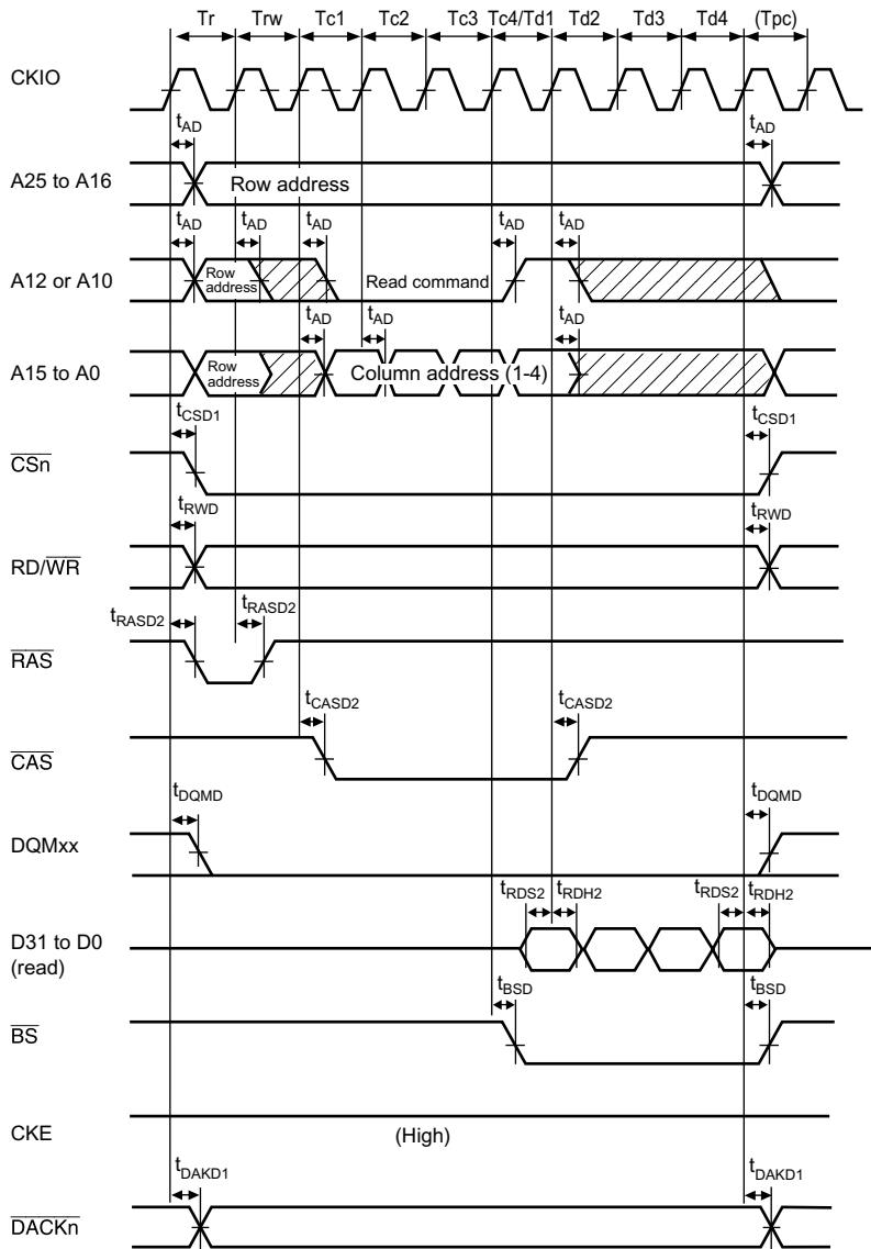
Figure 32.24 Synchronous DRAM Read Bus Cycle (Burst Read (Single Read \times 4), RCD = 1, CAS Latency = 3, TPC = 0)
