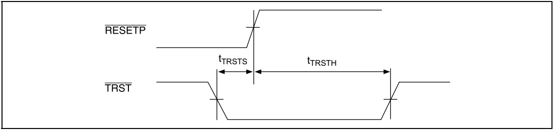
Figure 32.46 TRST Input Timing (Reset Hold)
