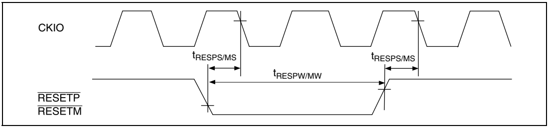
Figure 32.11 Reset Input Timing
