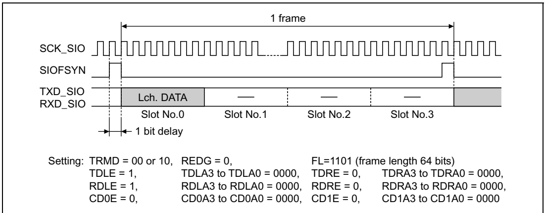
Figure 20.15 Transmit or Receive Timing (16 bits monaural—1)
