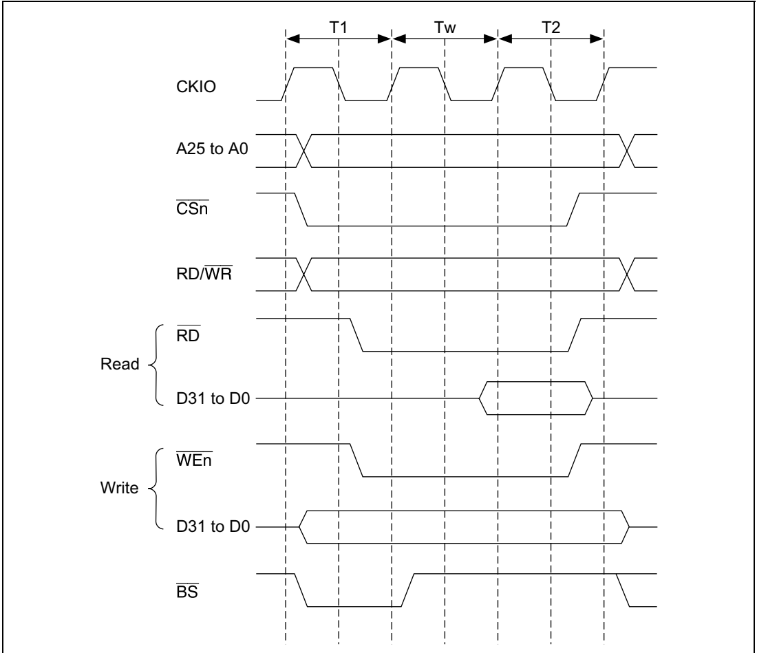
Figure 12.9 Basic Interface Wait Timing (Software Wait Only)
