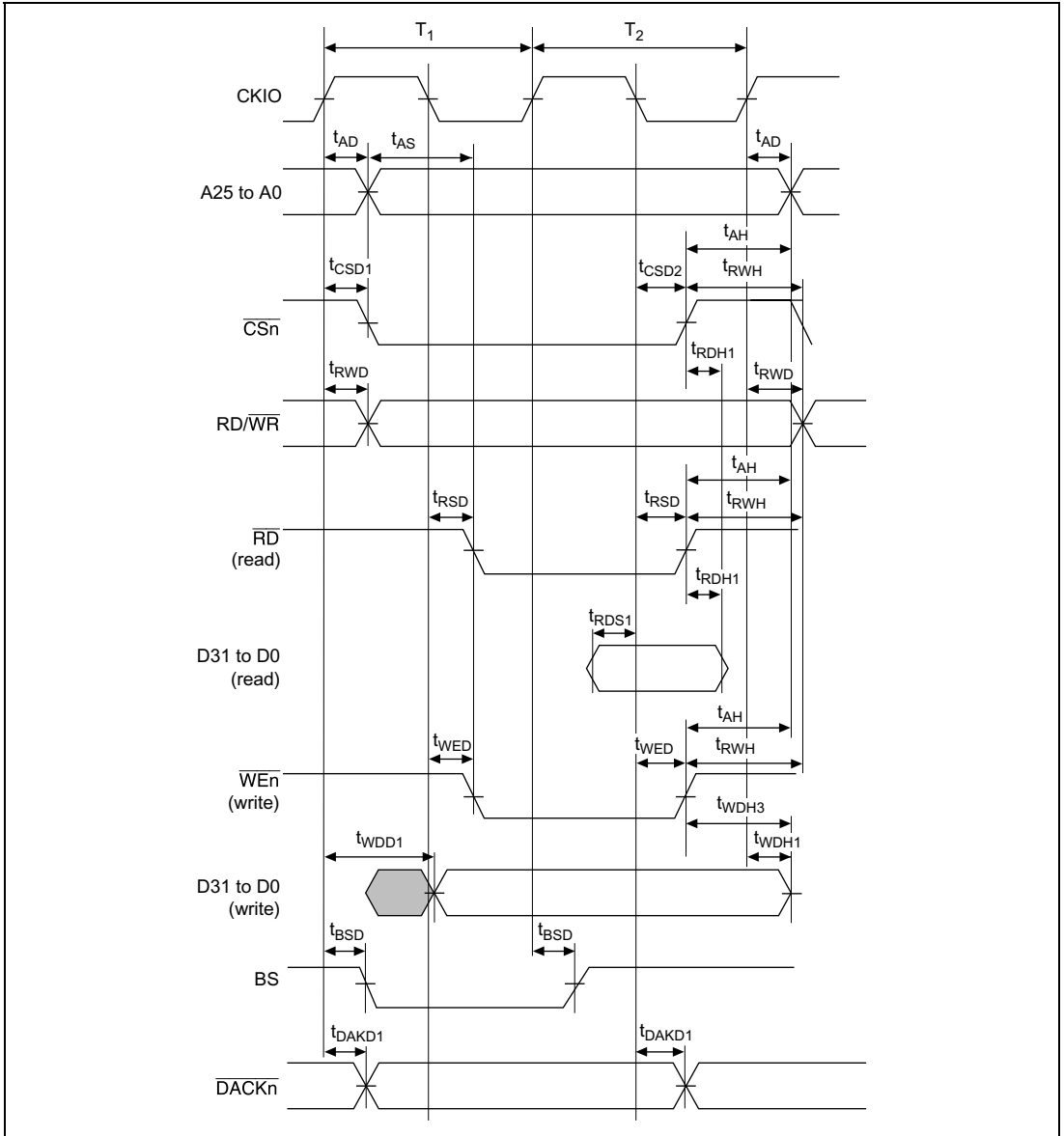
Figure 32.15 Basic Bus Cycle (No Wait)
