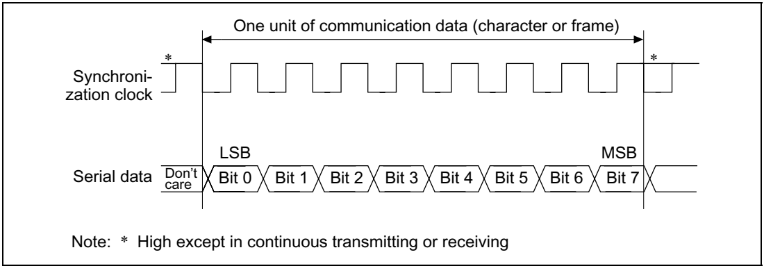
Figure 17.17 Data Format in Clock Synchronous Communication
