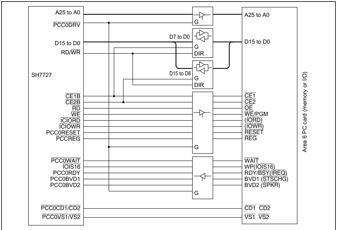
Figure 30.4 SH7727 Interface
