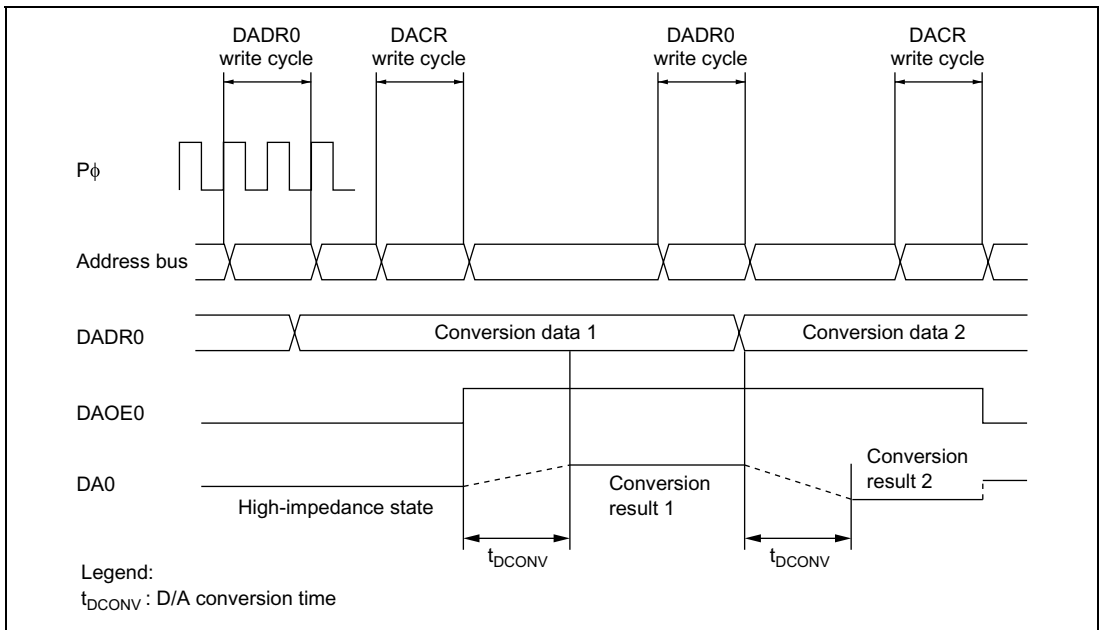
Figure 29.2 Example of D/A Converter Operation
