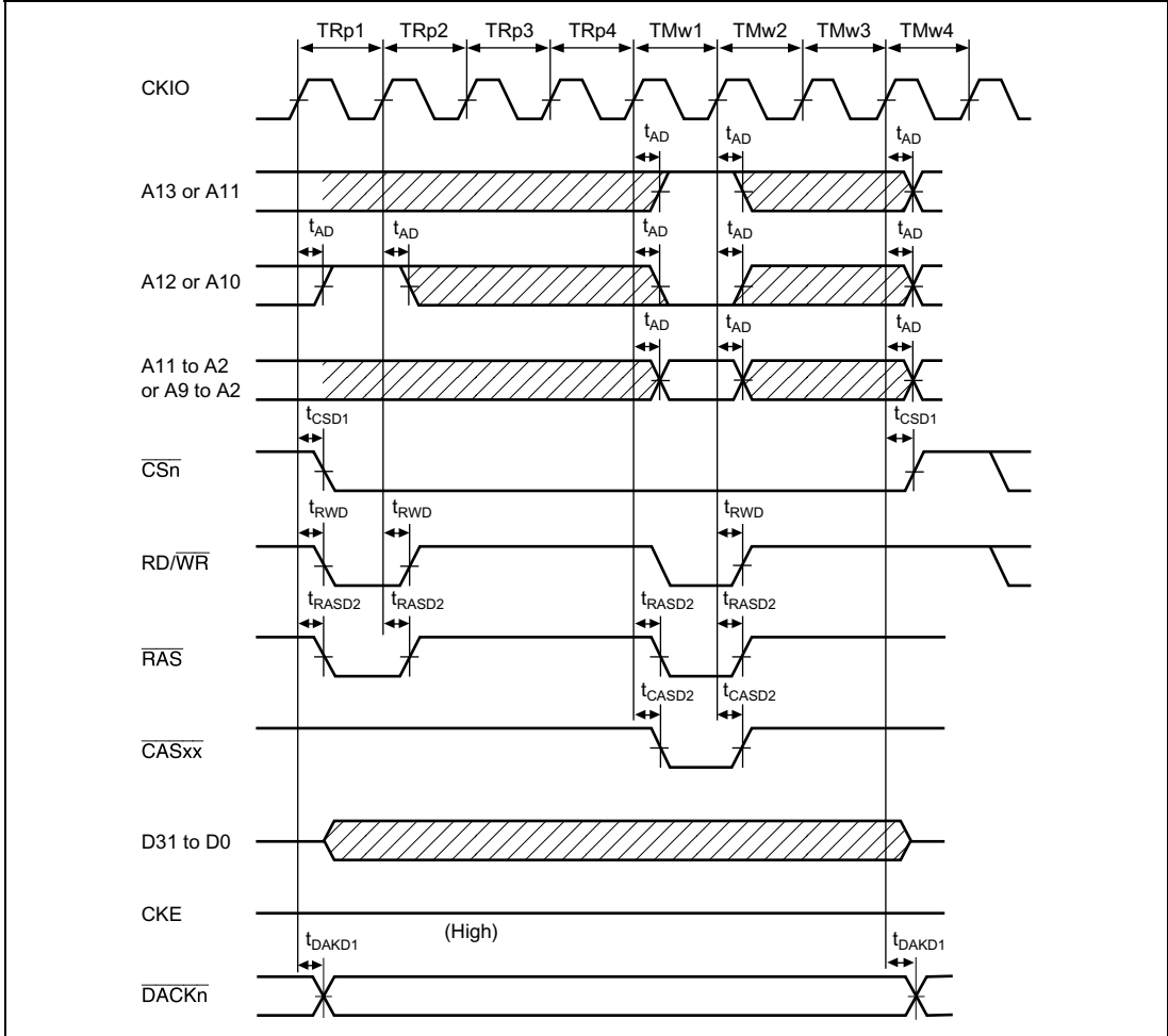
Figure 32.31 Synchronous DRAM Mode Register Write Cycle
