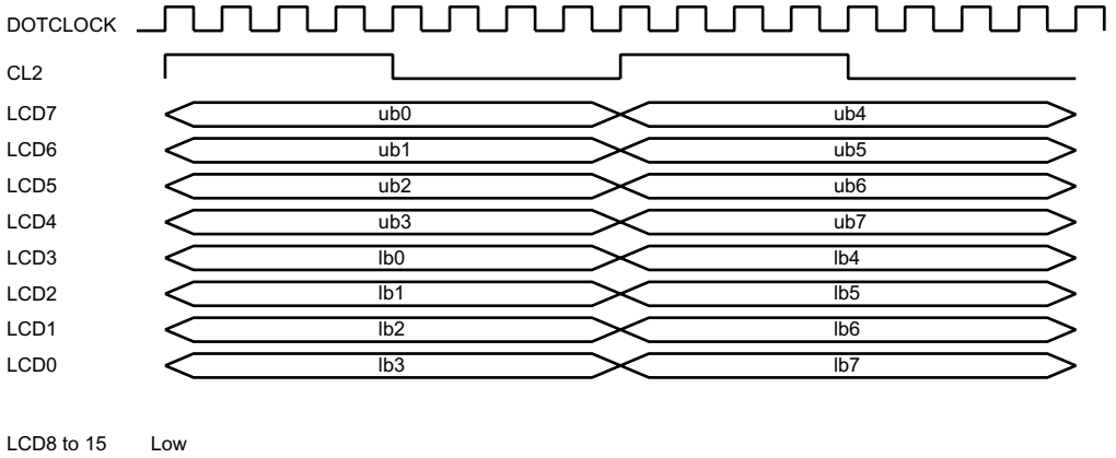
Figure 25.14 Clock and LCD Data Signal Example
