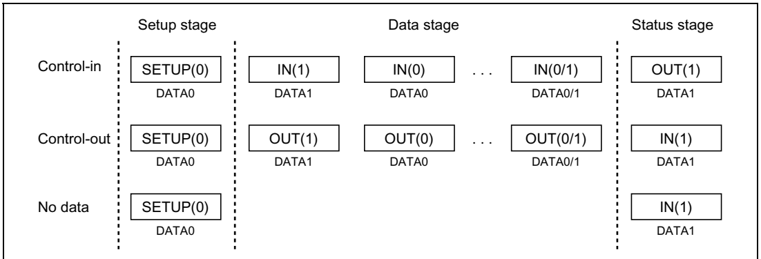
Figure 23.4 Transfer Stage for Control Transfer
