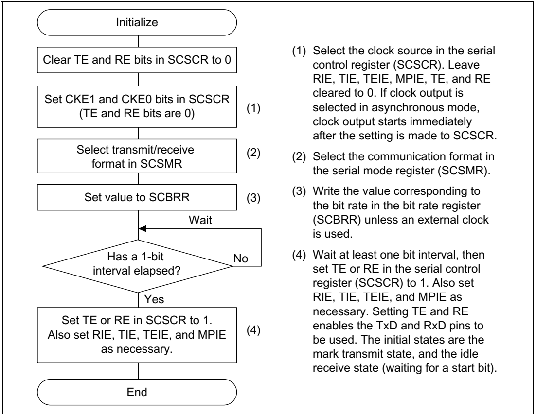
Figure 17.7 Sample SCI Initialization Flowchart
