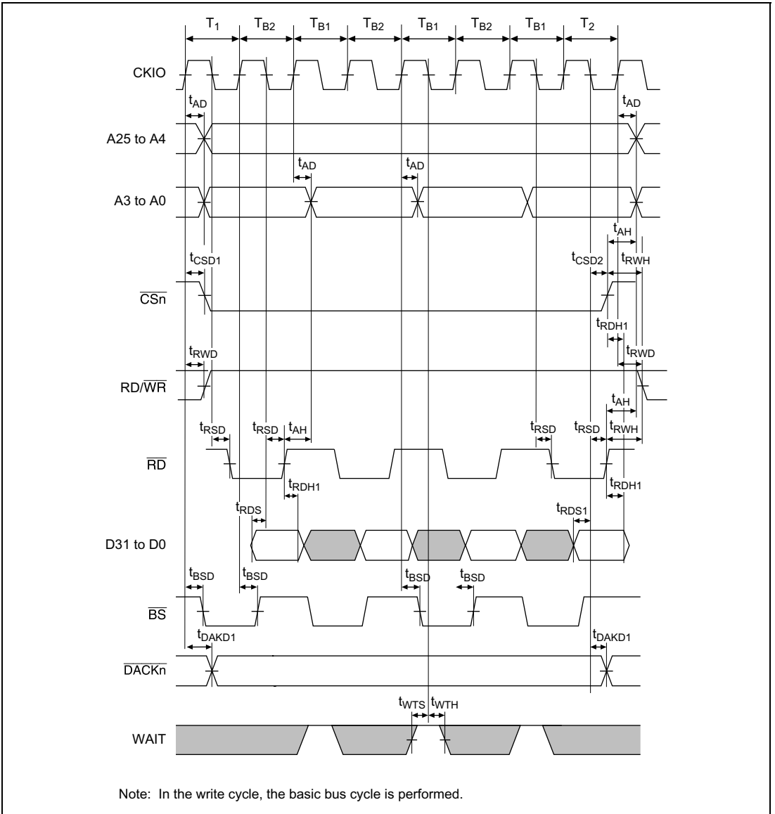
Figure 32.18 Burst ROM Bus Cycle (No Wait)
