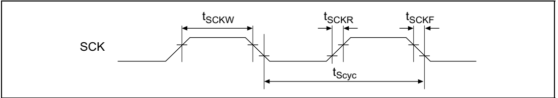
Figure 32.40 SCK Input Clock Timing
