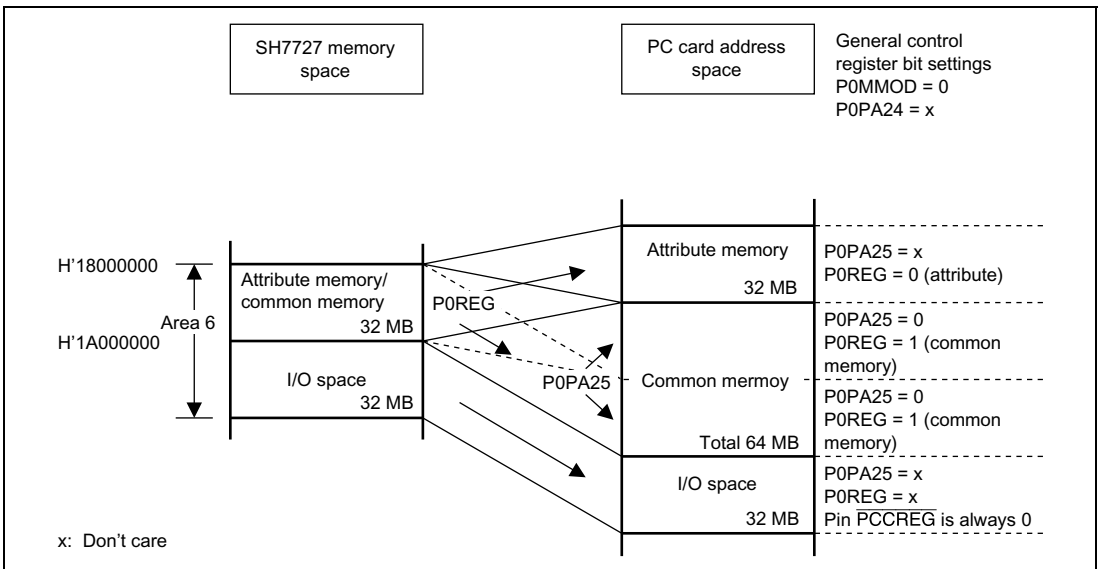
Figure 30.2 Continuous 32-MB Area Mode
