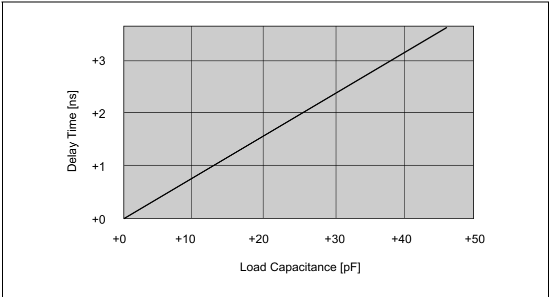
Figure 32.59 Load Capacitance vs. Delay Time
