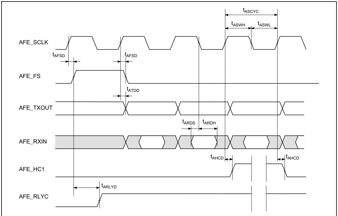
Figure 32.57 AFEIF Module AC Timing
