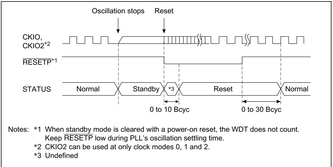
Figure 9.5 Standby to Power-On Reset STATUS Output
