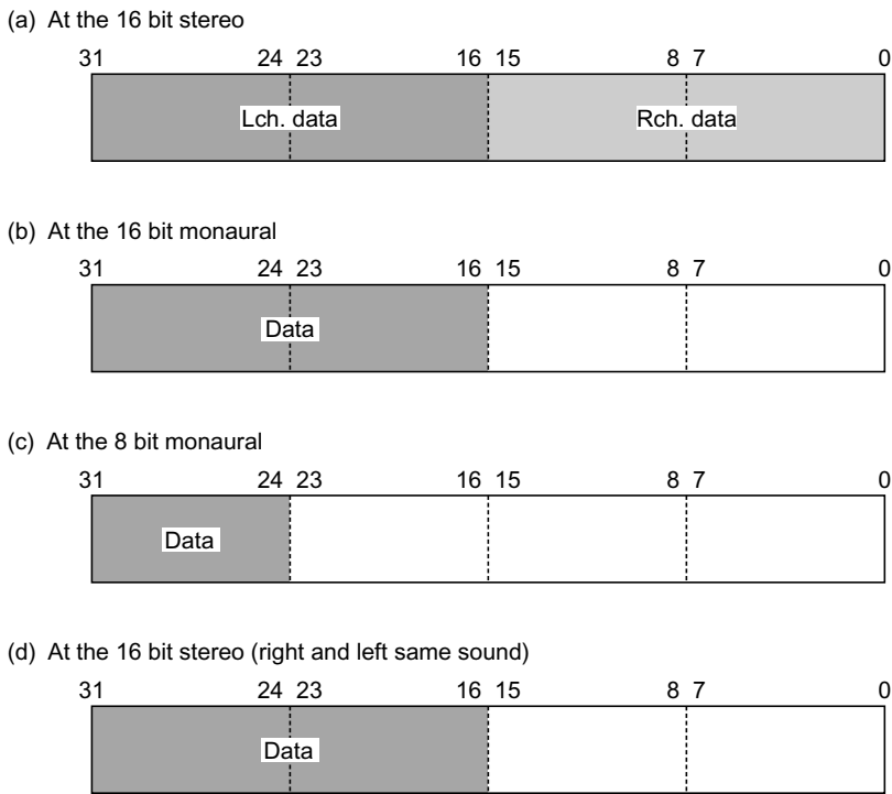
Figure 20.5 Transmit or Receive Data Bit Alignment
