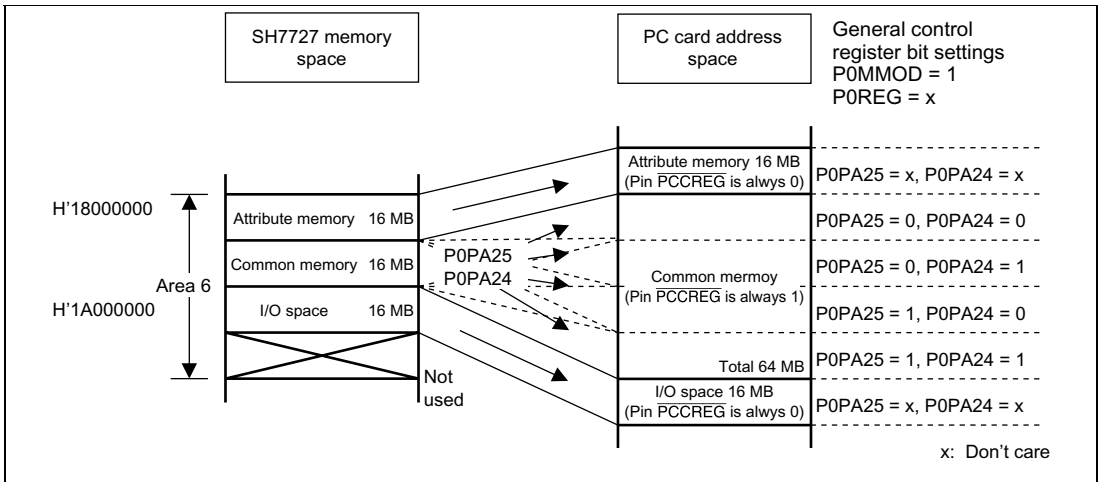
Figure 30.3 Continuous 16-MB Area Mode (Area 6)
