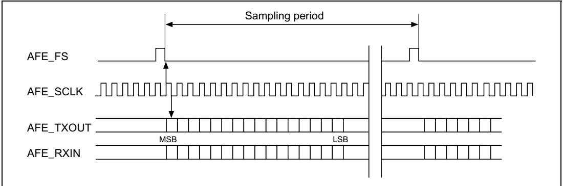
Figure 21.5 AFE Serial Interface
