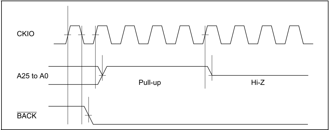
Figure 12.34 Pins A25 to A0 Pull-Up Timing
