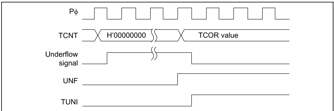
Figure 15.6 UNF Set Timing
