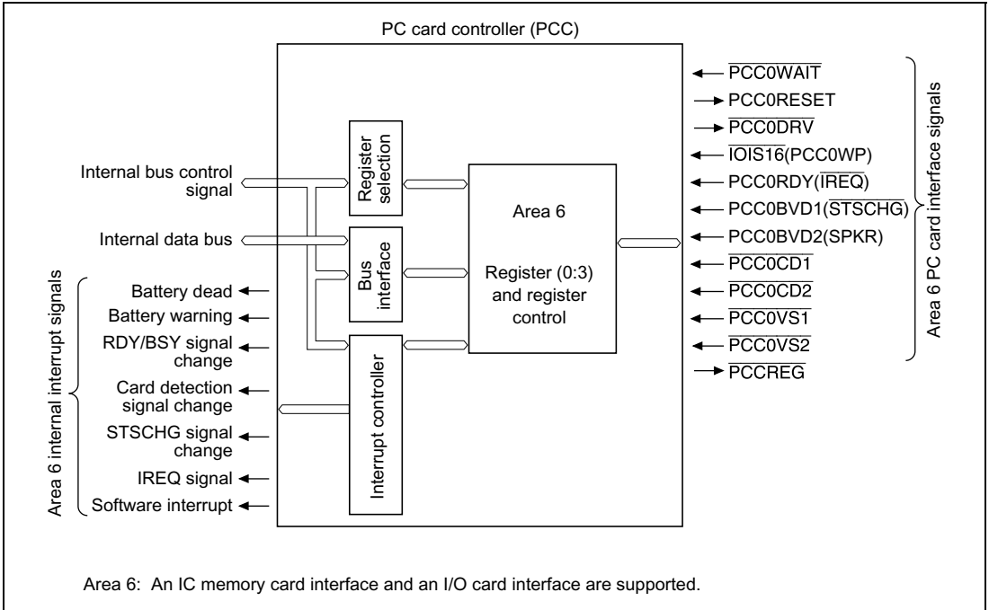
Figure 30.1 PC Card Controller Block Diagram
