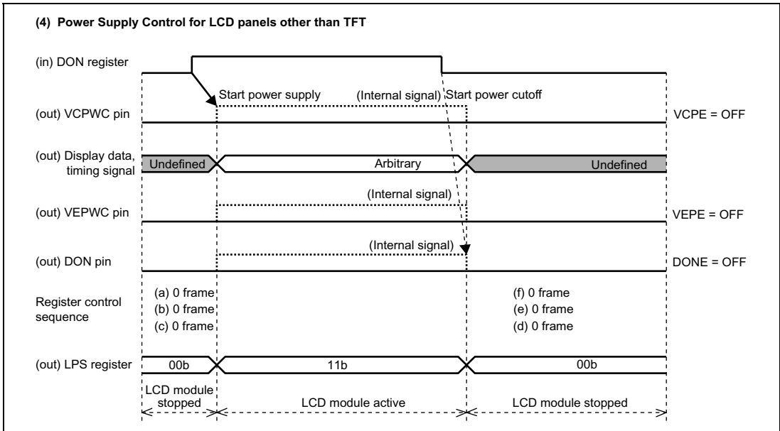
Figure 25.7 Power-Supply Control Sequence and States of the LCD Module
