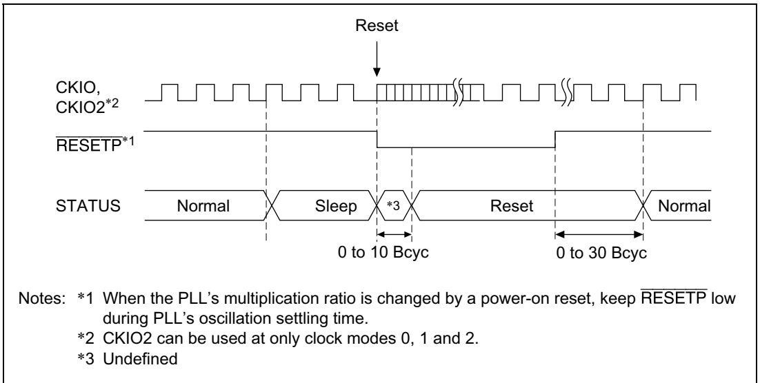
Figure 9.8 Sleep to Power-On Reset STATUS Output
