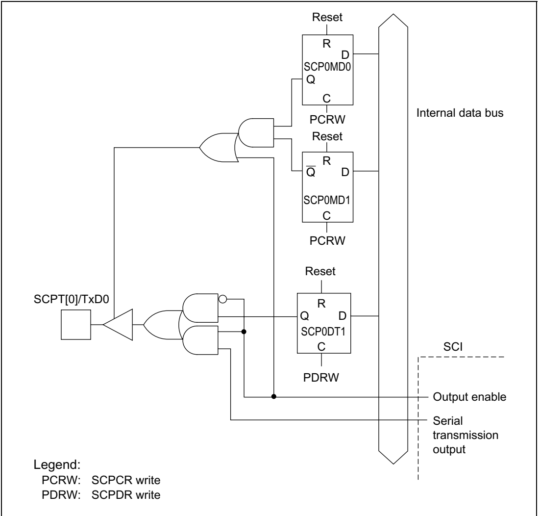
Figure 17.3 SCPT[0]/TxD0 Pin
