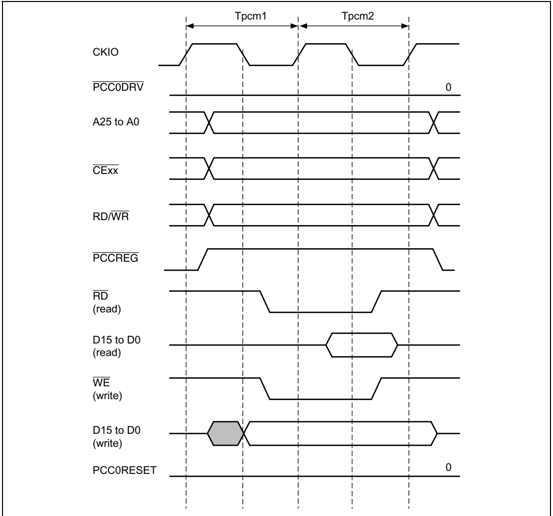
Figure 30.5 PCMCIA Memory Card Interface Basic Timing
