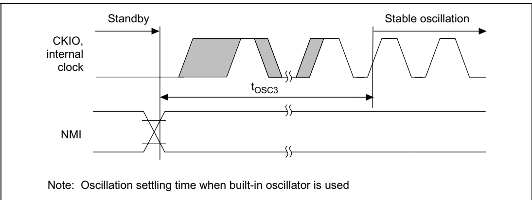
Figure 32.6 Oscillation Settling Time at Standby Return (Return by NMI)
