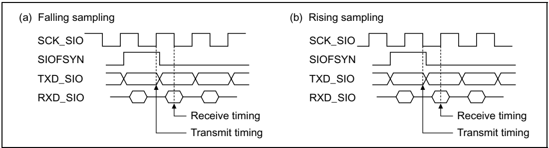
Figure 20.4 SIOF Transmit or Receive Timing
