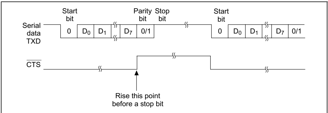
Figure 19.7 Example of Operation Using Modem Control ( \overline{\text{CTS}} )
