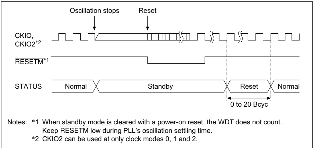
Figure 9.6 Standby to Manual Reset STATUS Output
