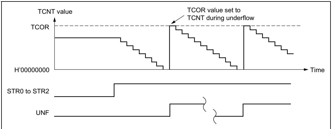
Figure 15.3 Auto-Reload Counter Operation
