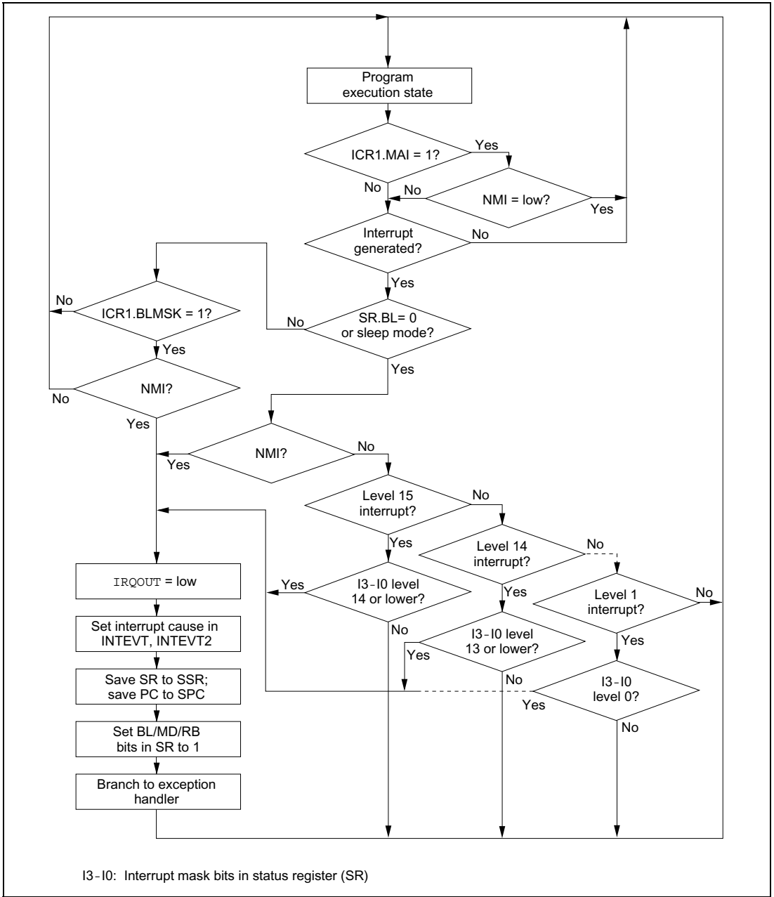
Figure 7.3 Interrupt Operation Flowchart
