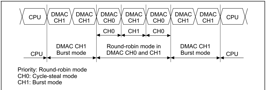
Figure 14.16 Bus State in Multiple Channel Operation
