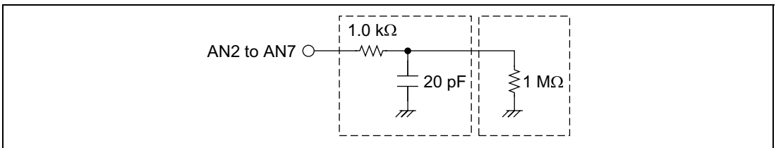
Figure 28.10 Analog Input Pin Equivalent Circuit
