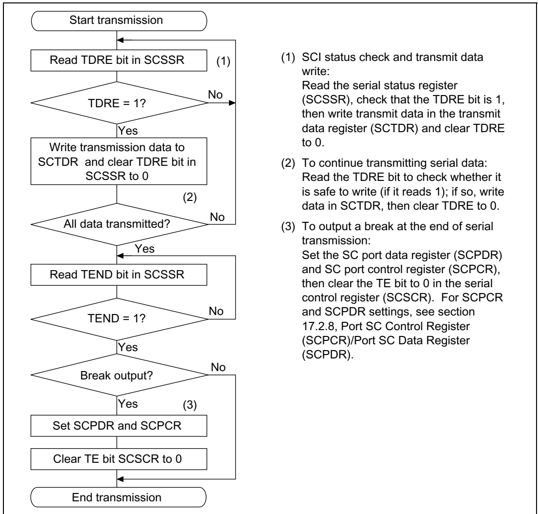
Figure 17.8 Sample Serial Transmission Flowchart
