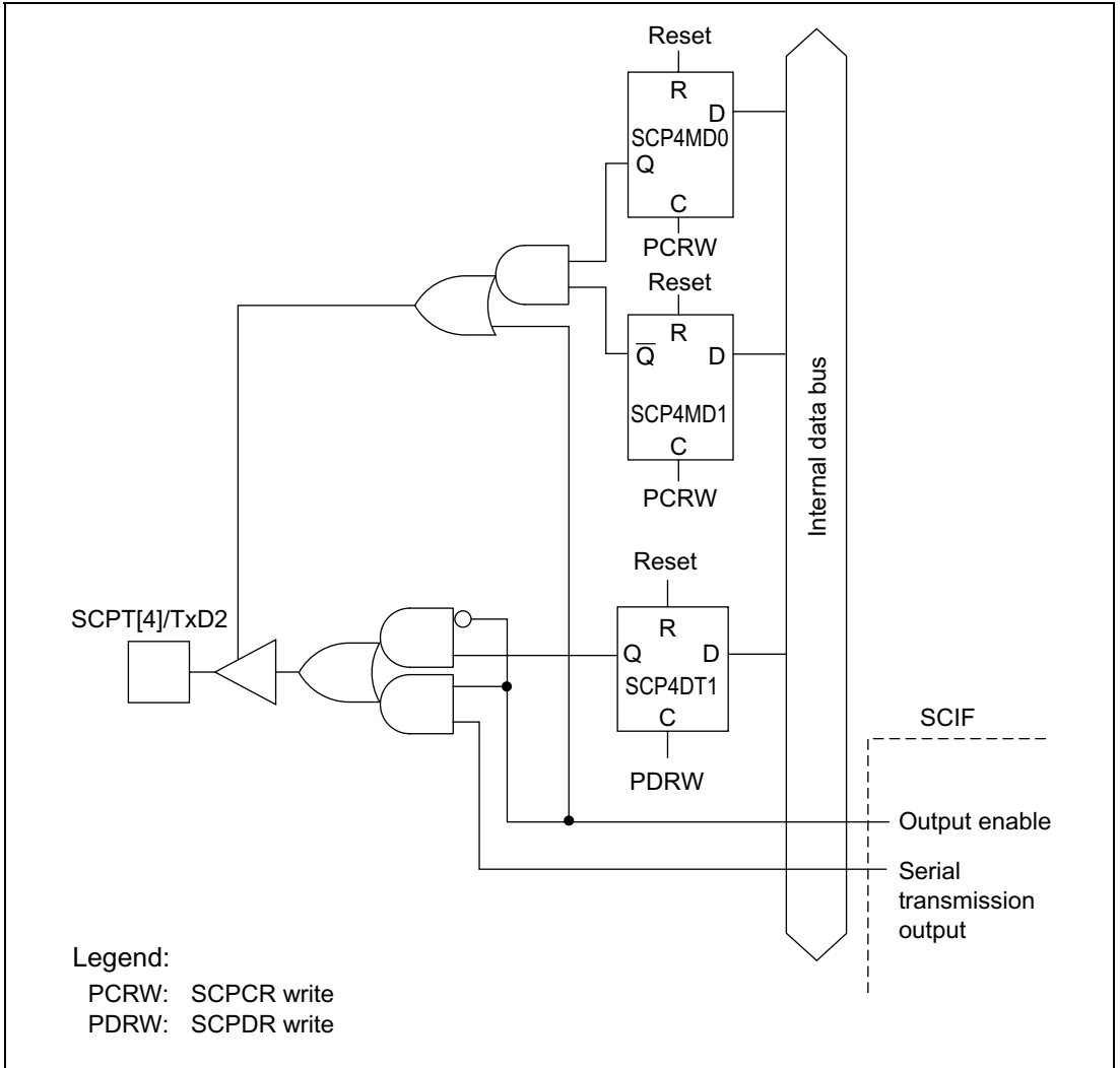
Figure 19.2 SCPT[4]/TxD2 Pin
