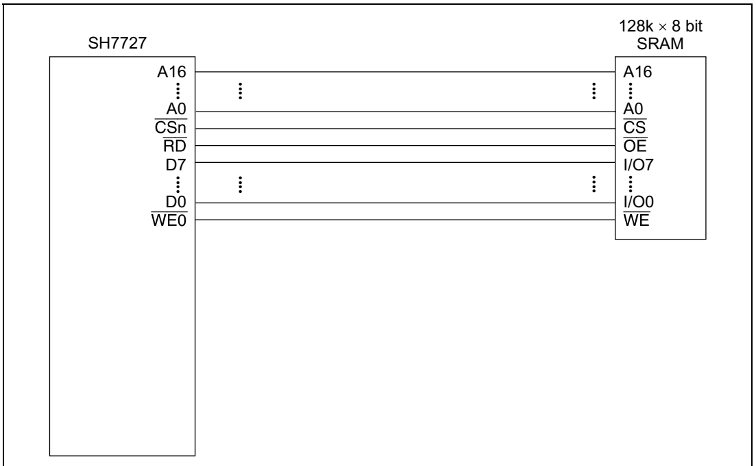
Figure 12.8 Example of 8-Bit Data-Width Static RAM Connection
