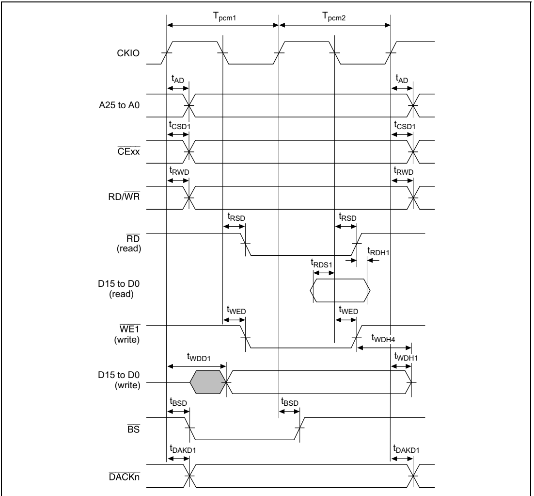
Figure 32.32 PCMCIA Memory Bus Cycle (TED = 0, TEH = 0, No Wait)
