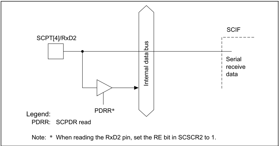
Figure 19.3 SCPT[4]/RxD2 Pin
