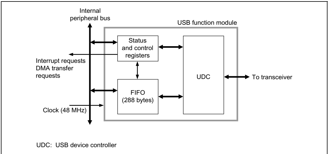
Figure 23.1 Block Diagram of UBC
