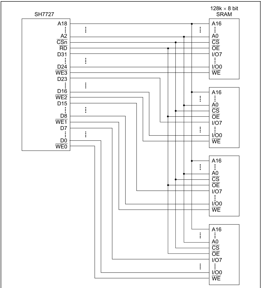
Figure 12.6 Example of 32-Bit Data-Width Static RAM Connection
