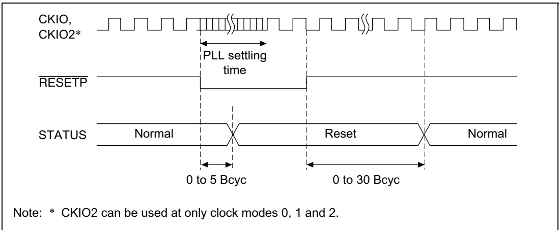
Figure 9.2 Power-On Reset (Clock Modes 0, 1, 2, and 7) STATUS Output
