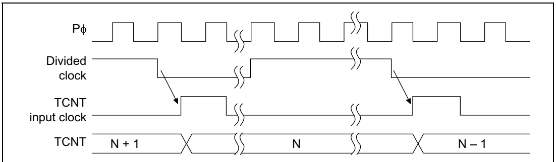
Figure 15.4 Count Timing when Internal Clock is Operating
