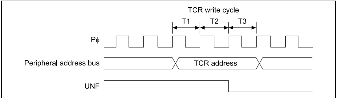
Figure 15.7 Status Flag Clear Timing
