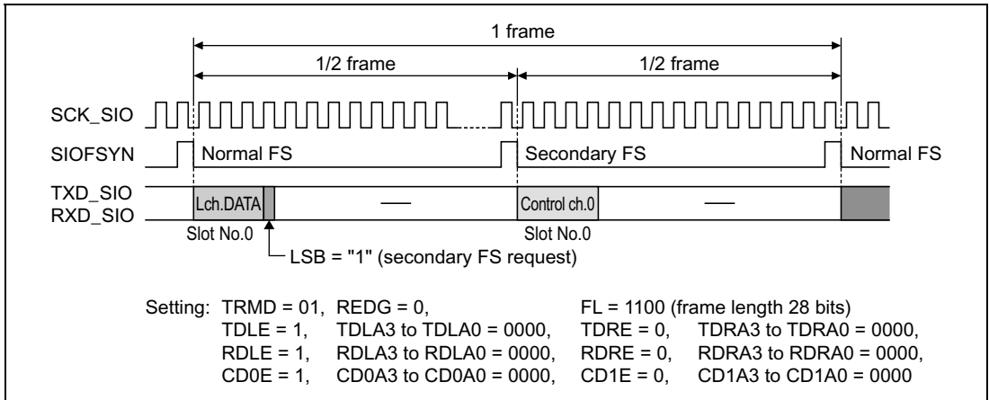
Figure 20.8 Control Data Interface (Secondary FS)
