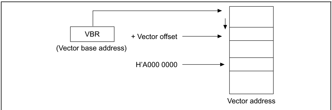
Figure 4.1 Vector Table
