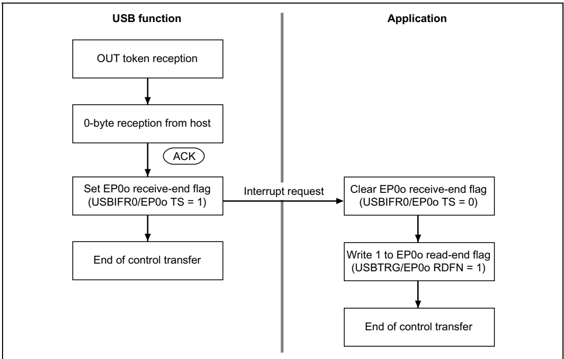
Figure 23.8 Status Stage Operation (Control-In)
