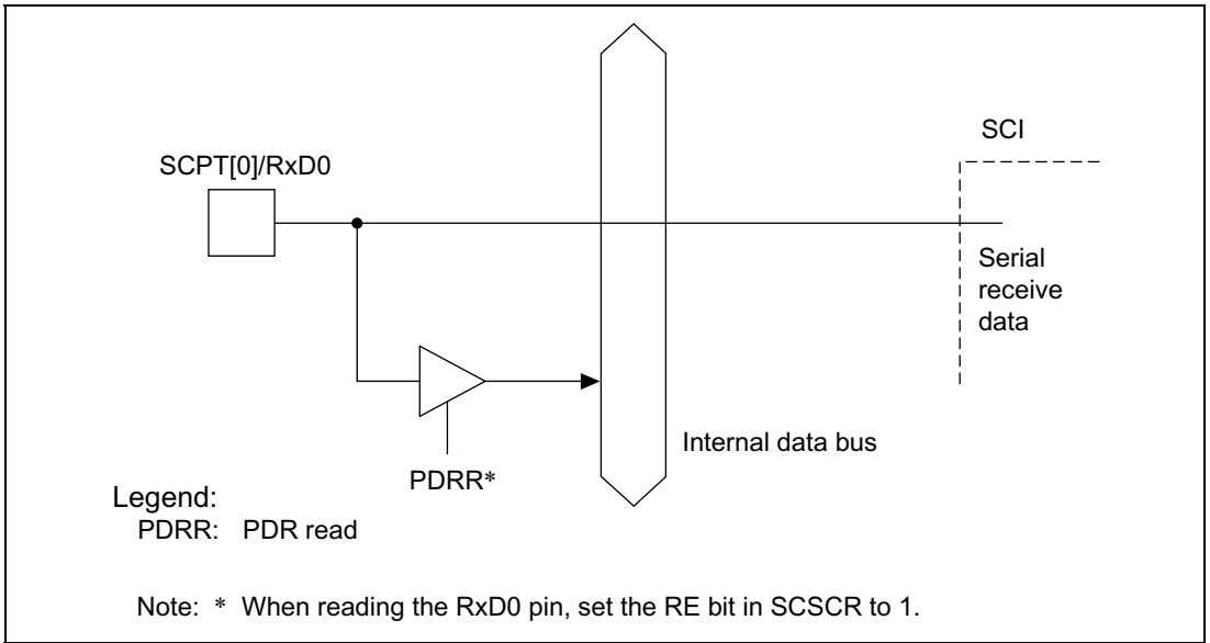
Figure 17.4 SCPT[0]/RxD0 Pin
