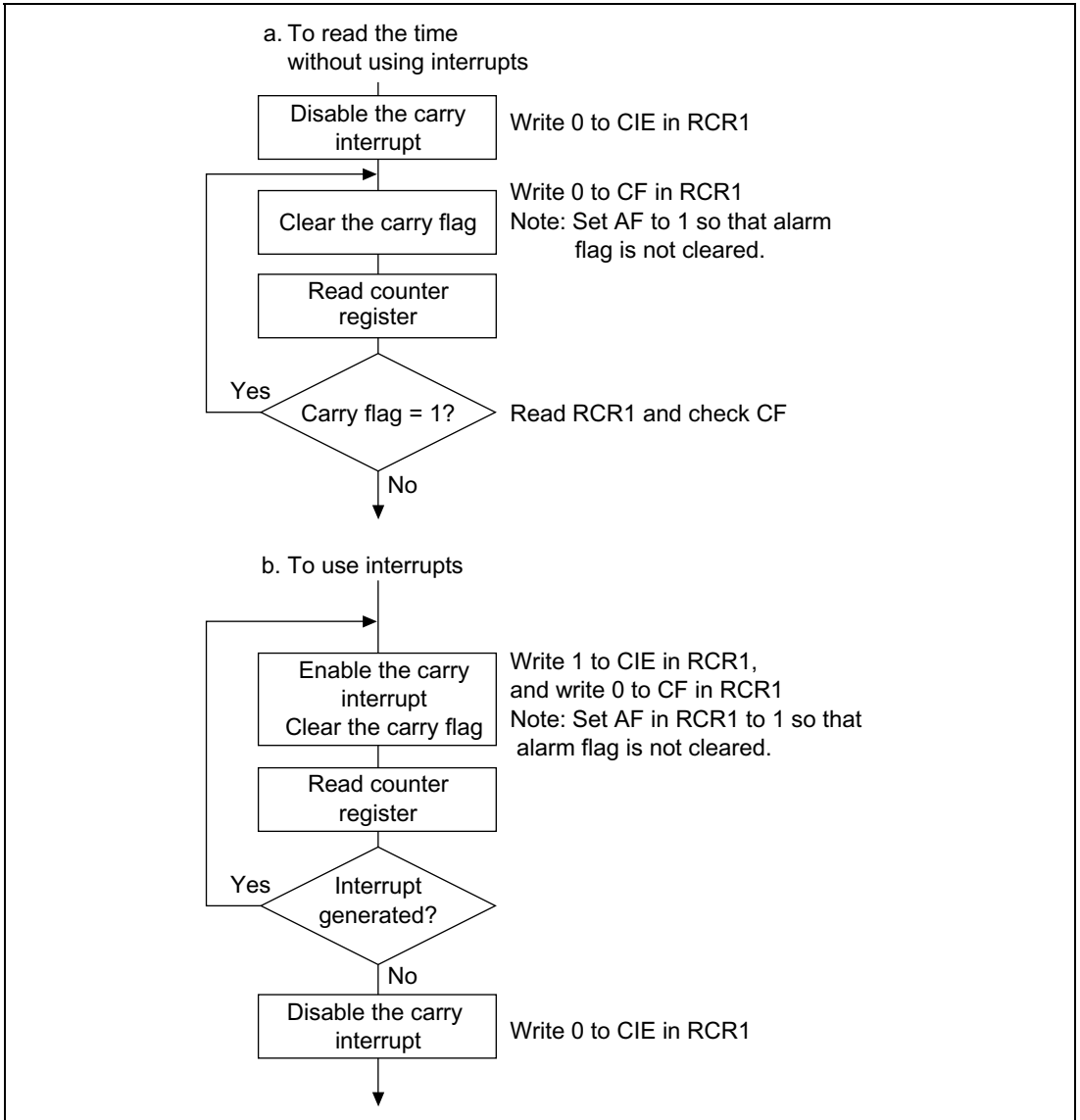
Figure 16.3 Reading the Time
