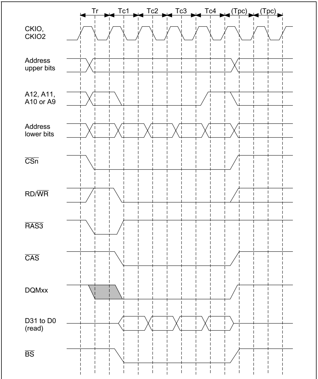
Figure 12.16 Basic Timing for Synchronous DRAM Burst Write
