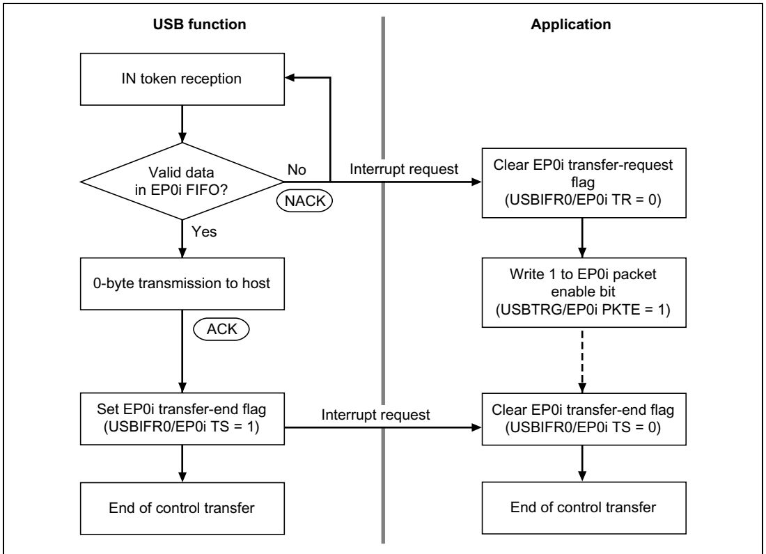
Figure 23.9 Status Stage Operation (Control-Out)
