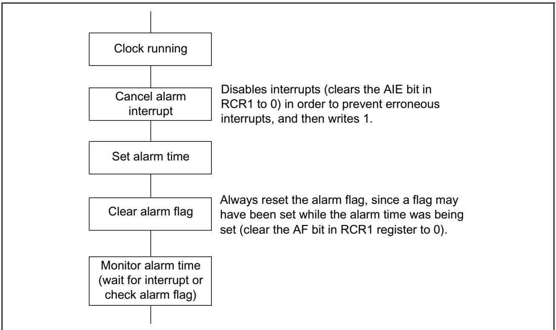
Figure 16.4 Using the Alarm Function
