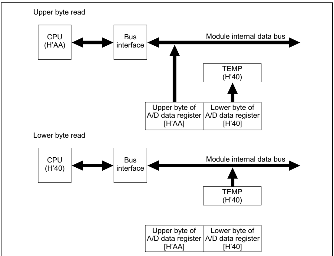
Figure 28.2 A/D Data Register Access Operation (Reading H'AA40)
