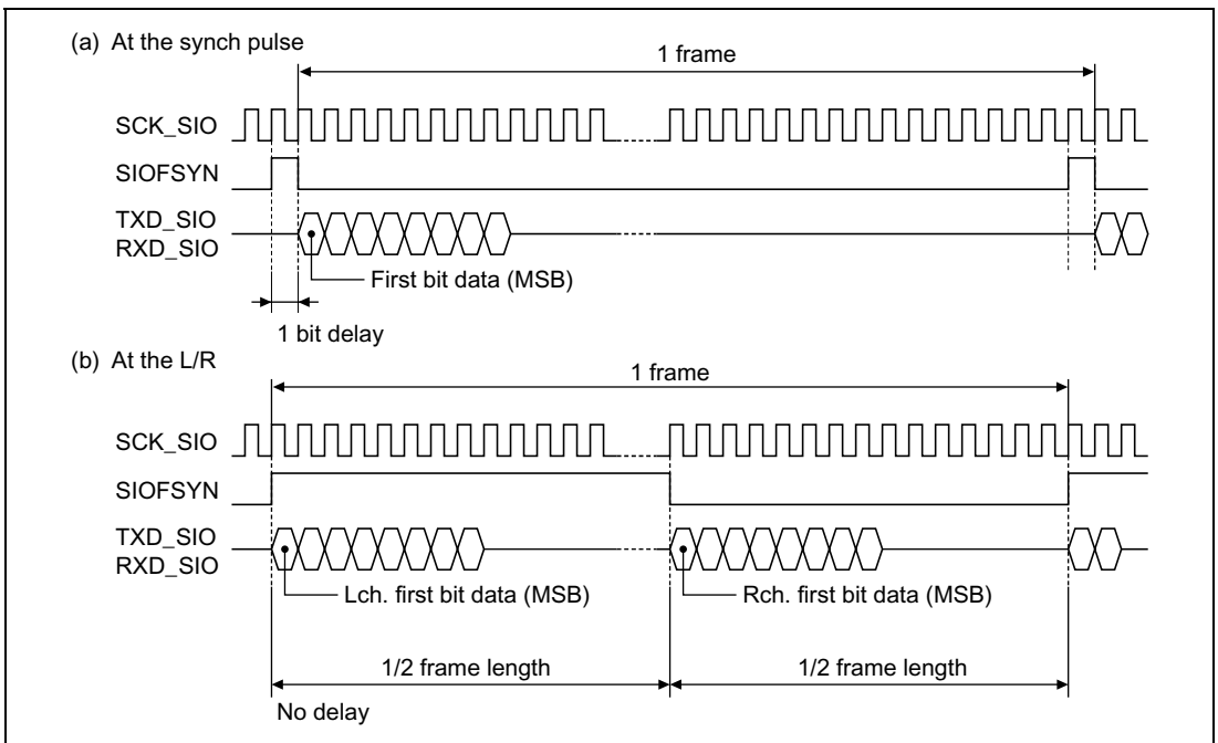
Figure 20.3 SIOF Serial Data Synchronized Timing
