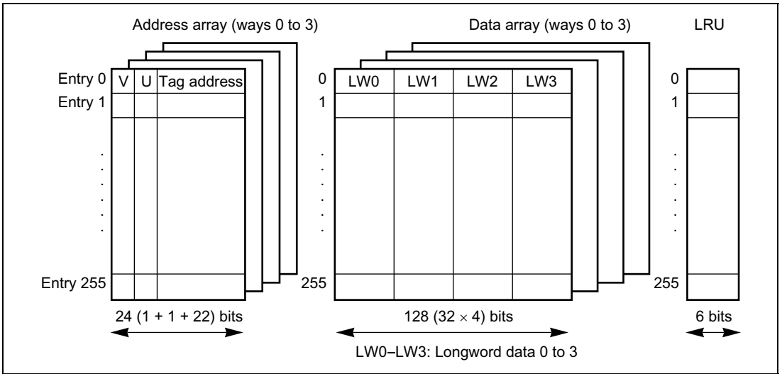
Figure 5.1 Cache Structure
