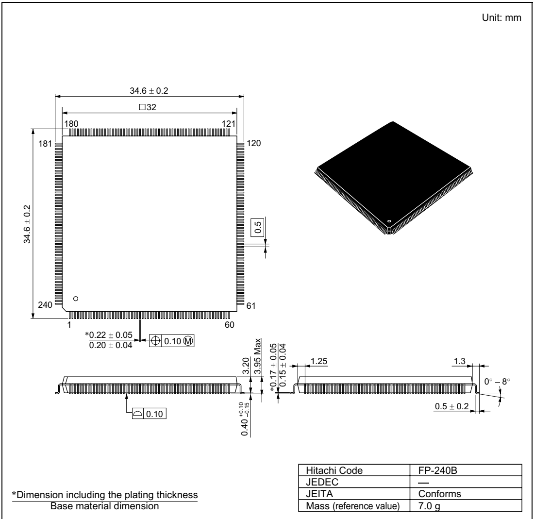
Figure D.1 Package Dimensions (FP-240B)
