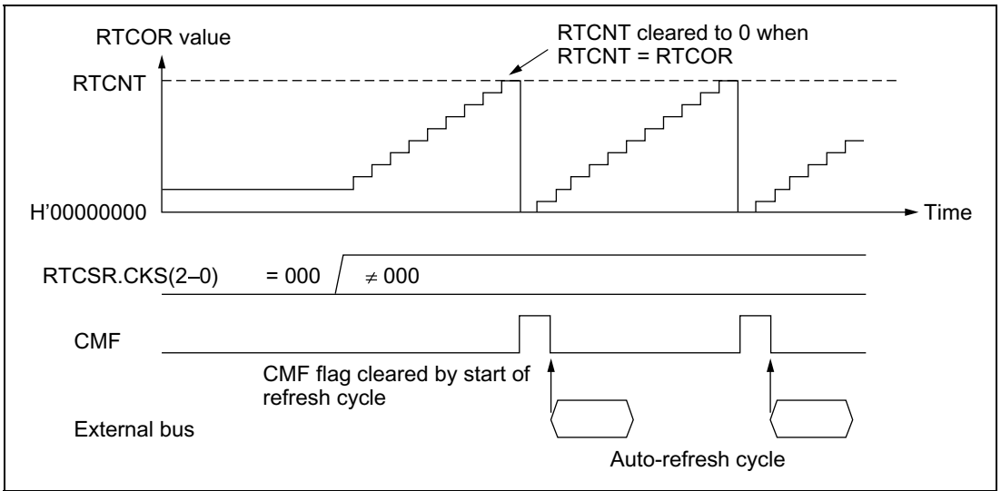
Figure 12.18 Auto-Refresh Operation
