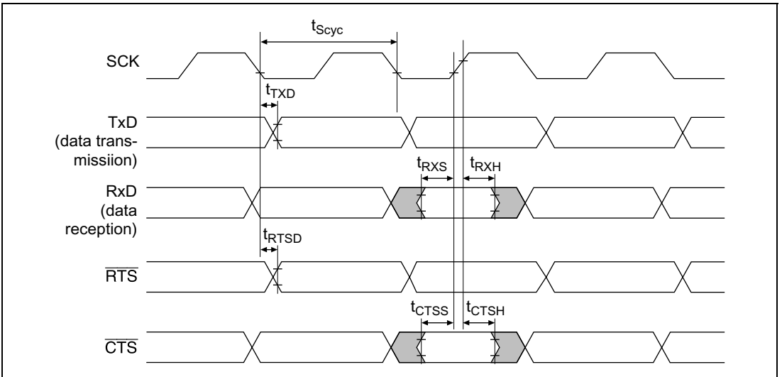
Figure 32.41 SCI I/O Timing in Clock Synchronous Mode
