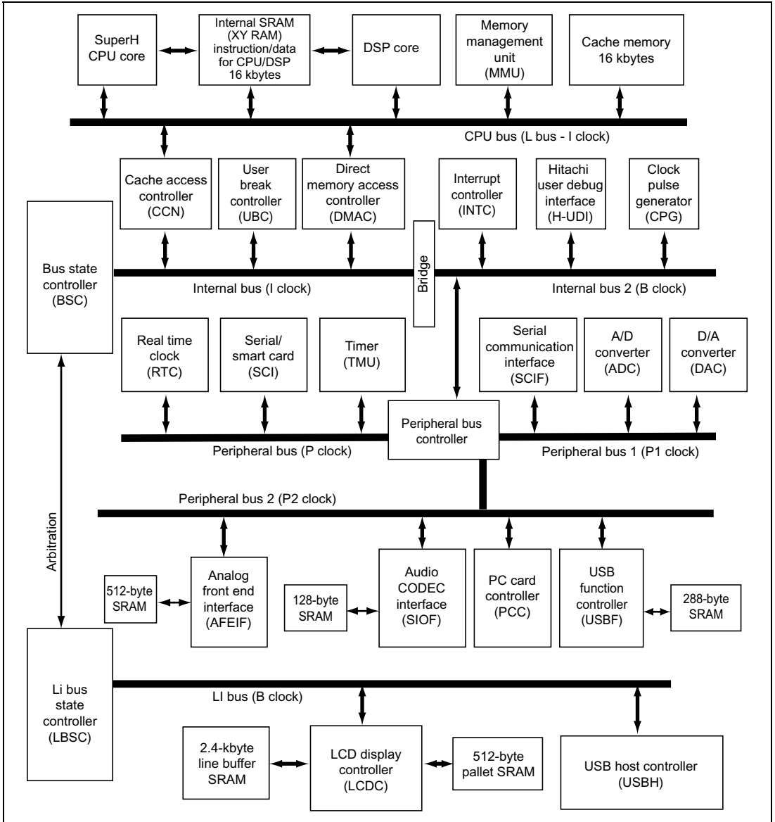
Figure 1.1 Block Diagram
