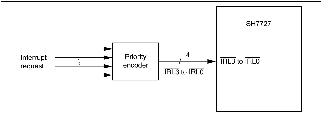
Figure 7.2 Example of IRL Interrupt Connection
