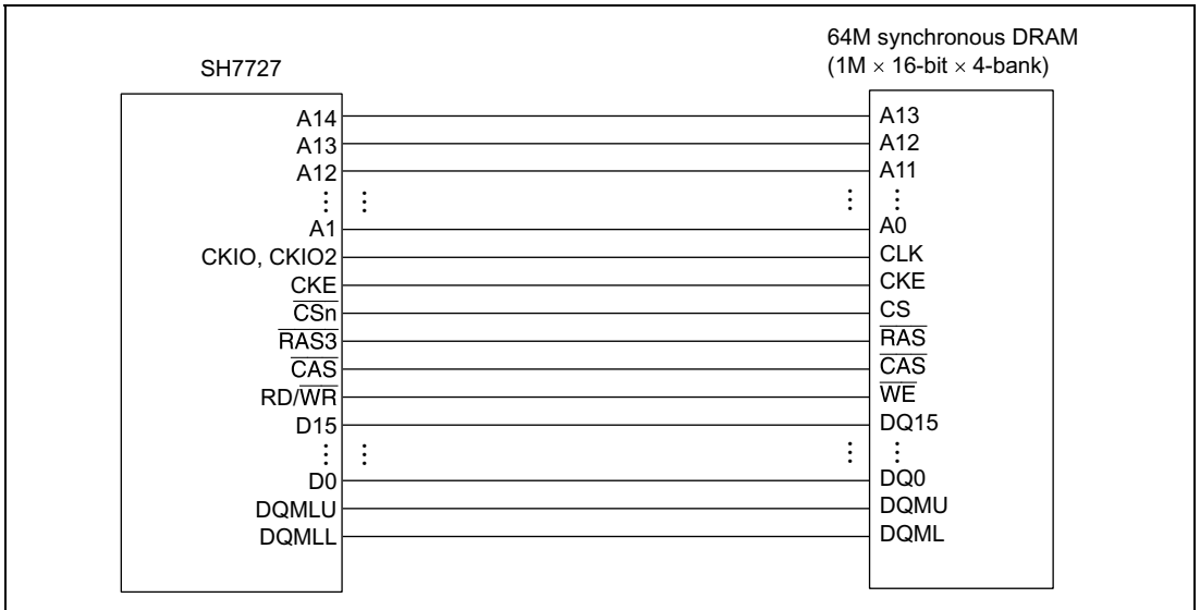
Figure 12.12 Example of 64-Mbit Synchronous DRAM (16-Bit Bus Width)
