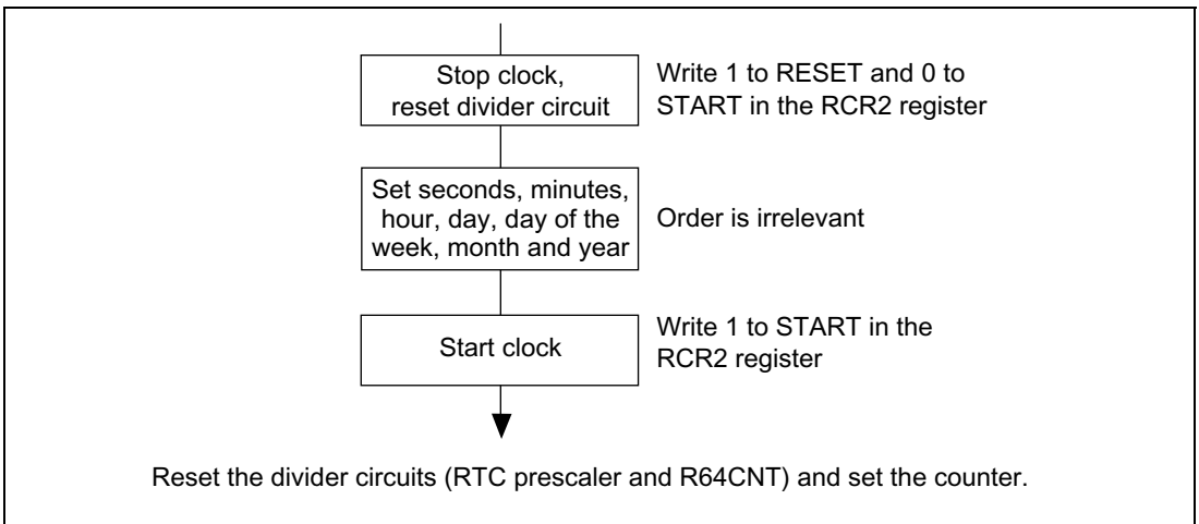
Figure 16.2 Setting the Time
