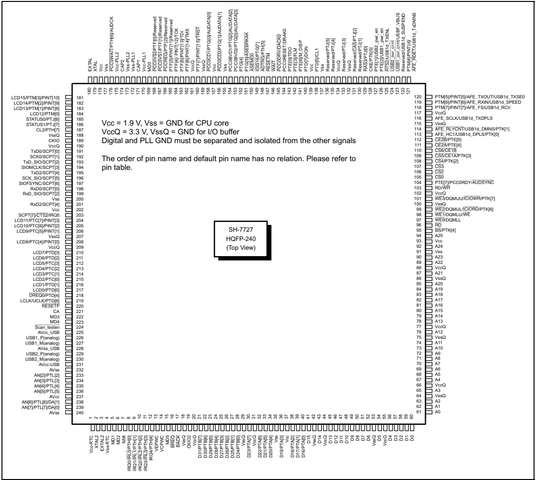
Figure 1.2 Pin Arrangement (FP-240B)
