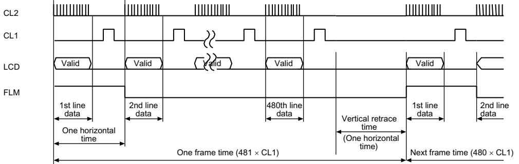
Figure 25.21 Clock and LCD Data Signal Example
