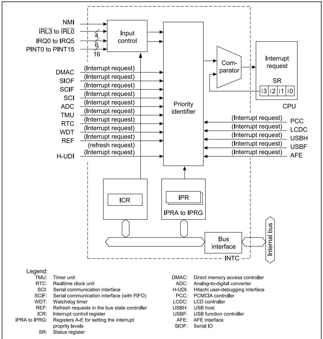
Figure 7.1 INTC Block Diagram
