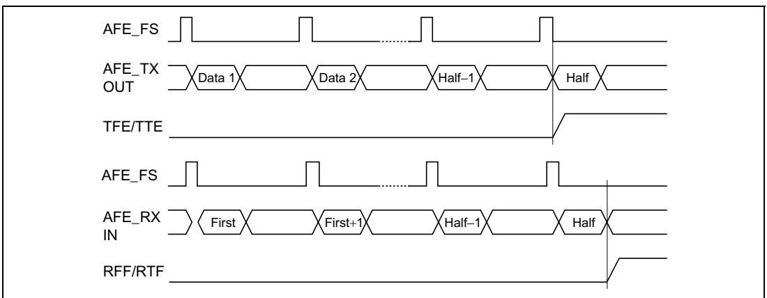
Figure 21.2 FIFO Interrupt Timing
