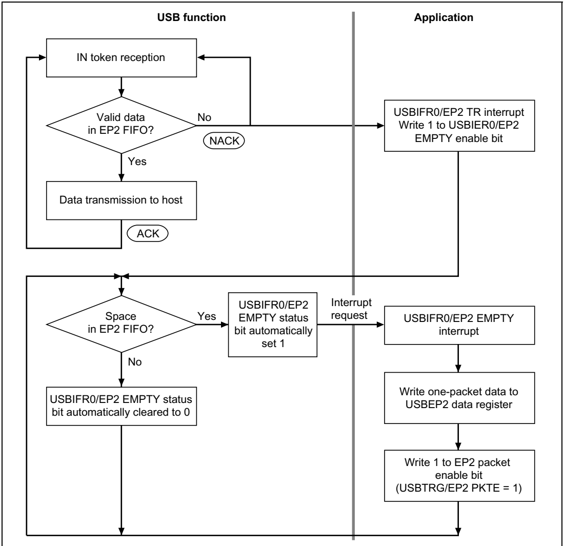
Figure 23.11 EP2 Bulk-In Transfer Operation
