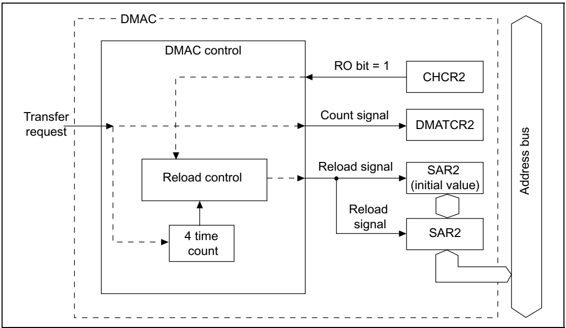
Figure 14.24 Source Address Reload Function Diagram
