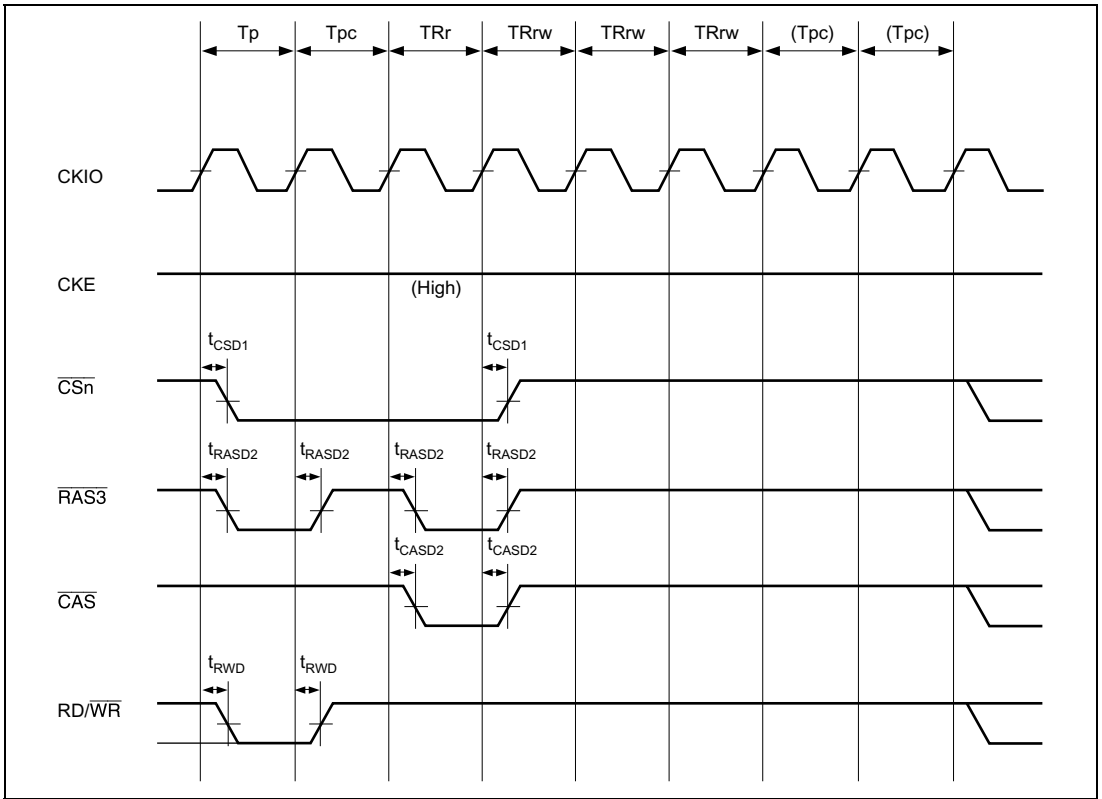
Figure 32.29 Synchronous DRAM Auto-Refresh Cycle (TRAS = 1, TPC = 1)
