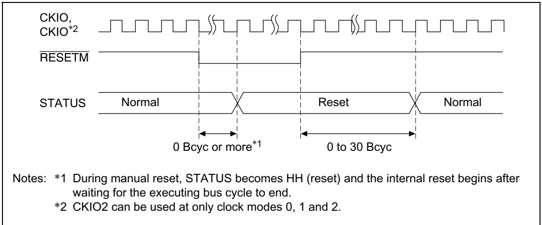
Figure 9.3 Manual Reset STATUS Output
