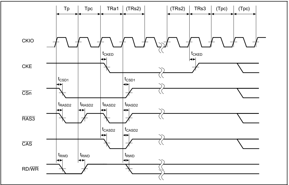
Figure 32.30 Synchronous DRAM Self-Refresh Cycle (TPC = 0)
