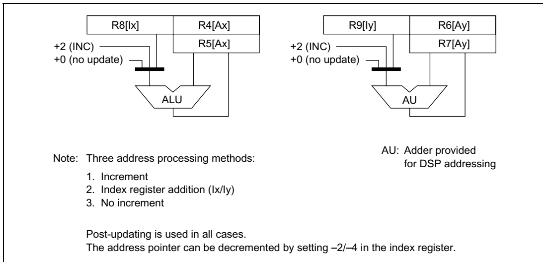
Figure 2.12 X and Y Data Transfer Addressing
