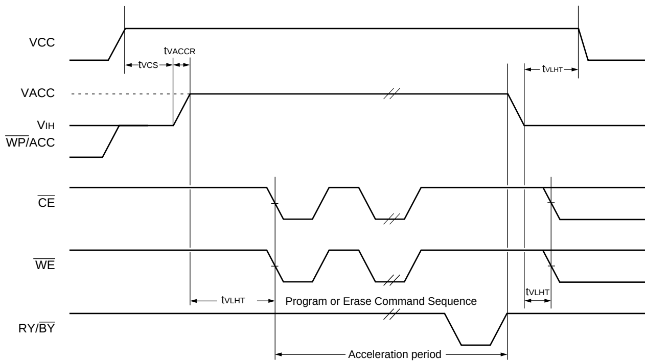
Figure 21 Accelerated Program Timing Diagram
