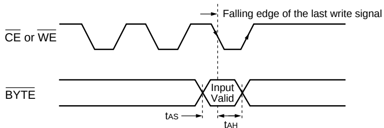
Figure 17 \overline{BYTE} Timing Diagram for Write Operations
