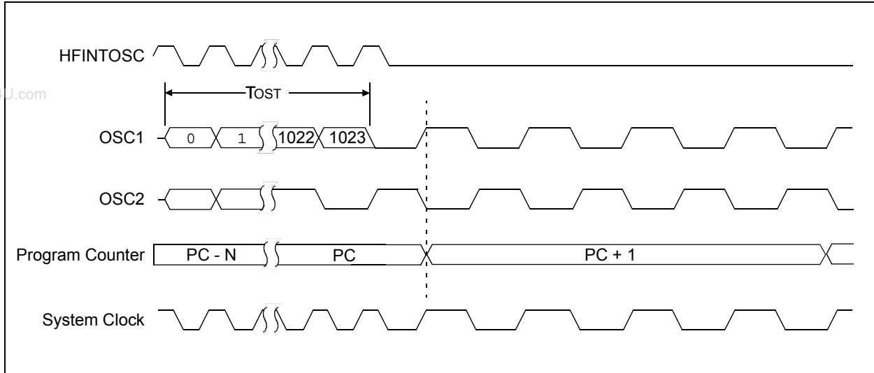
FIGURE 4-7: TWO-SPEED START-UP
