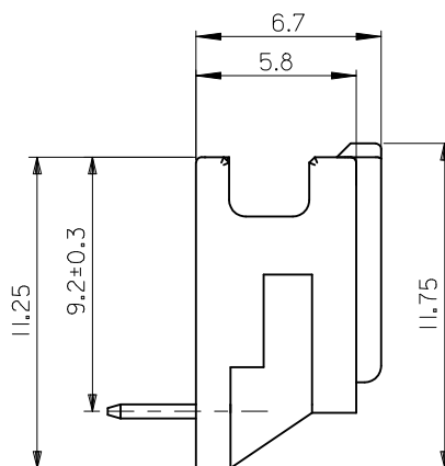
SECT. X-X
