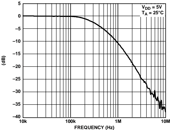
Figure 47. Multiplying Bandwidth
