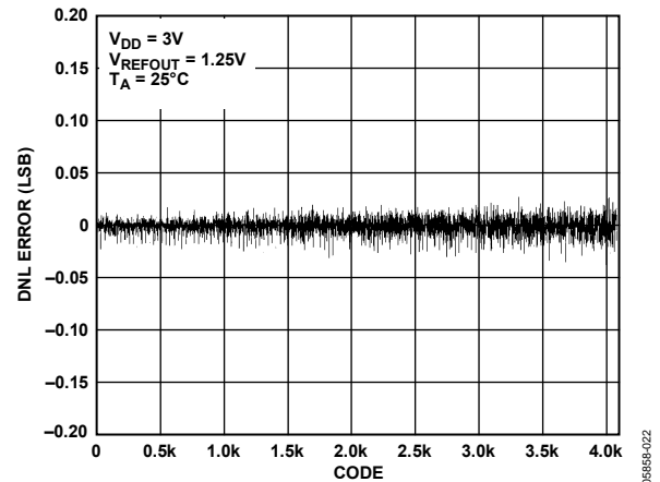
Figure 21. DNL—AD5623R-3
