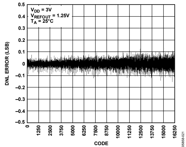
Figure 20. DNL—AD5643R-3
