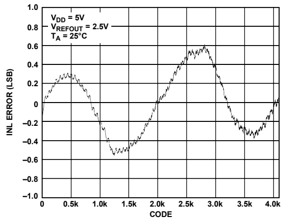
Figure 12. INL—AD5623R-5
