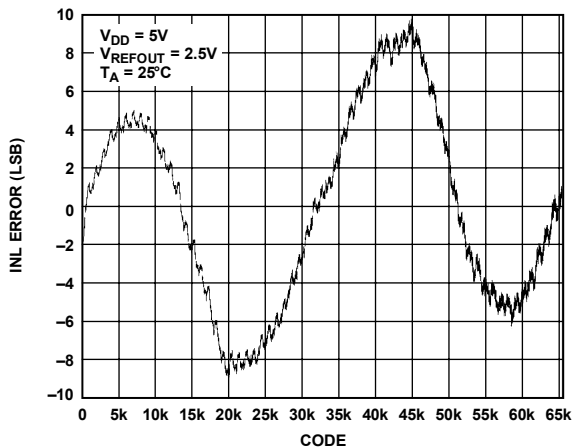
Figure 10. INL—AD5663R-5
