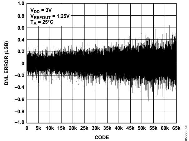
Figure 19. DNL—AD5663R-3
