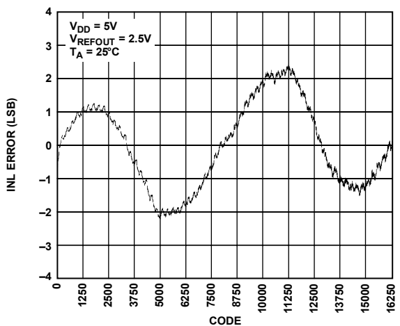
Figure 11. INL—AD5643R-5
