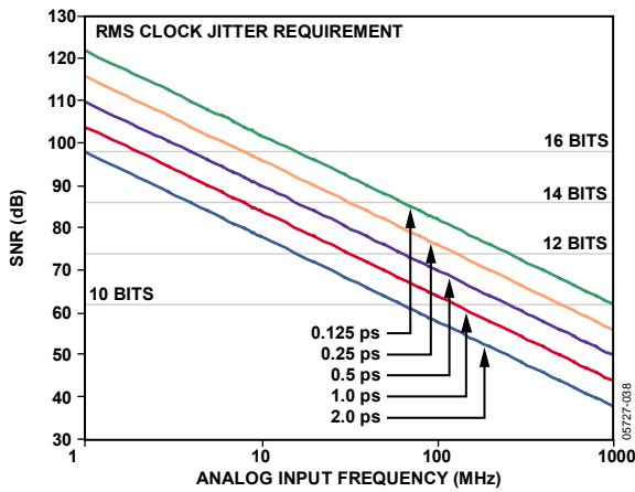
Figure 55. Ideal SNR vs. Input Frequency and Jitter
