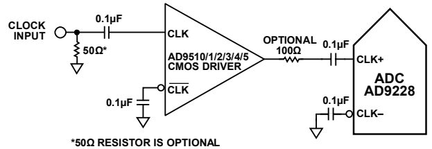
Figure 54. Single-Ended 3.3 V CMOS Sample Clock
