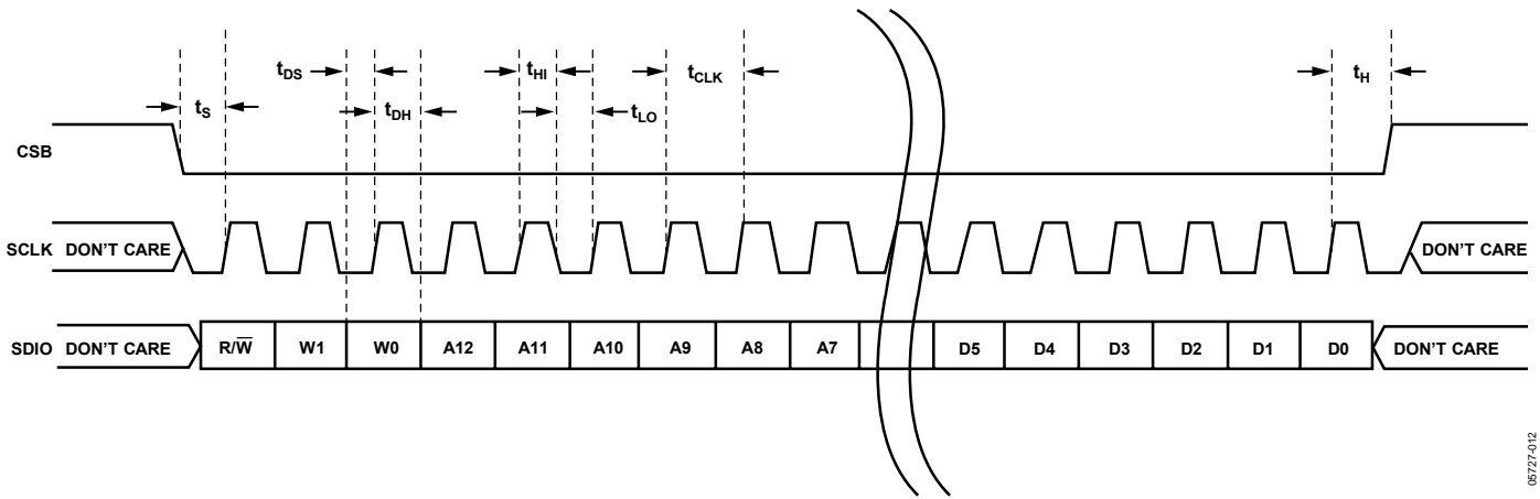
Figure 68. Serial Timing Details
