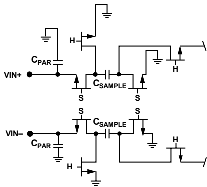
Figure 43. Switched-Capacitor Input Circuit
