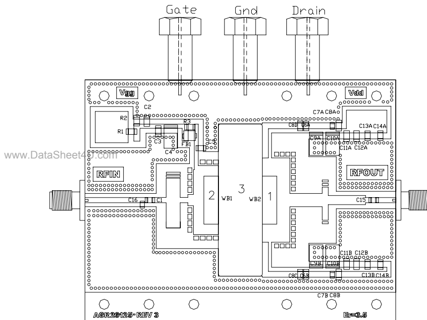
Figure 2. AGR26125E Component Layout
