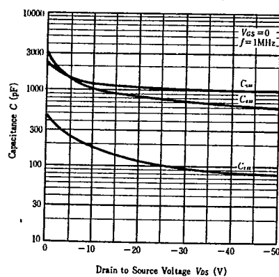
TYPICAL CAPACITANCE VS. DRAIN-SOURCE VOLTAGE
