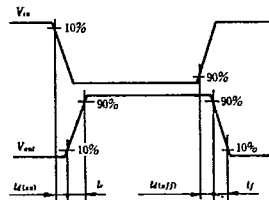
WAVEFORMS
