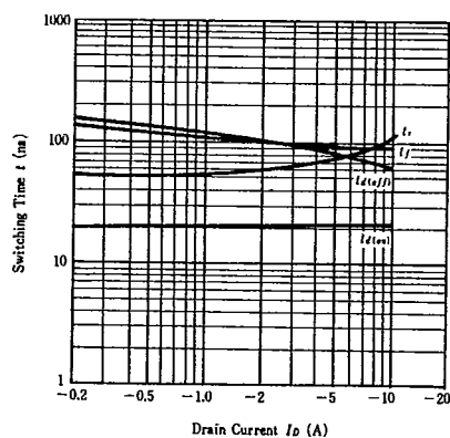
SWITCHING CHARACTERISTICS
