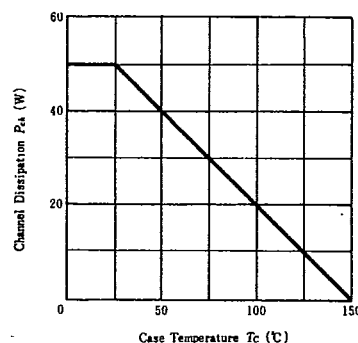
POWER VS. TEMPERATURE DERATING
