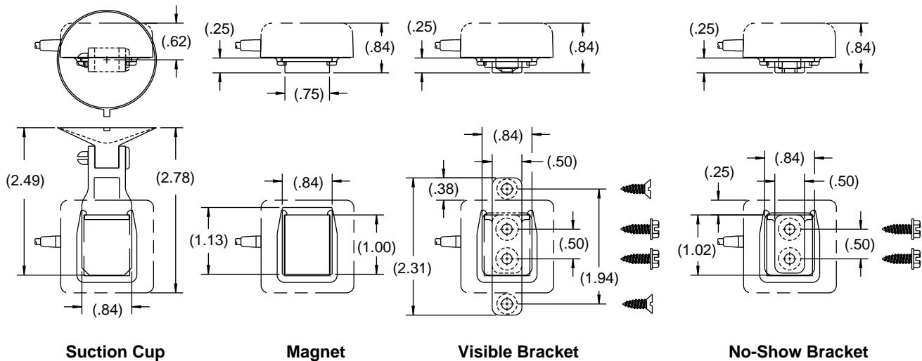
Mounting Options for QuickMount Micro GPS Patch Antennas
