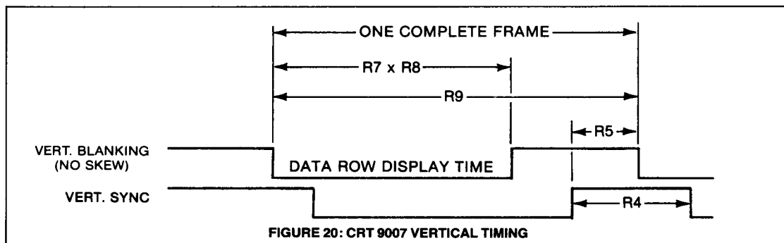
FIGURE 20: CRT 9007 VERTICAL TIMING
