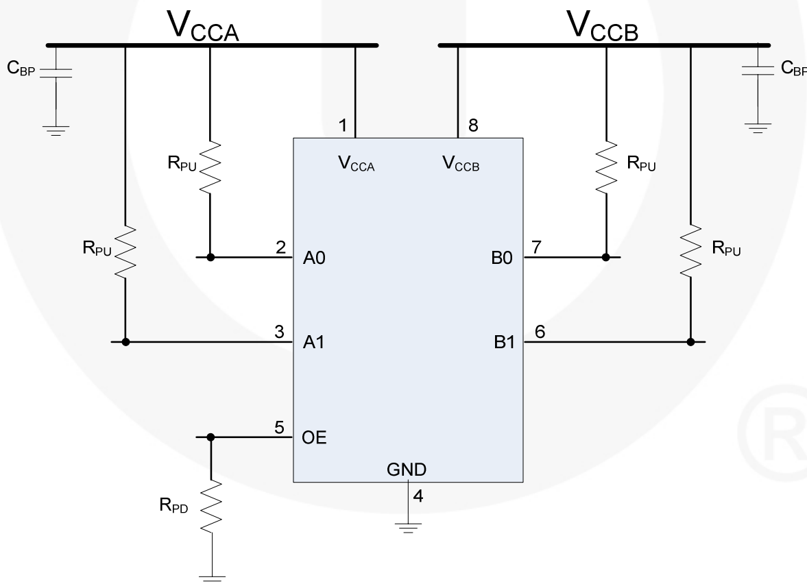
Figure 4. Application Circuit
