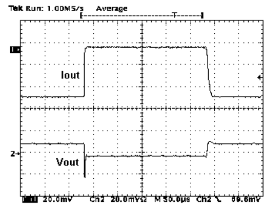
Figure 28 : Load Transient
