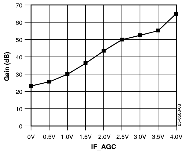
Figure 1. Typical IF_AGC Control Characteristics
