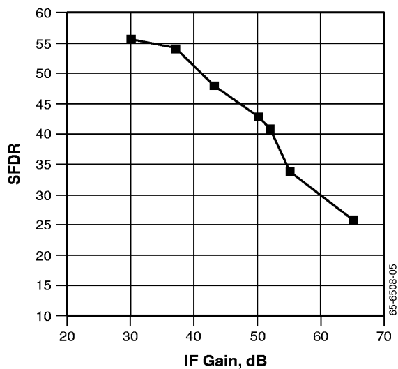
Figure 3. SFDR vs. RC6508/TMC1175AM7C40 (Raytheon Demo Board with 64 QAM demodulator)
