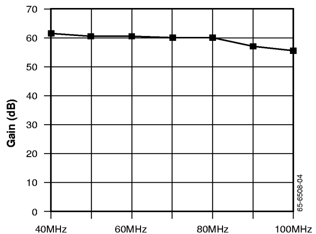
Figure 2. IF Input Bandwidth
