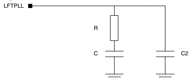
Figure 4. RC Filter Connection to PLL Input of Device
