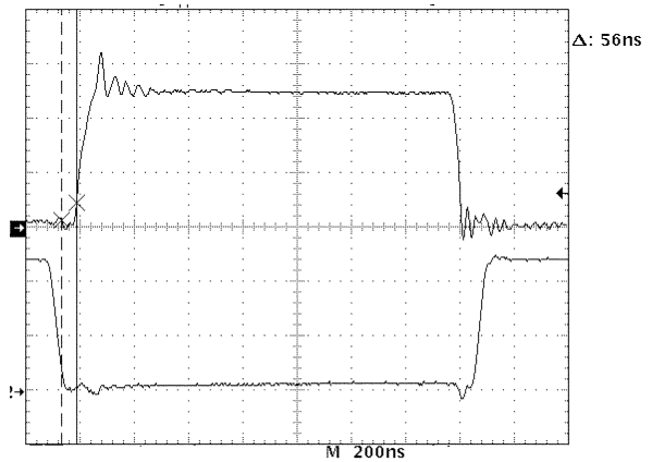
Trace 1 = GATE(H) (5.0 V/div.) Trace 2 = GATE(L) (5.0 V/div.)
