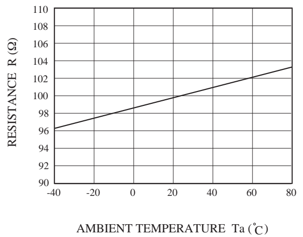
R_{Line} - TEMPERATURE
