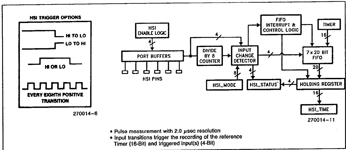
Figure 6. High Speed Input Unit
