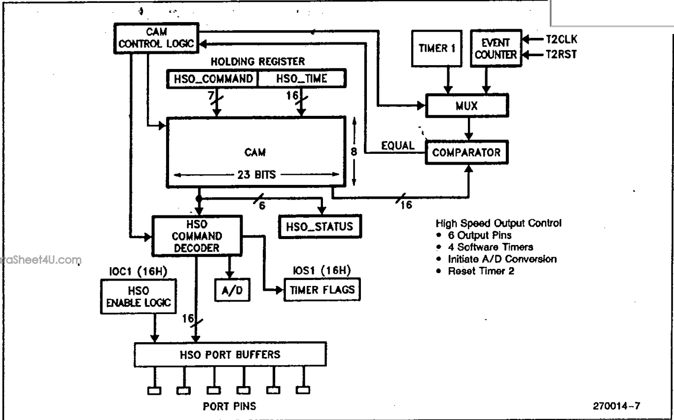
Figure 7. High Speed Output Unit
