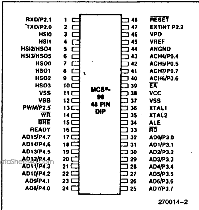
Figure 2. 48-Pin Package
