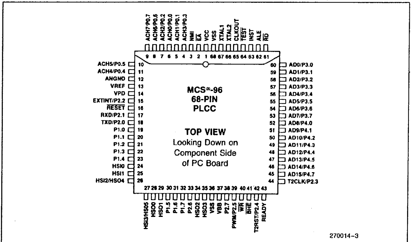
Figure 3. 68-Pin PLCC Package
