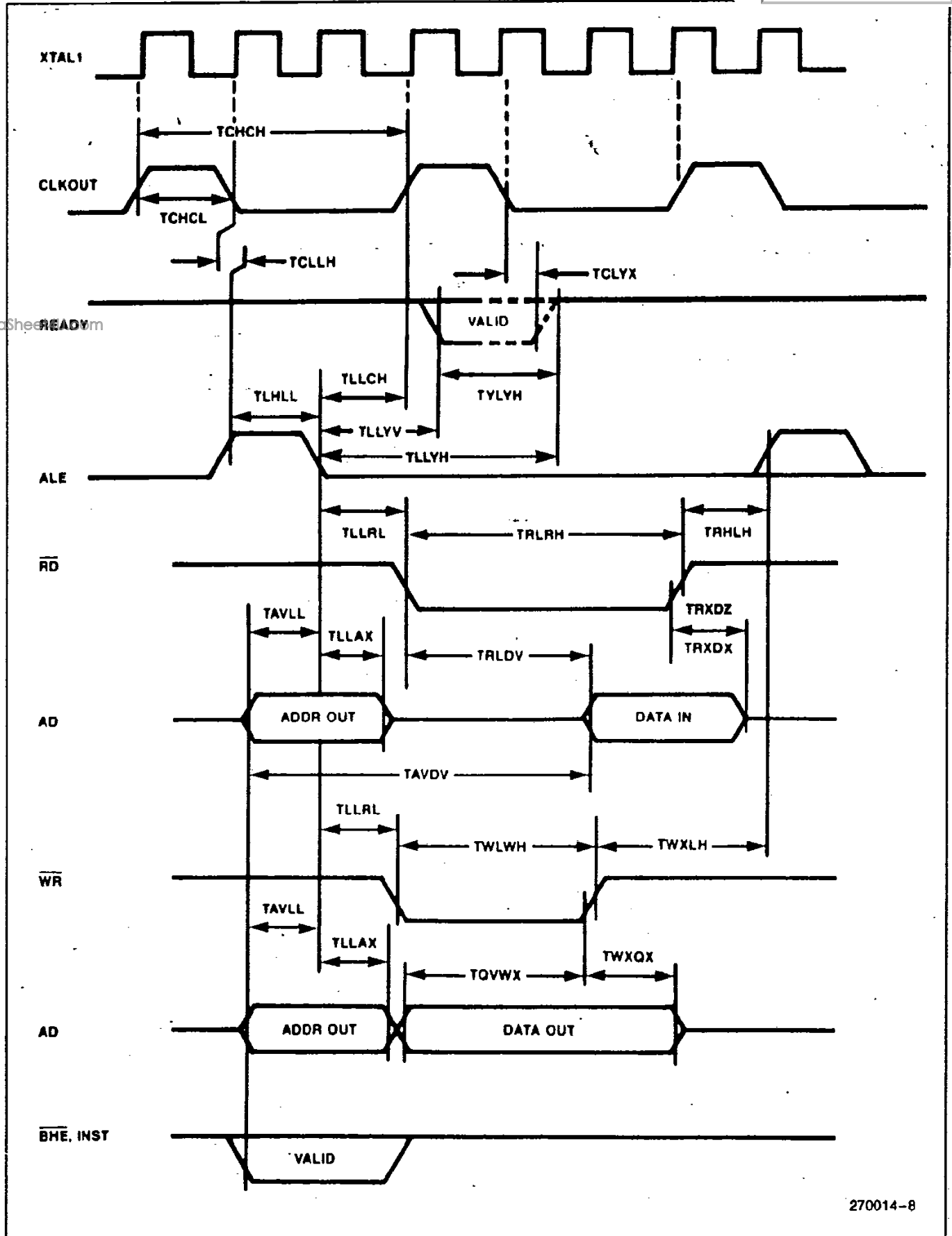
Bus Signal Timings
