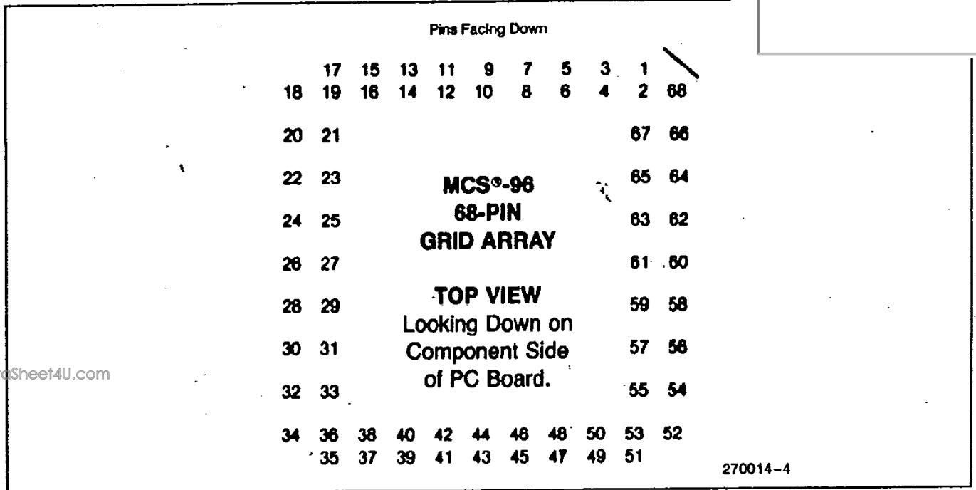
Figure 4. Pin Grid Array
