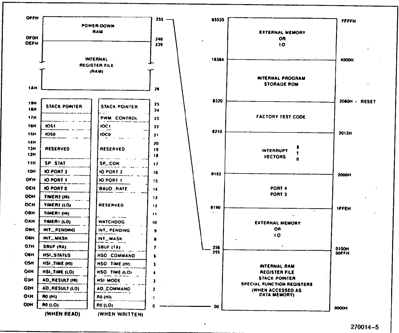
Figure 5. Memory Map
