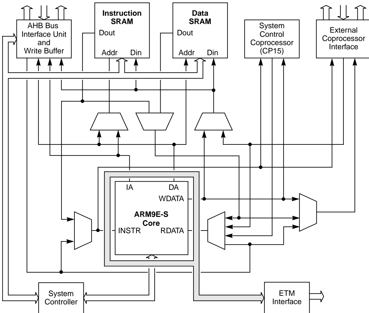
Figure 1 CW001103 Block Diagram
