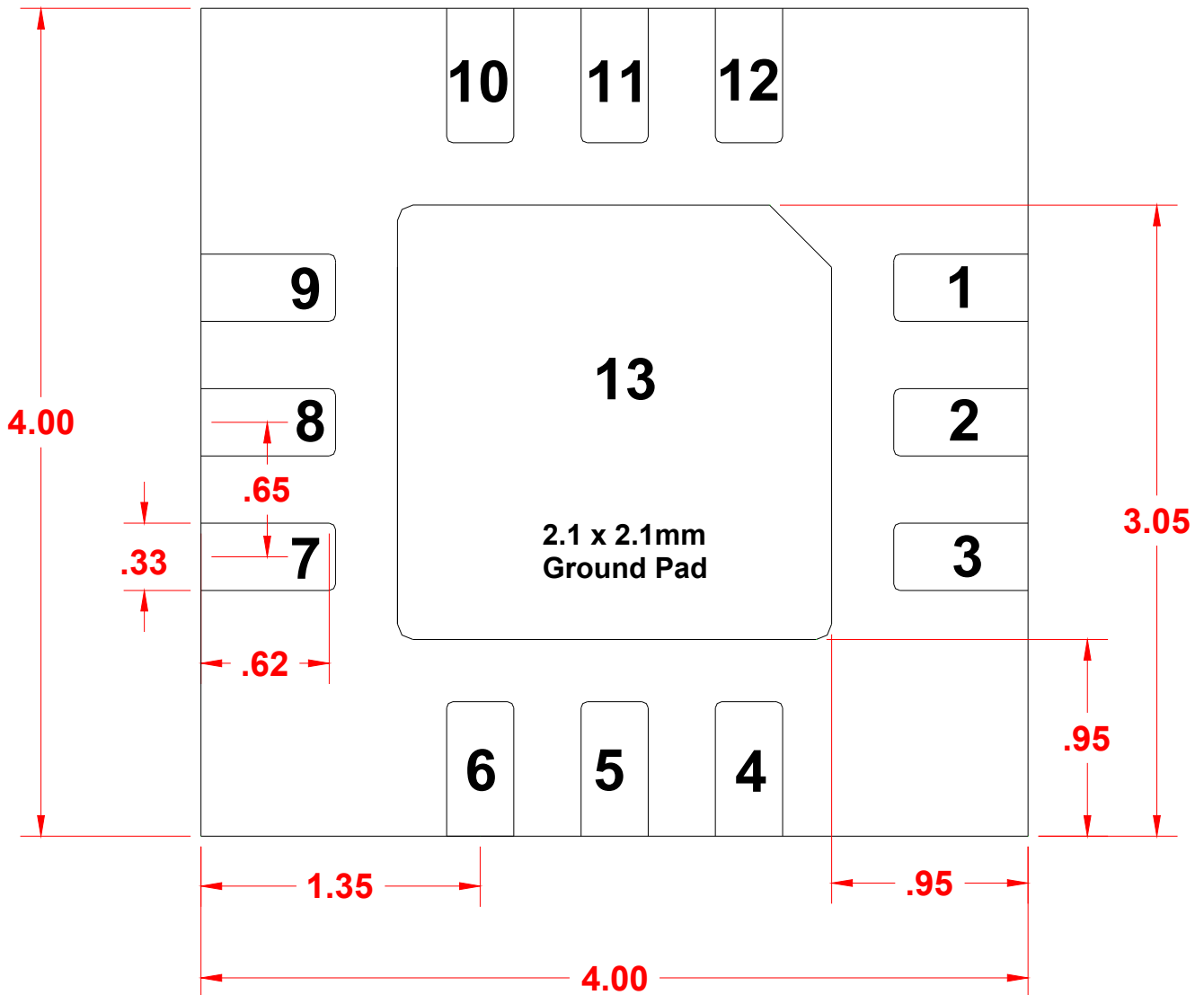
Bottom View
