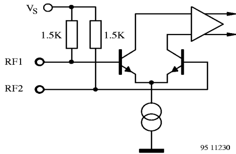
Figure 7. RF input
