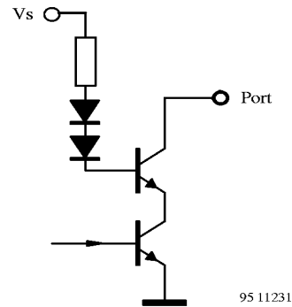
Figure 10. Ports
