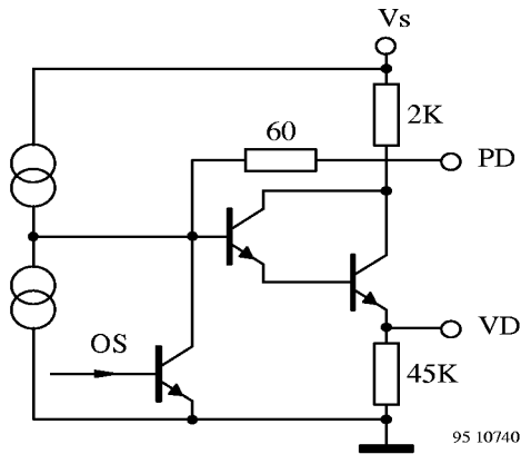
Figure 13. Loop amplifier
