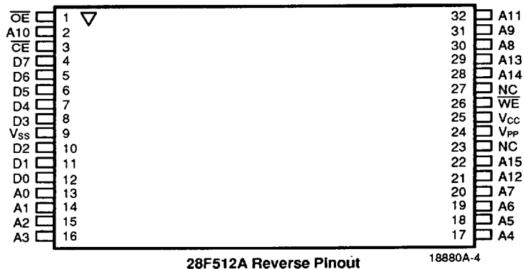
28F512A Reverse Pinout
