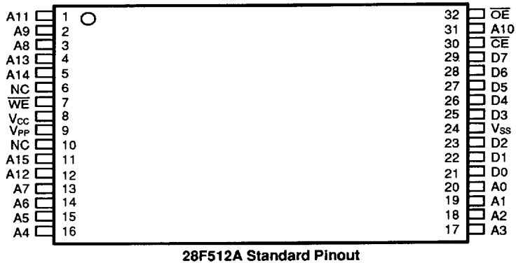
28F512A Standard Pinout
