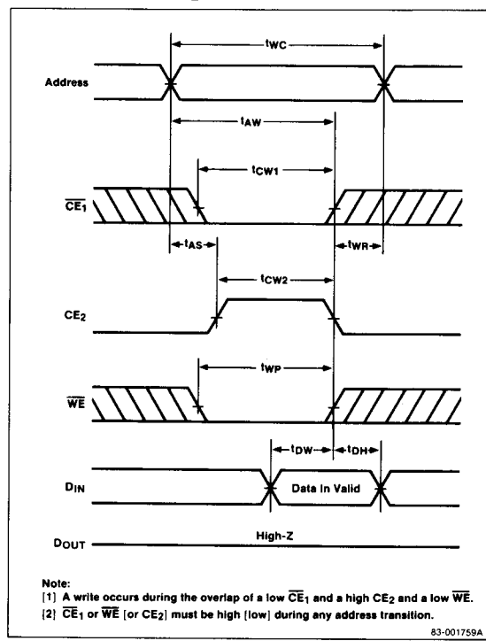
Write Cycle No. 3 ( \overline{CE}_2 Controlled)
