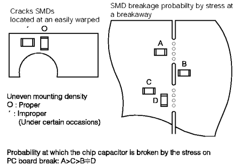
Fig.3 Component Layout
