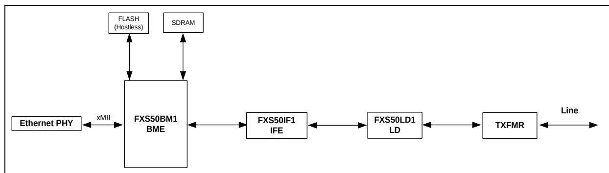
Figure 1–1 Sample Single Port Hostless (VDSL2/VDSL/ADSL2+/ADSL) SLE
