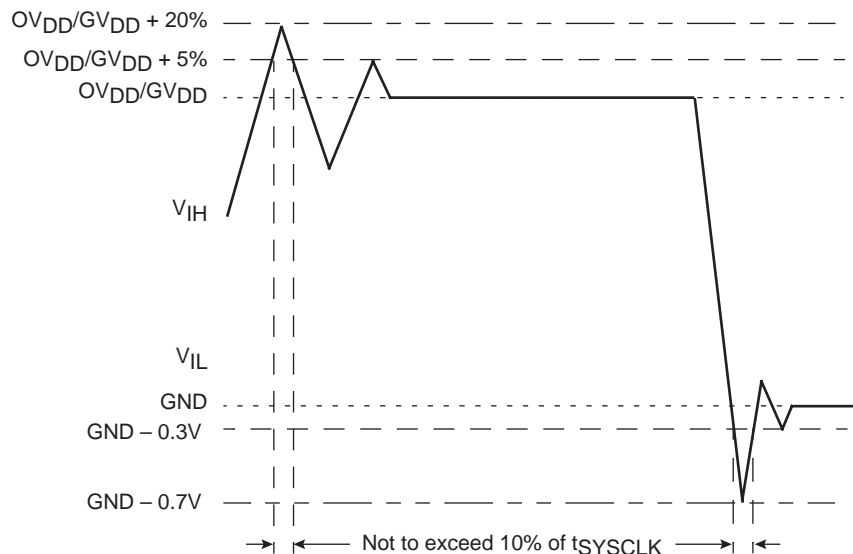
Figure 3. Overshoot/Undershoot Voltage
