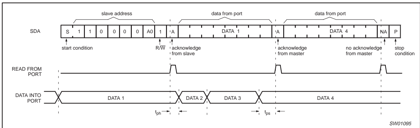
Figure 11. READ input port register
