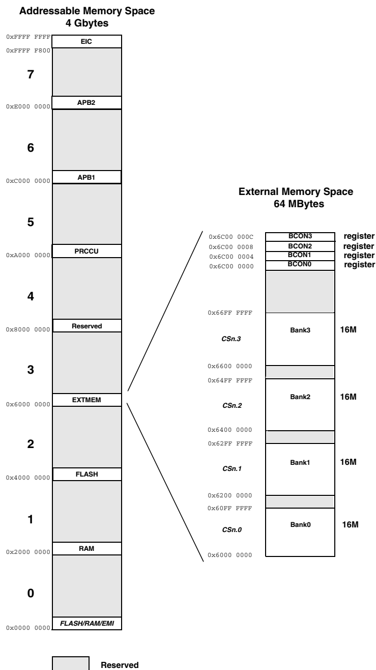
Figure 8. External Memory Map
