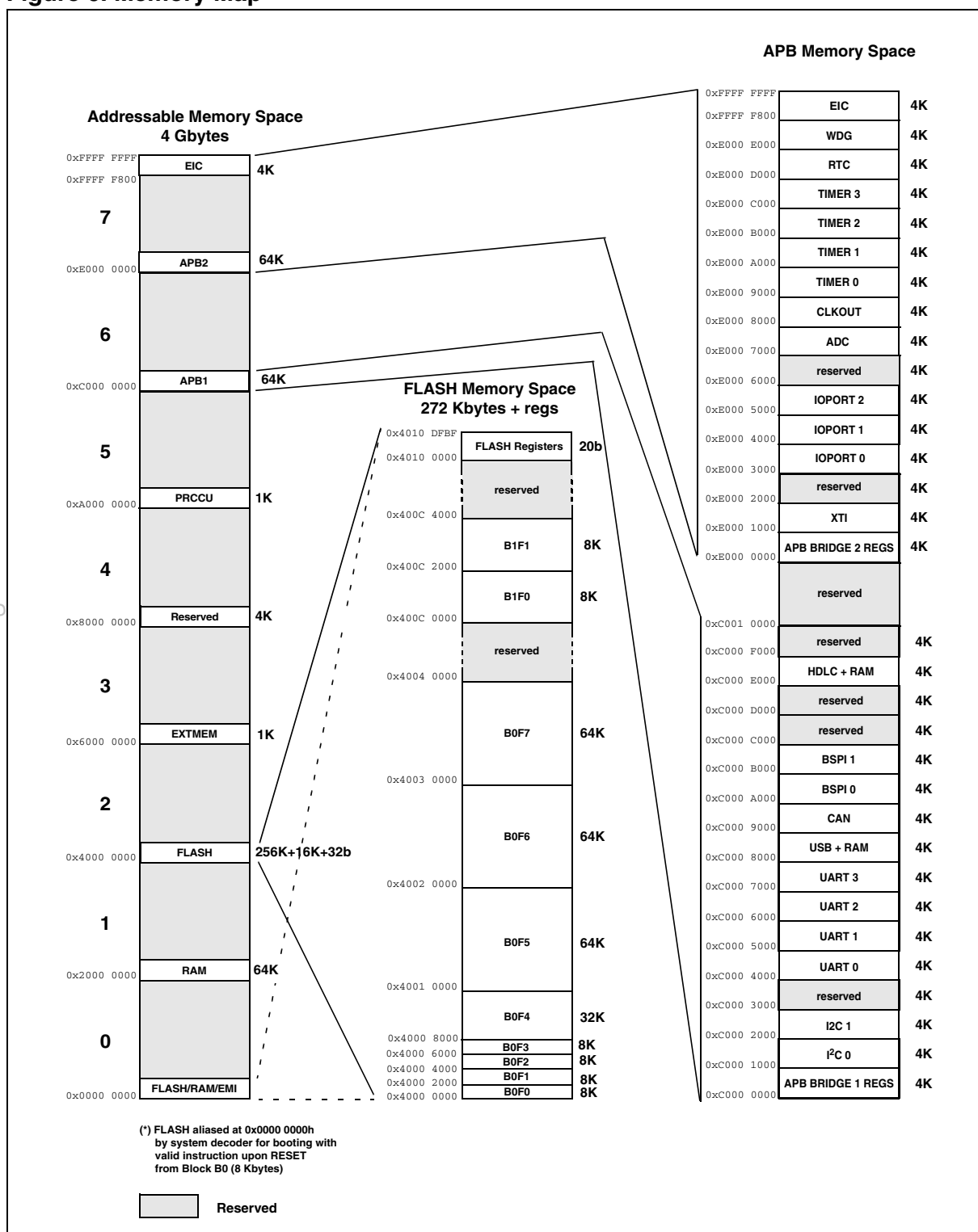
Figure 6. Memory Map
