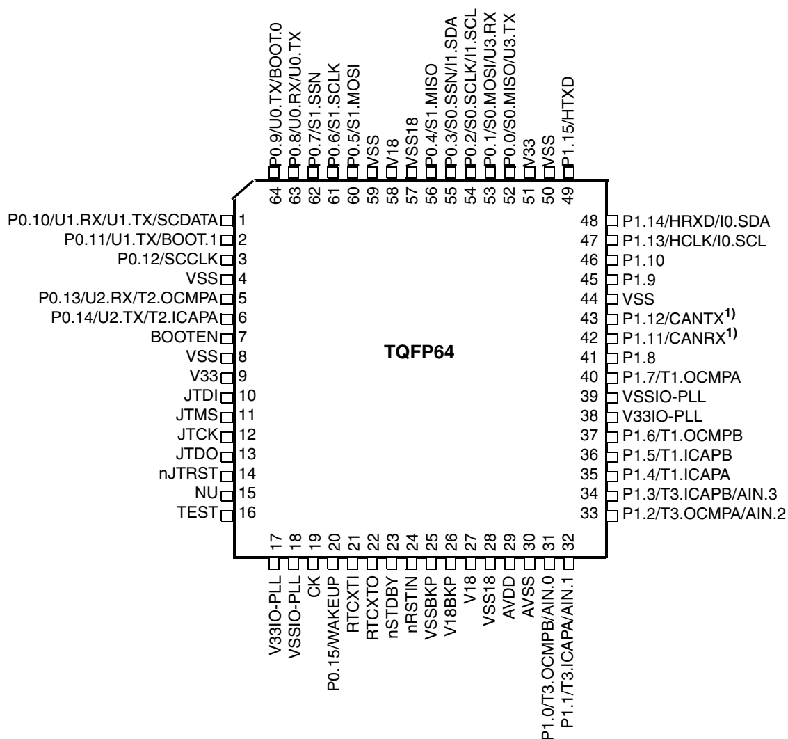
Figure 3. STR712F/STR715F TQFP64 Pinout
