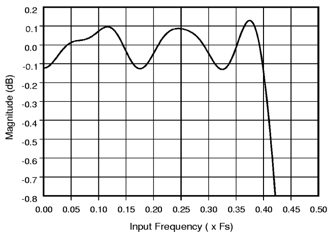
Figure 35. ADC Passband Ripple
