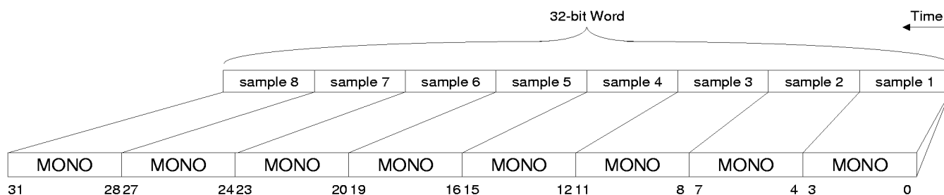
Figure 18. 4-bit Mono, ADPCM Audio Data
