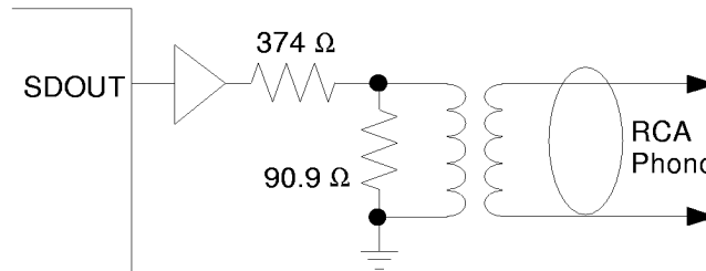
Figure 8. IEC-958 Consumer Interface
