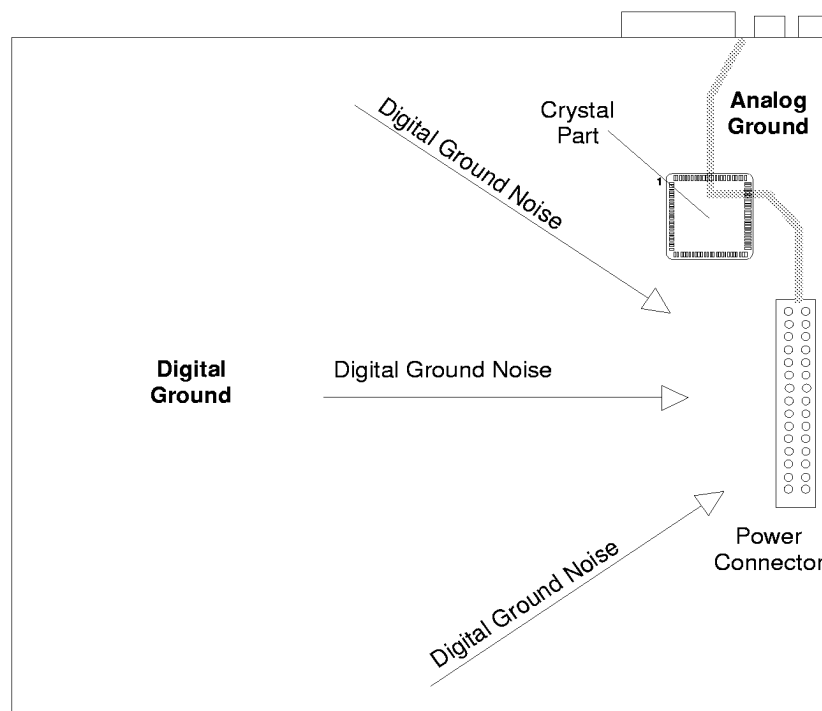
Figure 31. Suggested Motherboard Layout
