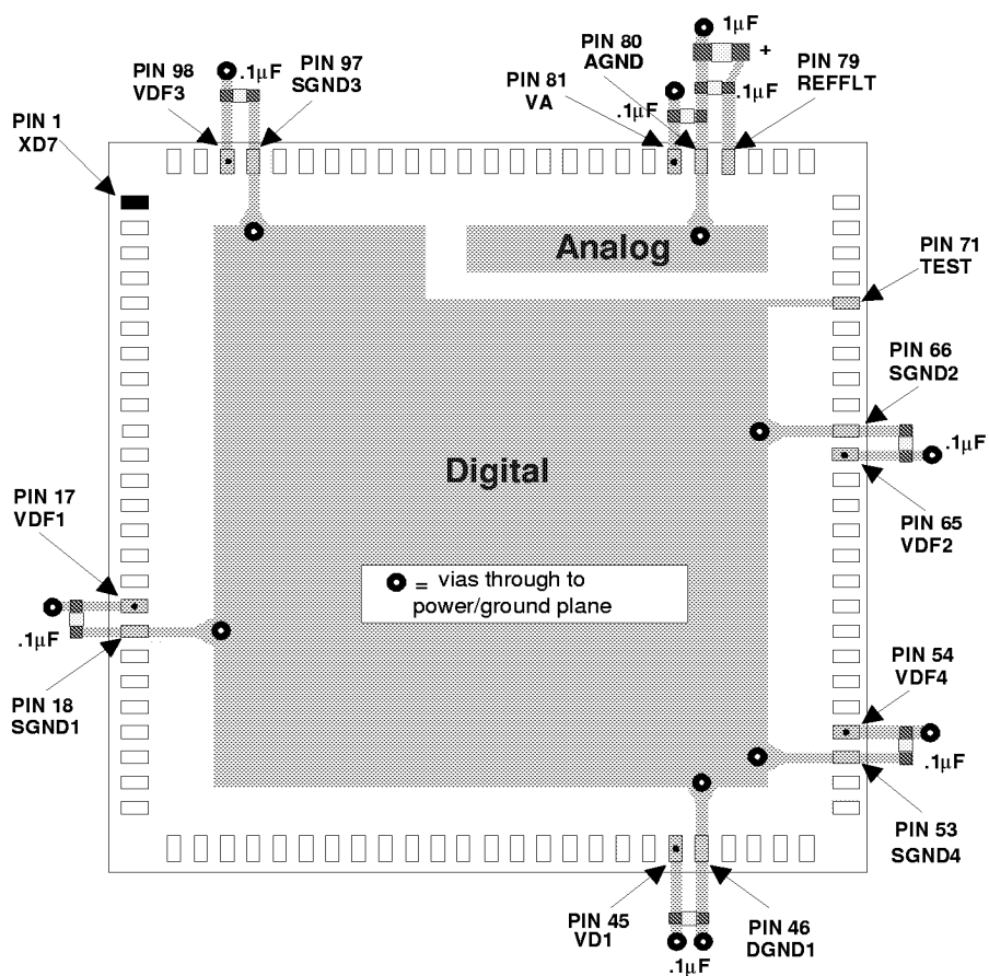
Figure 33. Recommended Decoupling Capacitor Positions
