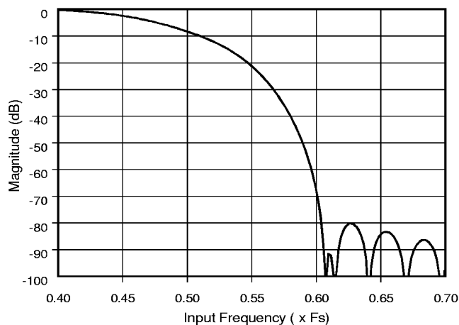
Figure 36. ADC Transition Band
