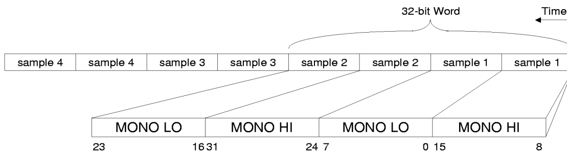
Figure 20. 16-bit Mono, Signed Big Endian Audio Data
