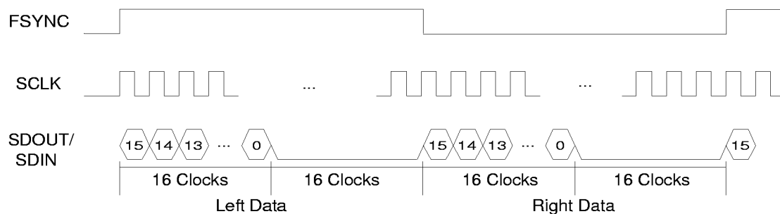
Figure 10. 64-bit Mode (SF1,0 = 01)
