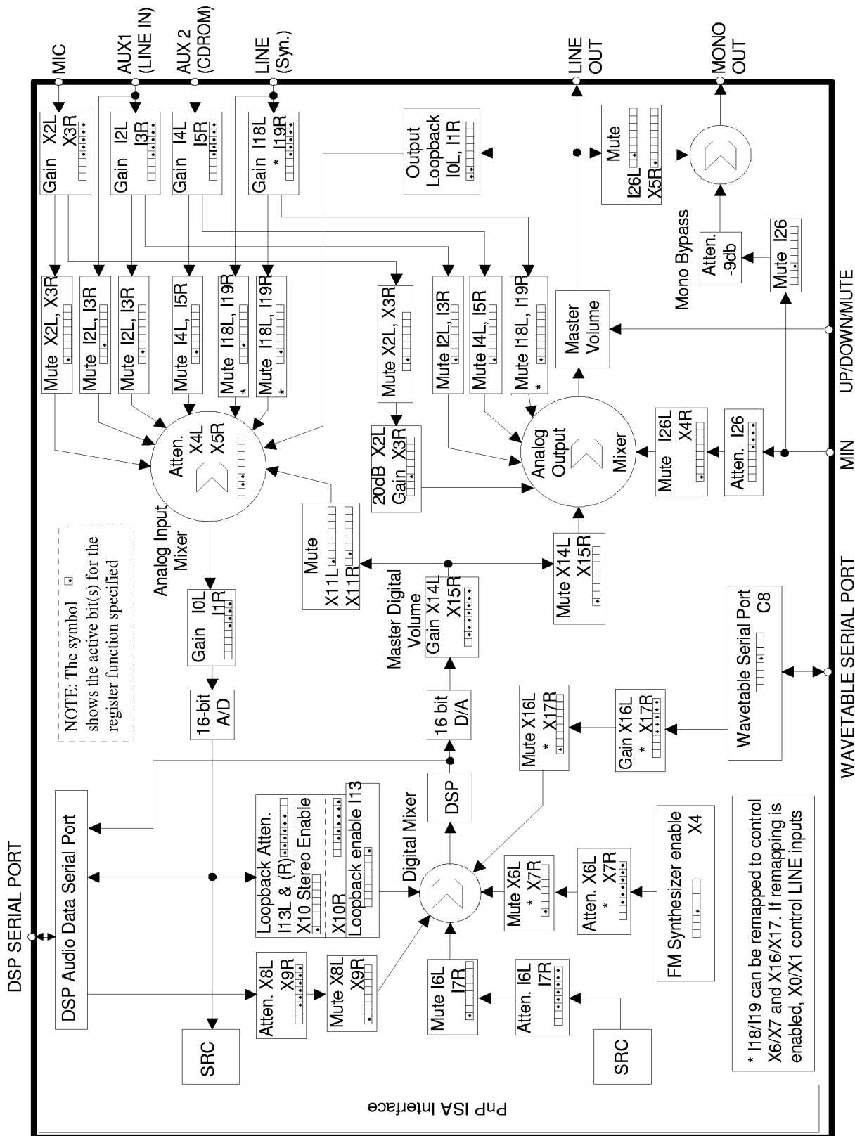
Figure 4. MODE 3 Mixer (assumes IFM or WTEN is set)
