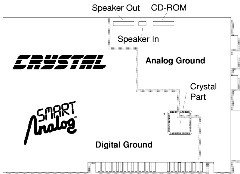
Figure 32. Suggested Add-In Card Layout
