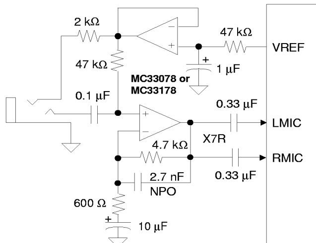
Figure 28. Left or Mono Microphone Input
