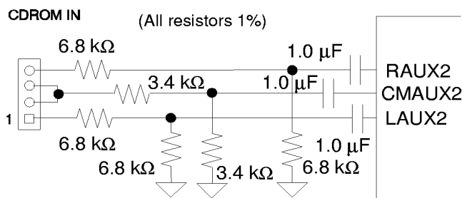
Figure 27. Differential CDRUM In
