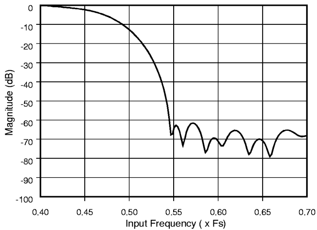
Figure 39. DAC Transition Band
