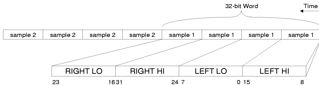
Figure 21. 16-bit Stereo, Signed Big Endian Audio Data
