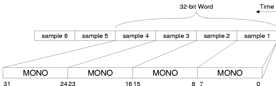
Figure 14. 8-bit Mono, Unsigned Audio Data
