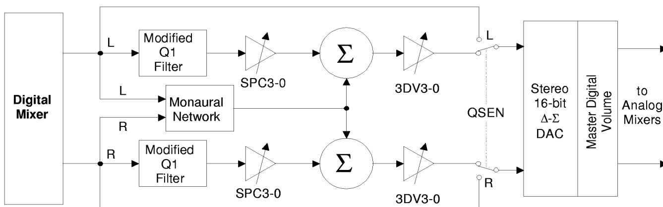
Figure 7. QXpander Block Diagram
