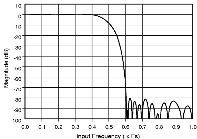
Figure 34. ADC Filter Response
