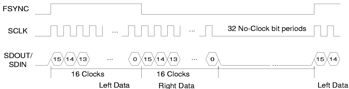
Figure 11. 32-bit Mode (SF1,0 = 10)
